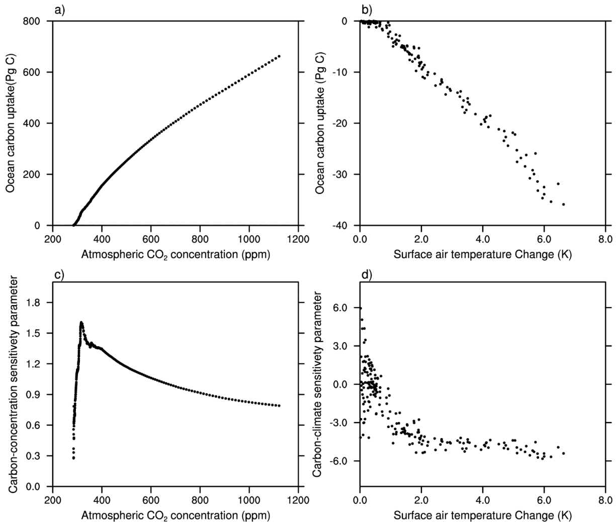
Figure 16. The cumulative oceanic CO 2 uptake against (a) the atmospheric CO 2 in the BC-HistSSP simulation (a) and (b) the global mean surface air temperature change in the RC-HistSSP simulation (b). Also shown is the time evolution of the diagnosed (c) carbon-concentration sensitivity parameter as a function of atmospheric CO 2 (c) and (d) carbon-climate sensitivity parameter as a function of global mean surface air temperature change (d). All the parameters in this figure are diagnosed from HistSSP scenarios
