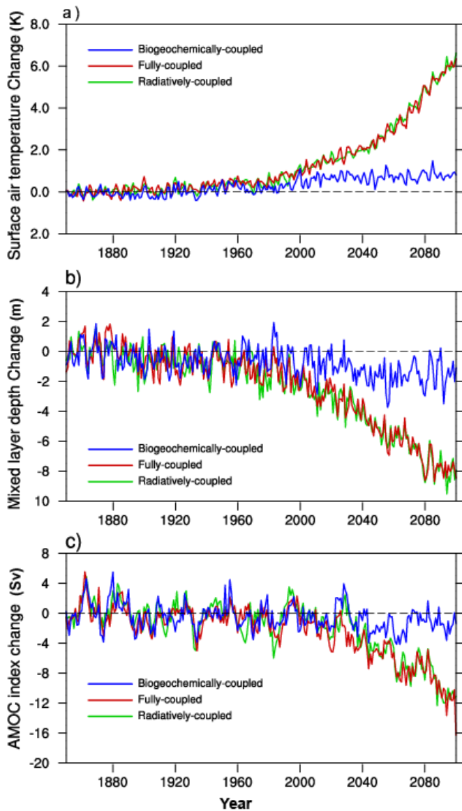
5 Figure 13. Time series of changes in climate changesfields (relative to control simulation) from 1850 to 2100 for the simulation of fully-coupled, biogeochemically-coupled BC-HistSSP, FC-HistSSP, and radiatively-coupled simulations RC-HistSSP. (a) global and annual mean surface air temperature (in the unit of K), (b) global and annual mean mixed layer depth (in the unit of meter, the mixed layer depth is defined to be the depth where the difference in potential density is 0.01 \text{ kg m}^{-3} relative to the sea surface) and (c) Atlantic meridional overturning circulation index (in the unit of Sv, maximum zonal mean stream function in the Atlantic Ocean at 30^\circ\text{N} ).
