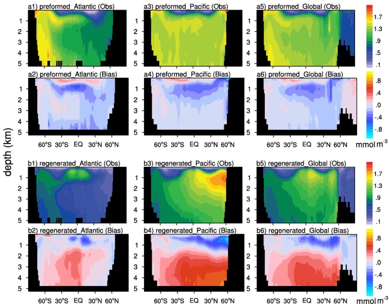
Figure 3. Latitude-depth distribution distributions of preformed and regenerated phosphate concentration ( \text{mmol m}^{-3} ) in the Pacific, Atlantic, and global Ocean averaged over 1985 to 2014. The results diagnosed from the WOA18 observation dataset are shown in the first and third rows (a1, a3, a5, b1, b3, and b5). The difference (model minus observation) between NESM v3 simulations and observation are shown in the second and the last rows (a2, a4, a6, b2, b4, and b6). The panels from a1 to a6 show the preformed component, and the panels from b1 to b6 show the regenerated component.
