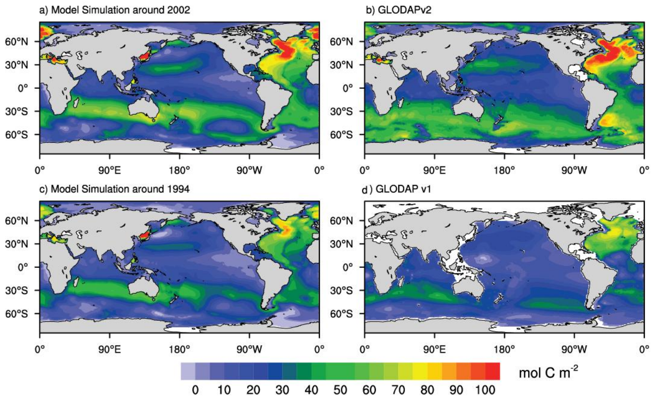
Figure 11. Vertically integrated column inventory of anthropogenic DIC ( \text{mol C m}^{-2} ) from the simulation (a, c), GLODAP v2 (b) and GLODAP v1 and GLODAP v2 observation ( b, d ). Model simulation results are averaged from 2000 to 2004 (a, represent the period around 2002 ) and from 1992 to 1996 (c, while the observation is, represent the period around 1994 ). The anthropogenic DIC from GLODAP v2 are normalized to the year 2002 ( b) and ), while that from GLODAP v1 are normalized to the year 1994 (d) .
