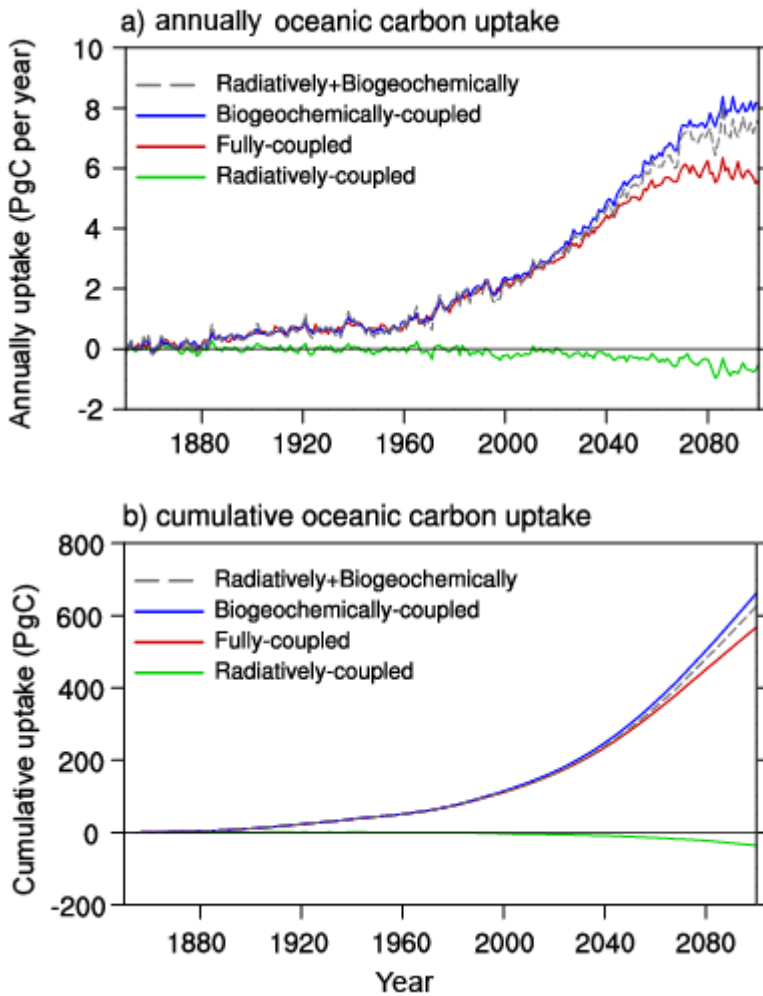
5 Figure 14. The NESM v3 simulated (a, in the unit of \text{PgC yr}^{-1} ) annually anthropogenic oceanic CO 2 uptake change (a, in the unit of \text{PgC yr}^{-1} ) and (b, in the unit of \text{PgC} ) cumulative oceanic CO 2 uptake (b, in the unit of \text{PgC} ) for the simulations RC-HistSSP, BC-HistSSP, FC-HistSSP, and the linear sum of BC-HistSSP and RC-HistSSP from 1850 to 2100.
