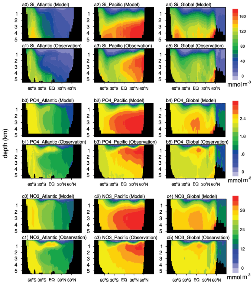
Figure 2. The latitude-depth distributiondistributions of silicate (a), phosphate (b), and nitrate (c) averaged fromover the years 1985 to 2014 from the NESM v3 simulation (FC- HistSSP ) and the WOA18 observation dataset ( with in the unit of \text{mmol m}^{-3} ). a, b, and c represent the silicate, phosphate, and nitrate, respectively. a1, a2, b1, b2, c1, and c2 represent the distributions in the Pacific Ocean, a3, a4, b3, b4, c3, and c4 represent the distributions in the Atlantic Ocean, and a5, a6, b5, b6, c5, and c6 represent the distributions in the Global Ocean.
