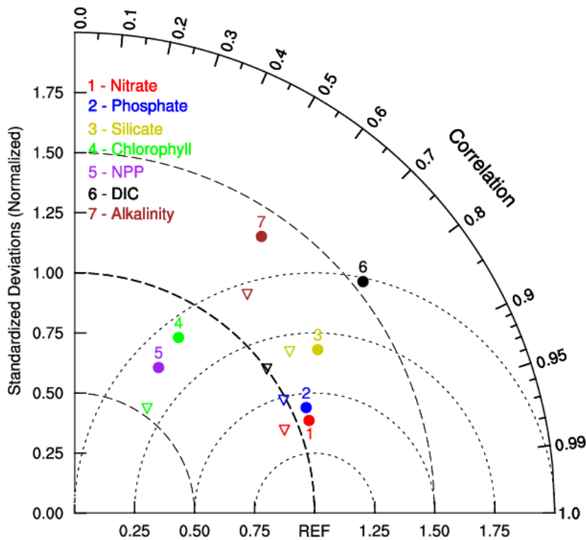
Figure 9. Taylor diagram comparing statistical patterns of annual mean biogeochemical fields averaged over the upper 100m ocean between the NESM v3 simulation (FC-HistSSP) and corresponding observations, including upper 100-m ocean nitrate, phosphate, silicate, alkalinity, chlorophyll concentration, and vertically-integrated net primary production. Nutrient concentrations are compared with WOA 18; DIC and alkalinity concentration are compared with GLODAP v2; NPP is compared with the CbPM, and ; chlorophyll is compared with SeaWiFS. All fields are normalized by the standard deviation of corresponding observations. Thus, observation fields have a standard deviation of one, which is represented by REF. The distance between the model points and the reference point indicates the root-mean-square (RMS) difference between model simulation and observations. The solid cycle represents the results diagnosed from the NESM v3, and the triangle represents the results from the IPSL, that shares the same marine biogeochemical model as the NESM v3 . The NPP of IPSL is not shown here.
