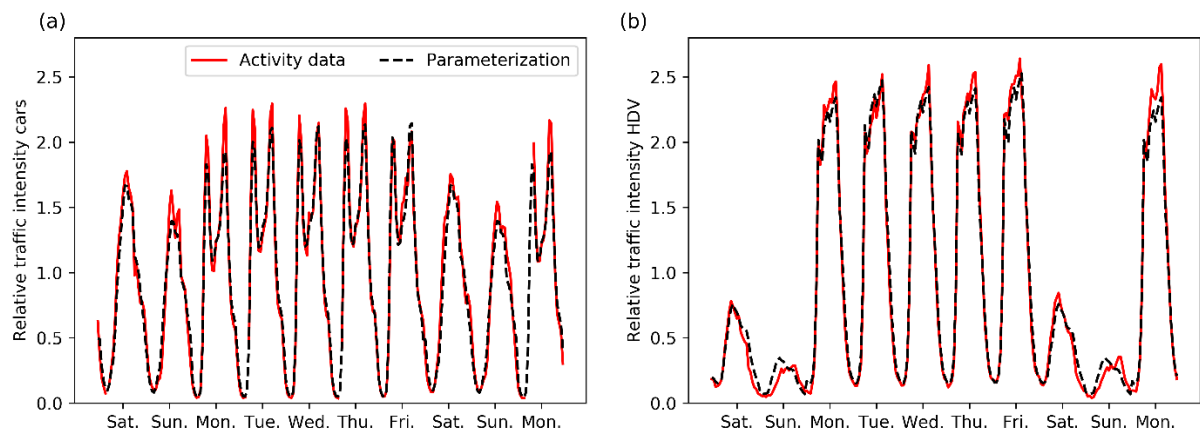
Figure 5. Time profiles of passenger cars (a) and heavy-duty vehicles (b) road transport on highways for ten randomly chosen days in March. Solid red lines are based on true activity data, whereas dashed black lines are parameterizations based on averaged traffic counts for Rotterdam.
