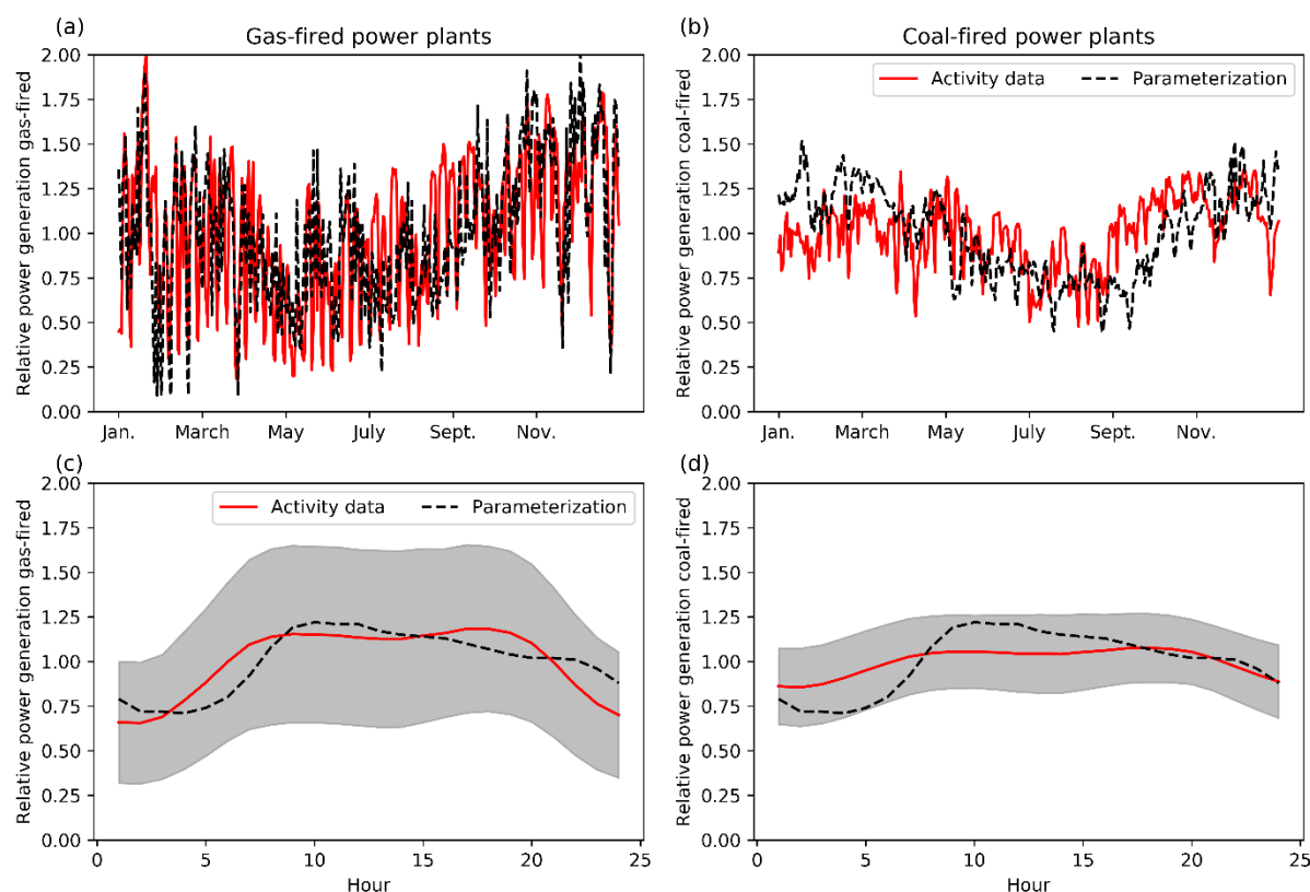
Figure 4. (top row) Daily time profiles for gas-fired (a) and coal-fired (b) power plants. Solid red lines are based on true activity data, whereas dashed black lines are parameterizations based on observed temperature (coal) and wind speed/radiation (gas). (bottom row) Average diurnal cycle for gas-fired (c) and coal-fired (d) power plants. Solid red lines are based on true activity data, whereas dashed black lines are fixed profiles from the MACC inventory (Denier van der Gon et al., 2011; Kuenen et al., 2014). Shading gives the 1\sigma variability of the diurnal cycle based on activity data.
