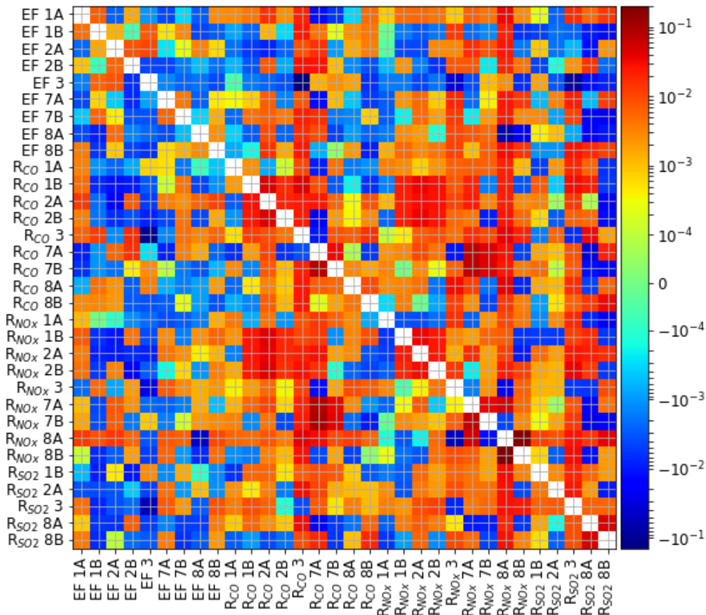
Figure D1. Matrix showing the difference in correlation coefficient ( r ) between the CO 2 _only_no_propagation and No_propagation run averaged for all 14 days, where positive differences indicate reduced parameter correlations when all tracers are included ( No_propagation ). (Sub)sectors are indicated with their short names as summarized in Table 1. For some parameters a strong reduction in parameter correlations is shown, indicating that with all tracers that parameter can be more easily separated from others, for example the emission factors of industry and coal-fired power plants (EF3 and EF1B).
