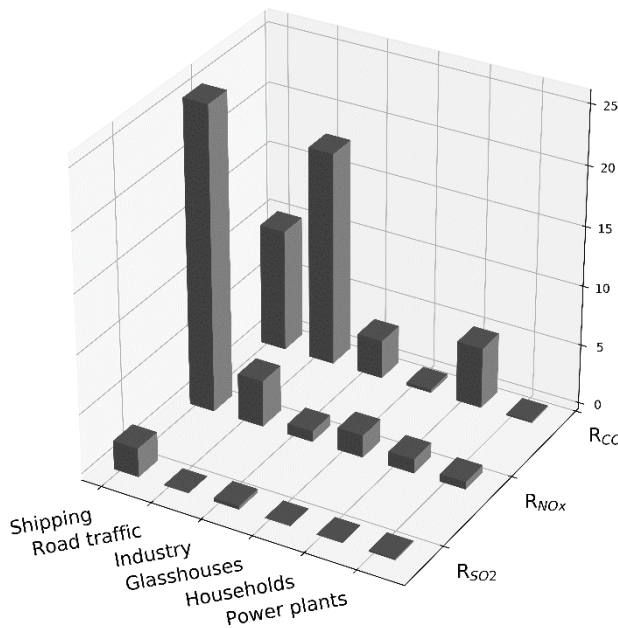
Figure 2. Emission ratios of \text{CO}:\text{CO}_2 ( R_{\text{CO}} ), \text{NO}_x:\text{CO}_2 ( R_{\text{NO}_x} ) and \text{SO}_2:\text{CO}_2 ( R_{\text{SO}_2} ) for specific source sectors based on the Dutch Pollution Release and Transfer Register (Netherlands PRTR, 2014). Units are in \text{ppb ppm}^{-1} . A value of 10 on the y-axis thus implies that for each 1000 moles of \text{CO}_2 , 10 moles of the auxiliary tracer is emitted.
