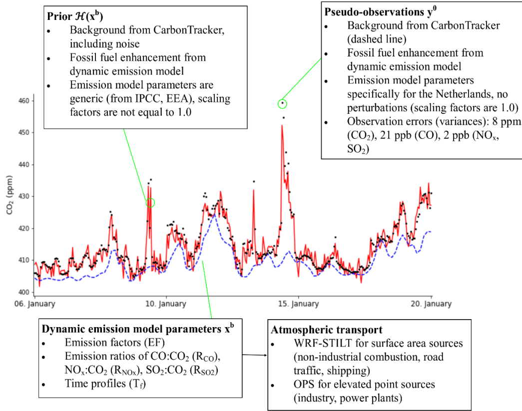
Figure 7. Time series of pseudo-observations and prior \text{CO}_2 mole fractions and a summary of how these time series were created.
