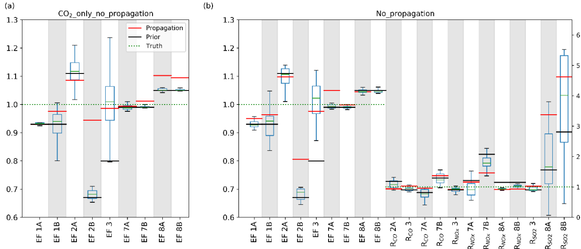
Figure 11. Spread (Q1-Q3) and median values of the parameter scaling factors for the fourteen individual days included in the CO 2 _only_no_propagation (a) and No_propagation (b) inversions, and final value of the CO 2 _only (left) and base (right) inversion (red lines). The prior values are indicated by the black lines and the truth is indicated with the green dotted lines (value of 1.0). The left y-axis is for the emission factors, the right y-axis for the tracer ratios. The inversion with all tracers shows more variability in the emission factors and larger deviations from the prior values.
