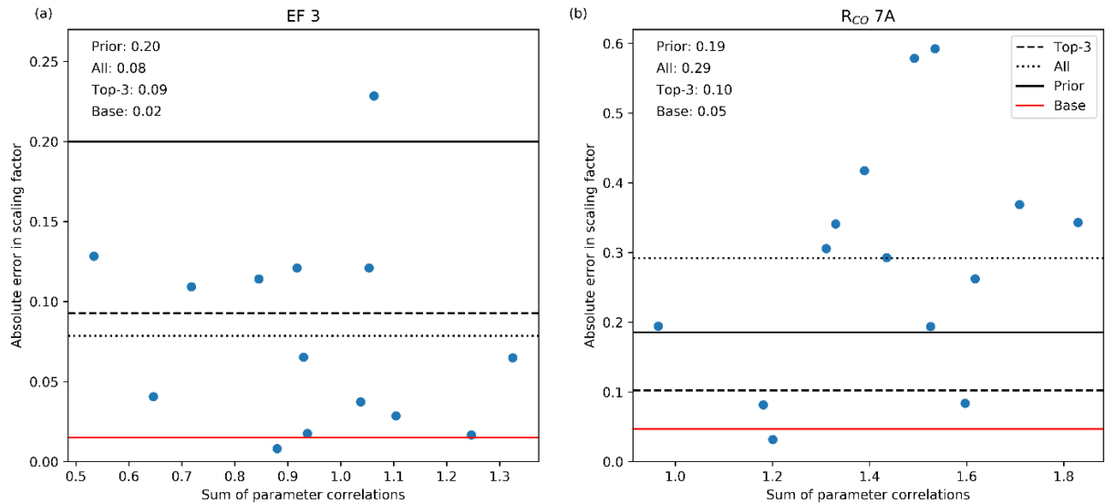
Figure 13. Scatter plot of the absolute error in the scaling factor of the industrial emission factor (EF 3) and R_{CO} of road traffic (7A) against the sum of the parameter correlations of the same parameters. The correlation coefficients are -0.17 and 0.37 respectively. The horizontal lines give the average absolute error in the scaling factor for the prior (full black line), if all 14 days are averaged (dotted line), and based on the 3 days with the smallest parameter correlations (dashed line) and the result for the base run (full red line). The values are also given.
