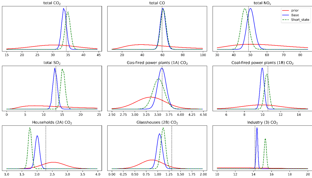
Figure 10. Probability density functions of emissions per species or per source category (for CO 2 ) in units of Tg (CO 2 ) or Gg (CO, NO x , SO 2 ). The truth is shown as a vertical dotted line, typically well-matched by the mean of the posterior in blue. Using a shortened state vector (green dashed line) deteriorates the total non-CO 2 emissions substantially and leads to misattribution of CO 2 emissions in minor categories such as 2A (households).
