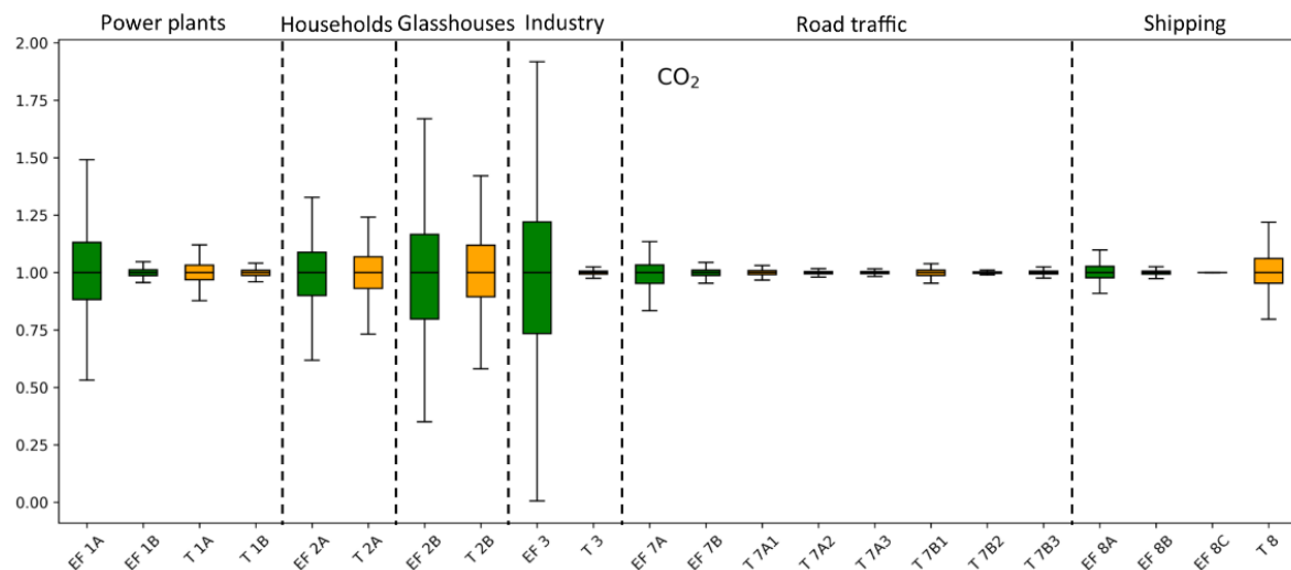
Figure 9. Box plots showing the uncertainty in the CO 2 emissions from power plants (1A+1B), households (2A), glasshouses (2B), industry (3), road traffic (7A+7B) and shipping (8A+8B+8C) caused by individual parameters affecting that sector. Uncertainty is represented as the spread in daily (normalized) emissions from each ensemble member (N=500) for a randomly chosen day. EF refers to an emission factor (green bars) and T to a time profile (orange bars). (Sub)sectors are indicated with their short names as summarized in Table 1. Note that the time profiles of road traffic emissions are specified per road type (1 = highway, 2 = main road, 3 = urban road). Minor parameters that have very small impacts on CO 2 emissions are not shown here (23 out of 44).
