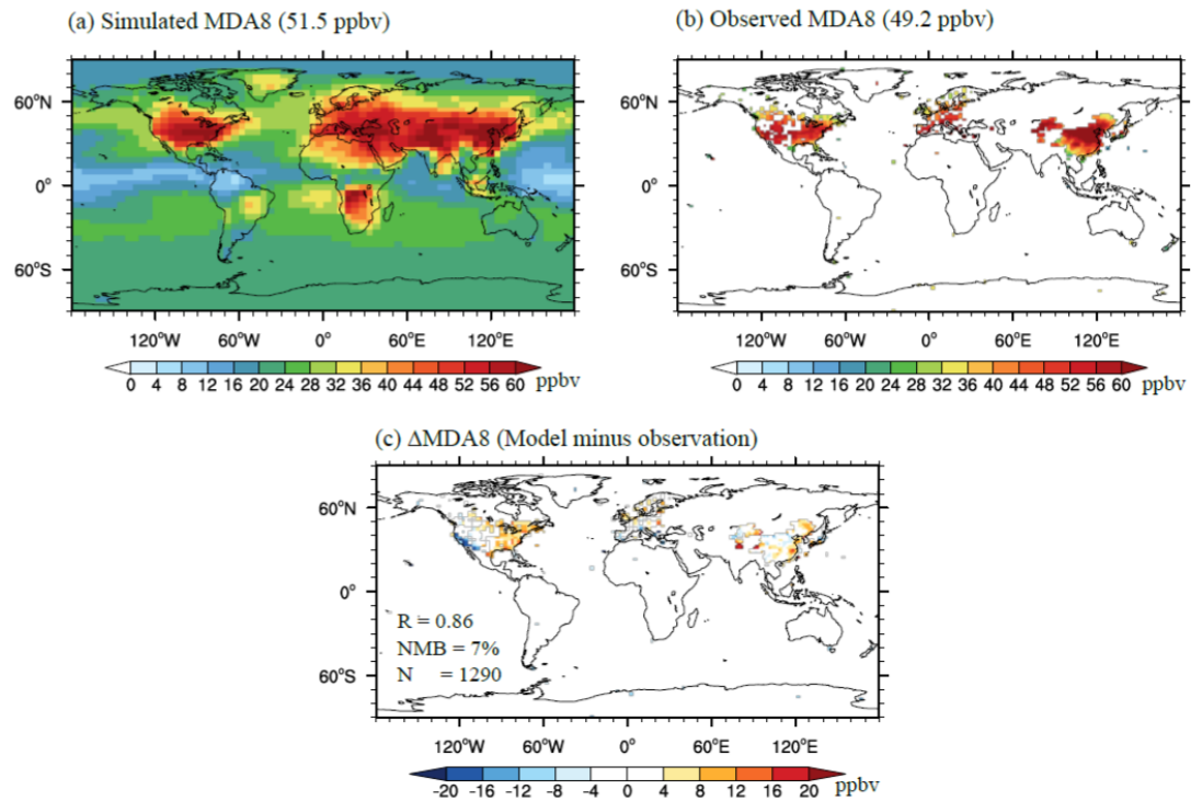
7 Figure S1 Summertime mean surface O_3 concentrations from (a) simulations, (b) 8 observations, and (c) their differences averaged for period of 2010-2012. Global area- 9 weighted surface O_3 concentrations over grids with available observations are shown 10 on the title brackets. The correlation coefficient (R), global normalized mean biases 11 (NMB), and grid numbers (N) with observations are shown in the bottom figure.
