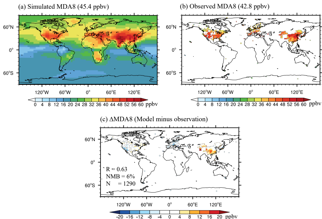
845 Figure 3 Annual surface O_3 concentrations ( [O_3] ) from Offline simulations (a), 846 observations (b), and their differences (c) averaged for period of 2010-2012. Global 847 area-weighted surface [O_3] over grids with available observations are shown on the 848 title brackets. The correlation coefficient (R) and global normalized mean biases 849 (NMB) are shown in the bottom figures with indication of grid numbers (N) used for 850 statistics.
