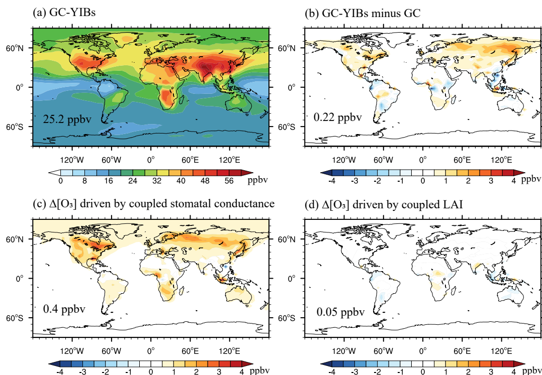
855 Figure 4 Simulated annual surface [O_3] from online GC-YIBs model (a) and its 856 changes (b-d) relative to Offline simulations. Changes of [O_3] are caused by (b) 857 jointly coupled LAI and stomatal conductance (Online_ALL – Offline), (c) coupled 858 stomatal conductance alone (Online_ALL – Online_LAI), and (d) coupled LAI alone 859 (Online_ALL – Online_GS). Global area-weighted [O_3] or \Delta[O_3] are shown in the 860 figures.
