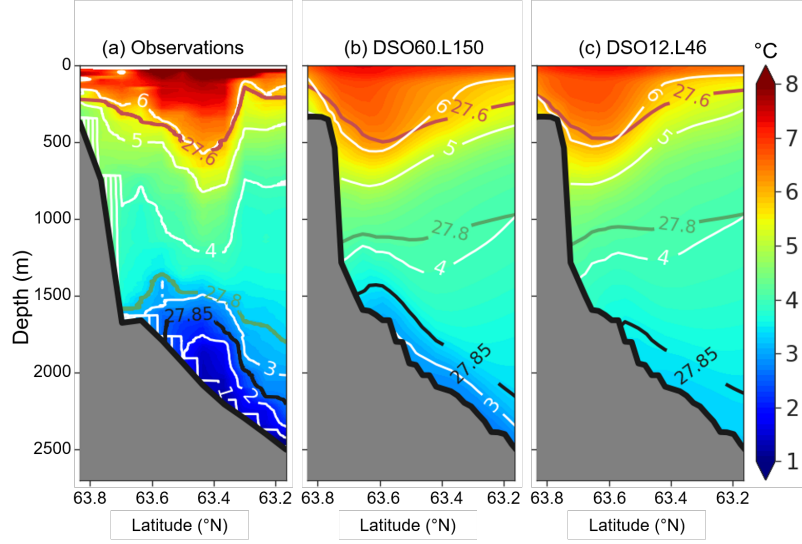
Figure 5. Potential Temperature (°C) at section 29 in (a) the observations (ASOF6-section, Quadfasel (2010) ), (b) the 1/60°, 150 levels simulation (annual mean), and (c) the 1/12°, 46 level simulation (annual mean). Red/Green/Black full lines are isopycnals 27.6/27.8/27.85. White lines are isotherms by 1°C interval. In panel b), the section 29 is outside ( 100 km downstream) the 1/60° AGRIF zoom, so the effective resolution is 1/12°. But the water masses acquired their properties upstream within the 1/60° resolution zoom.
