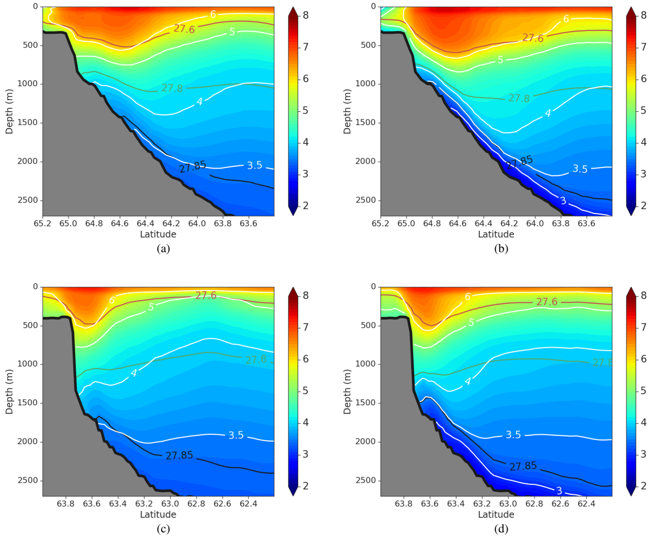
Figure 7. As in Fig. 6 at Section 24 ( TTO array) for a) simulation DSO12.L46 and b) simulation DSO60.L150 , and at Section 29 ( Angmagssalik array) for c) simulation DSO12.L46 and d) simulation DSO60.L150 .
