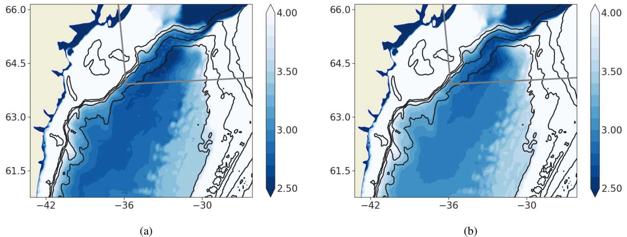
Figure 12. Annual mean of the bottom temperature in the 5th year of simulations using a grid refinement of 1/60^\circ for a) 150 vertical levels (DSO60.L150) and b) 300 vertical levels (DSO60.L300). Isobaths 500m, 1000m, 1500m and 2000m are contoured in black. The white box indicates the area of refinement.
