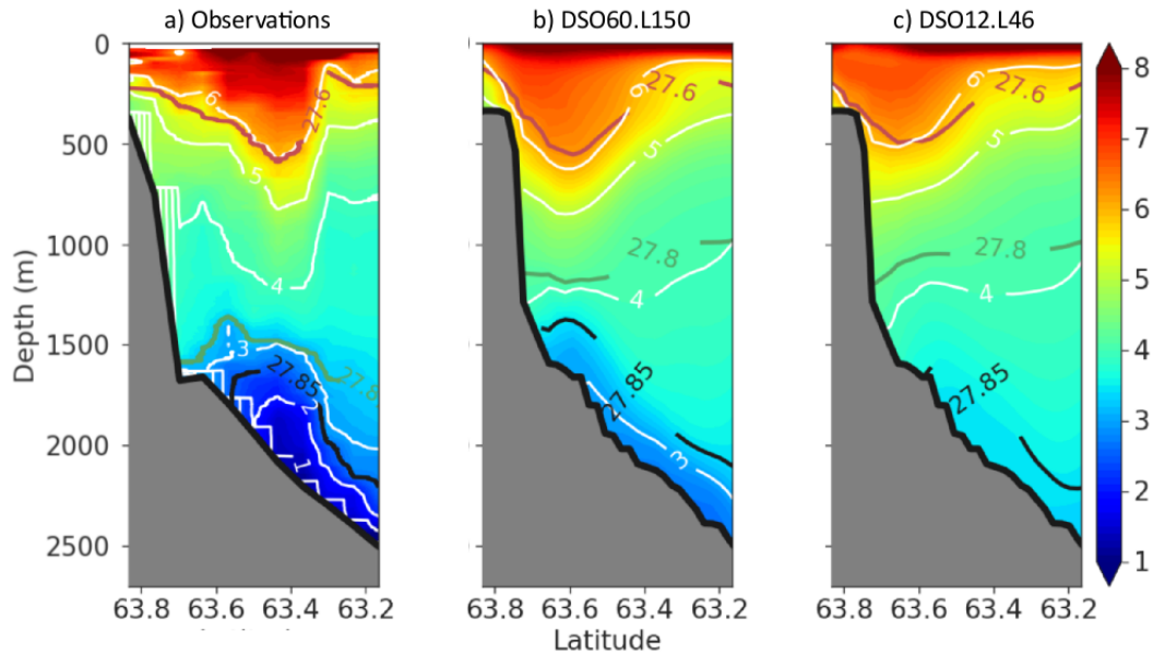
Figure 5. Potential Temperature ( ^{\circ}\text{C} ) at section 29 in (a) the observations (ASOF6-section, Quadfasel (2004)), (b) the 1/60^{\circ} , 150 levels simulation (annual mean), and (c) the 1/12^{\circ} , 46 level simulation (annual mean). Red/Green/Black full lines are isopycnals 27.6/27.8/27.85. White lines are isotherms by 1^{\circ}\text{C} interval. In panel b), the section 29 is outside ( 100 km downstream) the 1/60^{\circ} AGRIF zoom, so the effective resolution is 1/12^{\circ} . But the water masses acquired their properties upstream within the 1/60^{\circ} resolution zoom. Observation data were downloaded at: https://doi.pangaea.de/10.1594/PANGAEA.890362
