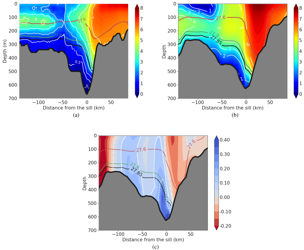
Figure 4. Mean flow characteristics (annual mean of year 76) in the global simulation at the sill. Temperature ( ^{\circ}\text{C} ) in colours and white contours for (a) the observations (Mastropole et al. (2017)) and (b) the control simulation ( 1/12^{\circ} and 46 vertical levels). Potential density values ( \sigma_0 ) are shown by the contour lines coloured in red (27.6), green (27.8) and black (27.85). (c) The velocity normal to the section in the control simulation (southward velocity in blue colour being negative). White lines indicate the 0\text{m s}^{-1} contour (dashed-dotted line), the -0.1\text{m s}^{-1} (full line) and the -0.2\text{m s}^{-1} contour (dashed line). The model section being taken along the model coordinate, the topography is slightly different in the model.
