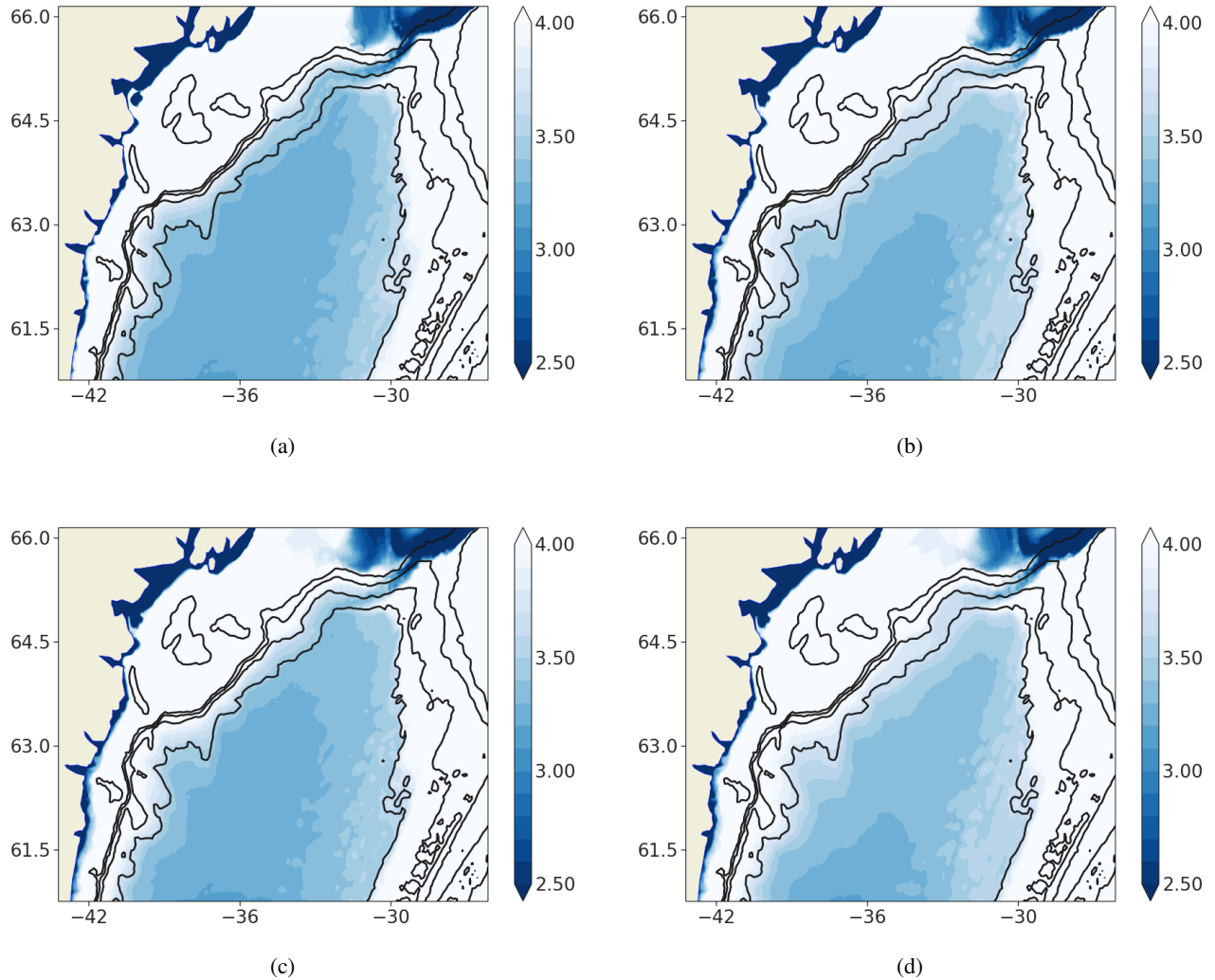
Figure 8. Annual mean bottom temperature (5th year of simulation) in ^\circ\text{C} at 1/12^\circ horizontal resolution in simulations differing the number of vertical levels. a) 46 levels (DSO12.L46) b) 75 levels (DSO12.L75), c) 150 levels (DSO12.L150) d) 300 levels (DSO12.L300). Isobaths 500m, 1000m, 1500m and 2000m are contoured in black.
