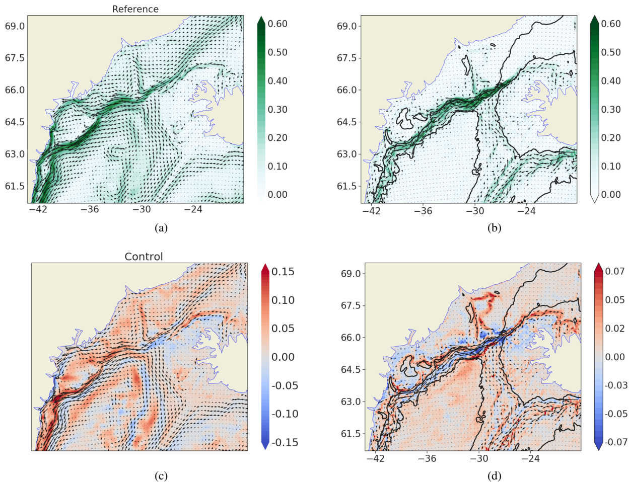
Figure 2. Surface (a) and bottom (b) mean currents (year 76) in the global ORCA12 simulation. Vectors/Colors indicate current direction/speed in m s^{-1} . Surface (c) and bottom (d) mean currents (year 76) in the regional DSO12.L46 regional simulation. Vectors indicate direction of the current. Colors indicate the current speed difference between the global and the regional simulation (in m s^{-1} ). Blue/red indicate that the current speed is greater/smaller in the global/regional simulation. Vectors at the bottom circulation are scaled by a factor of 7 compared to the surface for visibility reasons.
