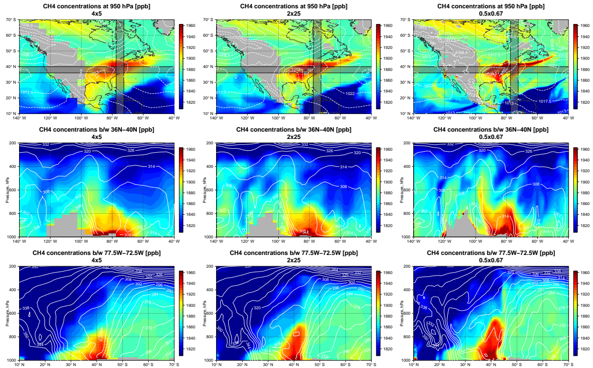
Figure 12. The distribution of \text{CH}_4 in GEOS-Chem at 12:00 UTC on 21 March 2010 at 4^\circ \times 5^\circ (left column), 2^\circ \times 2.5^\circ (middle column), and 0.5^\circ \times 0.67^\circ (right column). Top row: the distribution at 950 hPa, with sea level pressure indicated by the long-dashed white lines. Middle row: altitude-longitude cross section along the grey horizontal band in the figure in the top row. Bottom row: altitude-latitude cross section along the grey vertical band in the figure in the top row. The solid white lines in the figures in the middle and bottom rows indicate the moist isentropes.
