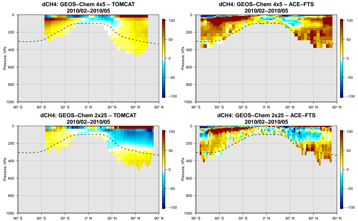
Figure 2. Zonal mean CH 4 differences (median value for the period of February - May 2010) in the stratosphere between GEOS-Chem at 4^\circ \times 5^\circ and the GOSAT CH 4 a priori fields (top left), GEOS-Chem at 4^\circ \times 5^\circ and ACE-FTS CH 4 retrievals (top right), GEOS-Chem at 2^\circ \times 2.5^\circ and the GOSAT CH 4 a priori fields (bottom left), and between GEOS-Chem at 2^\circ \times 2.5^\circ and ACE-FTS CH 4 retrievals (bottom right). The dashed line represents the mean dynamic tropopause averaged over February-May 2010 from the archived GEOS-5 meteorological fields.
