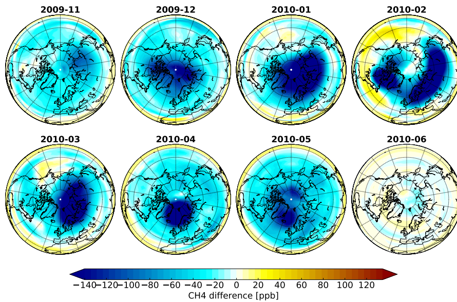
Figure 7. Monthly mean difference in CH 4 (in ppb) at 50 hPa (North Pole projection) between the GEOS-Chem 2^\circ \times 2.5^\circ and 4^\circ \times 5^\circ simulations.
