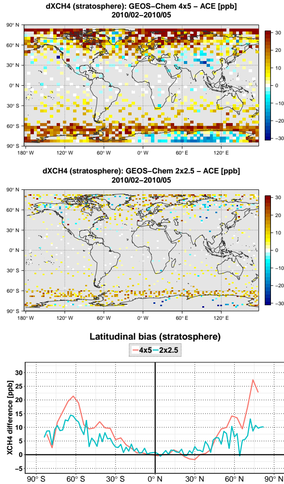
Figure 3. XCH 4 difference between GEOS-Chem and ACE-FTS due to the stratosphere, for GEOS-Chem at 4° × 5° (top panel) and at 2° × 2.5° (middle panel). The zonal mean difference for both model resolutions are shown in the bottom panel. XCH 4 differences were obtained by augmenting the ACE-FTS stratospheric profile with the GEOS-Chem troposphere and smoothing the vertical CH 4 difference profile with the mean zonal GOSAT averaging kernels.
