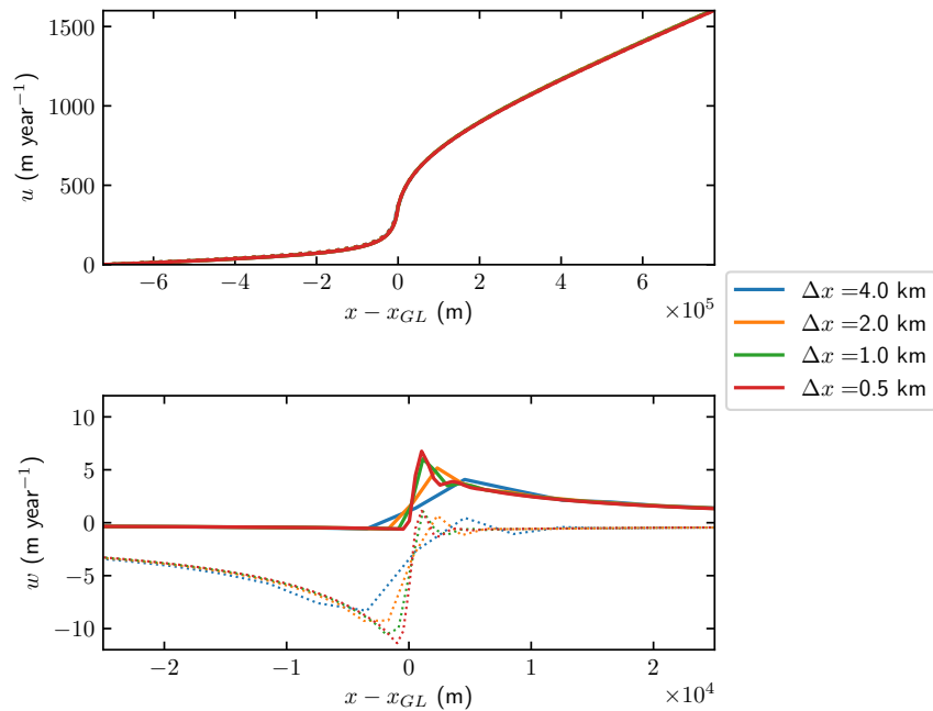
Figure 8. The velocities u (upper panel) and w (lower panel) of the ice in the advance experiment with \Delta x = 0.5, 1, 2, 4 km after 10000 years. The solutions at the upper surface are the solid curves, and the solutions at the lower surface are the dotted curves. The vertical velocity w is zoomed-in close to the GL with the distance to the mesh dependent GL on the x -axis.
