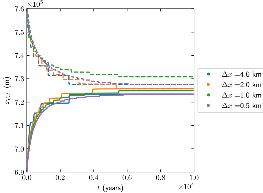
Figure 5. The MISIP 3a experiments for the GL position when t \in [0, 10000] with \Delta x = 4 km, 2 km, 1 km and 0.5 km for the advance (solid) and retreat (dashed) phases.
