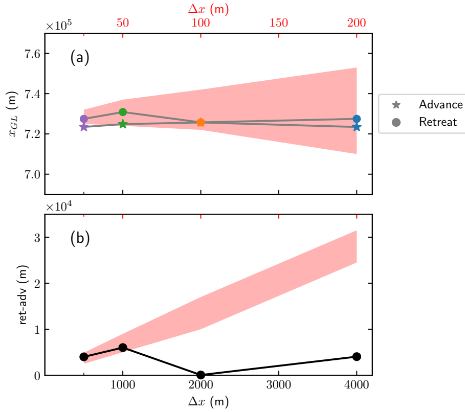
Figure 6. The MIS3a experiments at the final time t = 10000 with the resolutions at \Delta x = 4 km, 2 km, 1 km and 0.5 km. (a) The GL positions in the advance (★) and retreat (●) phases. (b) The distance between the retreat and the advance x_{GL} at the steady states. The shaded regions indicate the range of the results in Gagliardini et al. (2016) with 20 times smaller mesh resolutions from 25 to 200 m with the axis scale shown in red at the top of the plot.
