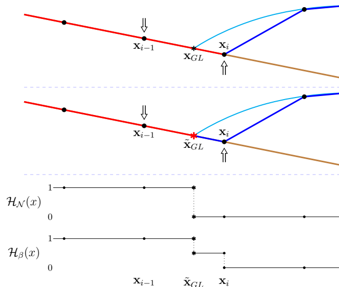
Figure 2. Schematic figure of the GL in case i, with the arrows indicating the direction of the net forces in the vertical direction. The light blue line is the analytical solution of the ice sheet with the analytical GL position \mathbf{x}_{GL} . The red line is the grounded boundary \Gamma_{bg} , the dark blue line is the floating boundary \Gamma_{bf} , and the brown line is the bedrock topography b(x) . Upper panel: The last grounded and first floating nodes as defined in Elmer/ICE. Middle panel: Linear interpolation to approximate the numerical GL position \tilde{\mathbf{x}}_{GL} . Lower panel: The step functions \mathcal{H}_N(x) and \mathcal{H}_\beta(x) indicate the area for Nitsche’s penalty and slip boundary conditions.
