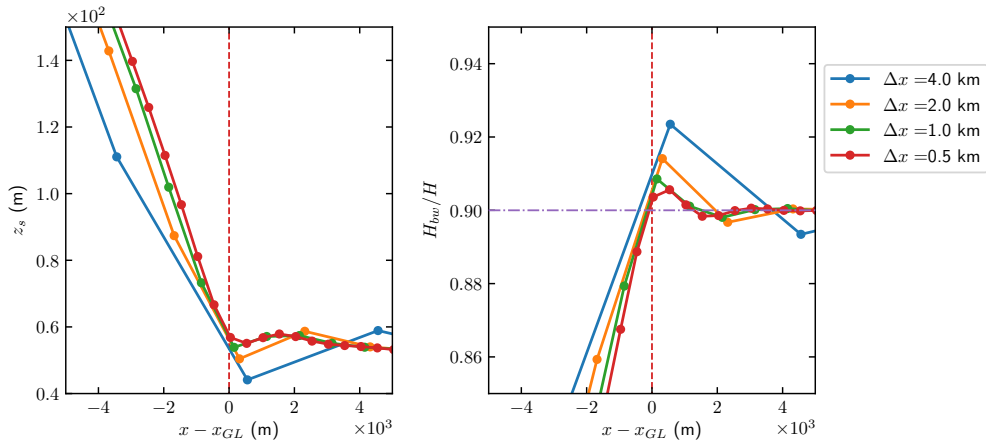
Figure 7. Details of the solutions for the advance experiment with \Delta x = 0.5, 1, 2, 4 km after 10000 years. The solid dots represent the nodes of the elements and the vertical, red, dashed lines indicate the GL position. Left panel: The oscillations in z_s at the ice surface near GL. Right panel: The flotation criterion is evaluated by H_{bw}/H . The ratio between \rho/\rho_w is drawn in a horizontal, purple, dash-dotted line.
