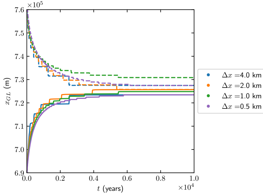
Figure 5. The MISMP 3a experiments for the GL position when t \in [0, 10000] with \Delta x = 4 km, 2 km, 1 km and 0.5 km for the advance (solid) and retreat (dashed) phases.
