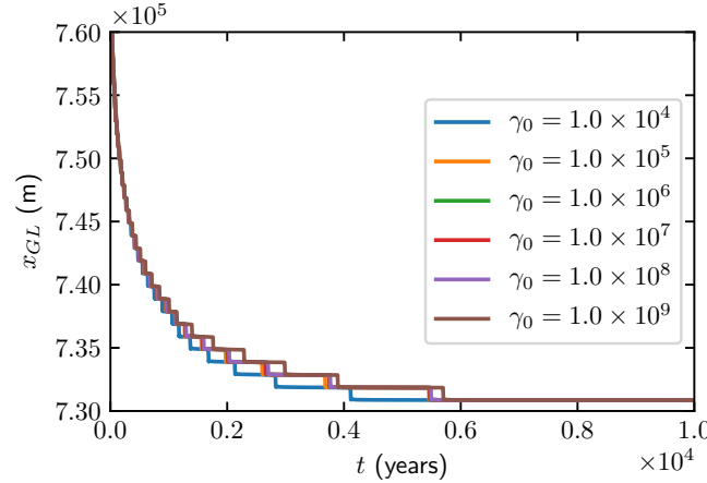
Figure 4. The MISIMIP 3a retreat experiment with \Delta x = 1 km for different choices of \gamma_0 in the time interval [0, 10000] years.
