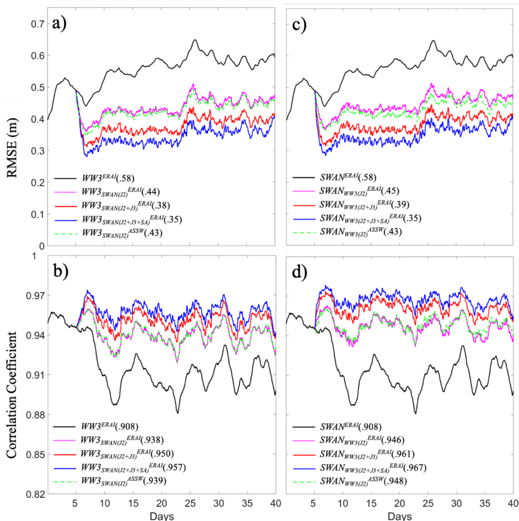
735 Figure 4: The time series of RMSEs (upper) and correlation coefficients (bottom) of the WW3(left) and SWAN(right) biased model experiments in the model control run forced by the ERA-Interim wind (black, denoted as WW3^{ERA1} and SWAN^{ERA1} ), assimilations with “observed” data from one (pink, denoted as WW3_{SWAN(J2)}^{ERA1} and SWAN_{WW3(J2)}^{ERA1} ), two (red, denoted as WW3_{SWAN(J2+J3)}^{ERA1} and SWAN_{WW3(J2+J3)}^{ERA1} ), and three (blue, denoted as WW3_{SWAN(J2+J3+SA)}^{ERA1} and SWAN_{WW3(J2+J3+SA)}^{ERA1} ) 740 satellites, as well as the assimilation with corrected wind (dotted green, denoted as WW3_{SWAN(J2)}^{ASSW} and SWAN_{WW3(J2)}^{ASSW} ) against the “truth” (same as in Fig. 3 but for SWAN and WW3 with the ERA-Interim wind). The numbers in the parentheses correspond to the RMSE (in panels a and c) and correlation coefficient (in panels b and d) over the last 30 days during the assimilation period. The “observed” data are produced by projecting the “truth” SWH onto the satellite orbit.
