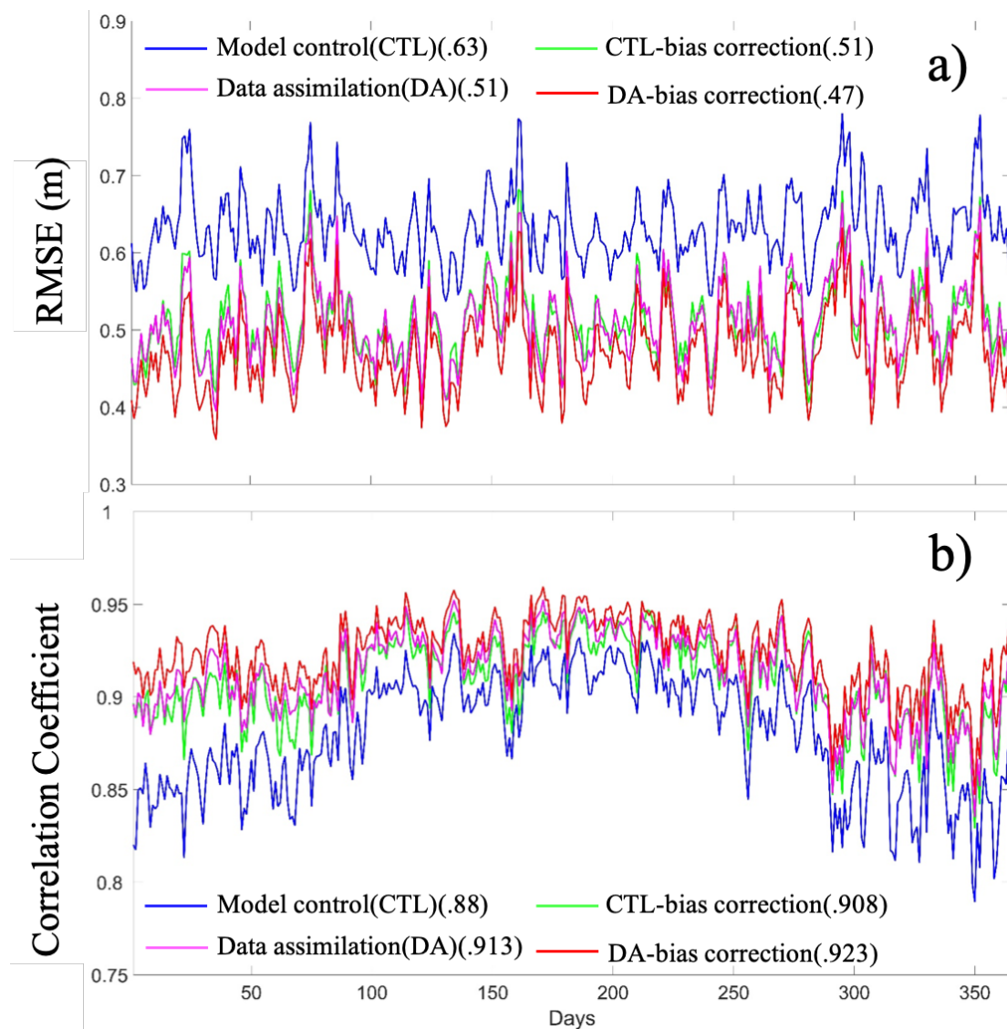
Figure 10: The time series of a) RMSEs and b) correlation coefficients produced by the model control run (blue), data assimilation (pink) and their corresponding bias corrections (green and red) combining three wave model assimilation results (WAM, WW3 and SWAN) over 1 year.
