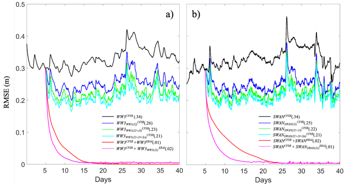
Figure 3: The time series of RMSEs of the a) WW3 and b) SWAN perfect model experiments in the model control run with the NCEP CFSRv2 wind (black, denoted as WW3^{CFSR} in panel a and SWAN^{CFSR} in panel b), assimilating the “observed” data sampled by the tracks of Jason-2 (blue, denoted as WW3_{WW3(J2)}^{CFSR} and SWAN_{SWAN(J2)}^{CFSR} ), Jason-2 & 3 (green, denoted as WW3_{WW3(J2+J3)}^{CFSR} and SWAN_{SWAN(J2+J3)}^{CFSR} ), as well as Jason-2 & 3 and SARAL (cyan, denoted as WW3_{WW3(J2+J3+SA)}^{CFSR} and SWAN_{SWAN(J2+J3+SA)}^{CFSR} ) against the “truth” simulation forced by the ERA-Interim wind. The red and pink are forced by the NCEP CFSRv2 wind in the first 45 days, but the next 35 days are forced using the ERA-Interim wind (same as “truth”) without (denoted as WW3^{CFSR} + WW3^{ERA-I} and SWAN^{CFSR} + SWAN^{ERA-I} ) or with (denoted as WW3^{CFSR} + WW3_{WW3(J2)}^{ERA-I} and SWAN^{CFSR} + SWAN_{SWAN(J2)}^{ERA-I} ) the assimilation of Jason-2 data. The number in parentheses for each color is the corresponding RMSE summed over the verification time period (30 days after the 45-day model spin-up and 5-day assimilation spin-up). The “observed” data are produced by projecting the “truth” SWH onto the satellite orbit.
