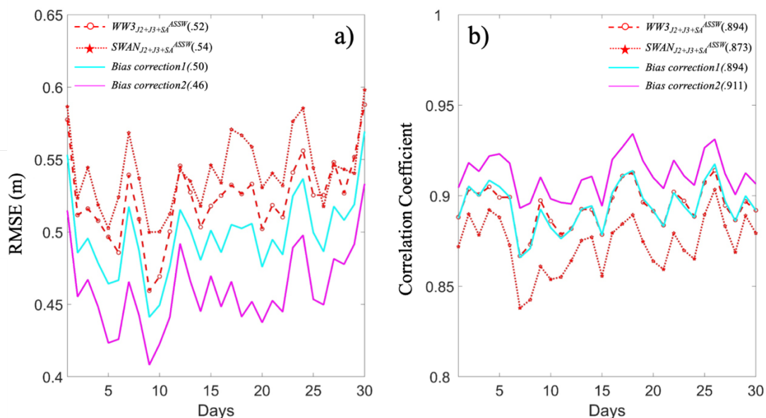
765 Figure 8: Time series of a) RMSEs and b) correlation coefficients produced by two bias correction schemes (cyan and pink) through a combination of WW3 and SWAN assimilations with the data from three satellites (Jason-2, Jason-3 and SARAL) and wind correction starting from the ERA-Interim wind. The results of the individual assimilation systems are plotted as dotted and dashed red lines (taken from Fig. 7) for reference.
