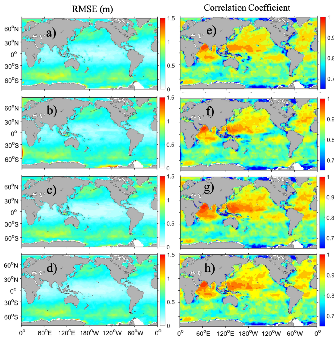
Figure 9: Distributions of SWH RMSEs (left) and correlation coefficients (right) (against the merged grid altimeter data) of the WW3 (a, e), SWAN (b, f) and WAM (c, g) assimilations and the bias correction (d, h). The statistics are conducted over the entire 1-year assimilation period. Other information is the same as that in Fig. 8.
