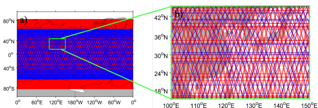
Figure 1: The ground projection tracks of satellite Jason-2 (blue line, with an inclination of 66° N(S)) and SARAL (red line, with an inclination of 88° N(S)) in one cycle over approximately 10 days and 35 days, respectively, in the a) global and b) East Asia domains (zoomed out of green box in panel a).
