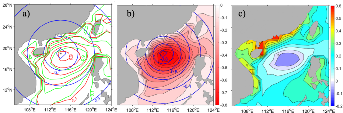
Figure 2: Spatial distributions of a) background correlation coefficients by the empirical correlation model (blue), model data statistics (green) as well as their combination of Eq. (3) (red), b) adjustment increments of SWH, and c) the SWH difference from panel b by an analysis process given the single observation obtained at 114.09° E, 18.90° N, denoted by the asterisk (unit: meter).
