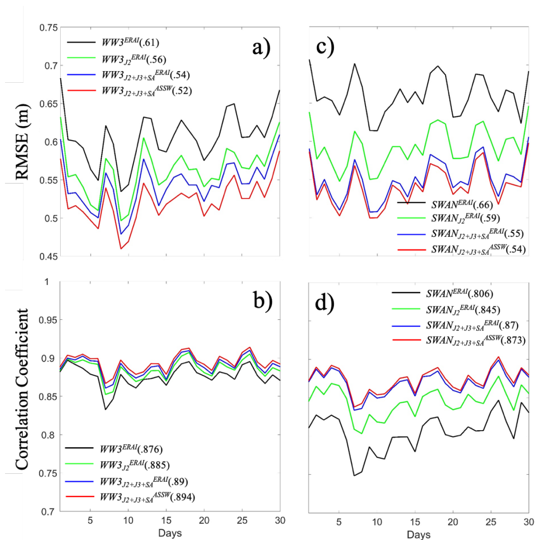
760 Figure 7: Time series of RMSEs (upper) and correlation coefficients (bottom) of WW3 (left) and SWAN (right) produced by the model control run (black, denoted as WW3^{ERA1} and SWAN^{ERA1} ), assimilation using the data from one (green, denoted as WW3_{J2}^{ERA1} and SWAN_{J2}^{ERA1} ) and three satellites (blue, denoted as WW3_{J2+J3+SA}^{ERA1} and SWAN_{J2+J3+SA}^{ERA1} ) with corrected wind (red, denoted as WW3_{J2+J3+SA}^{ASSW} and SWAN_{J2+J3+SA}^{ASSW} ).
