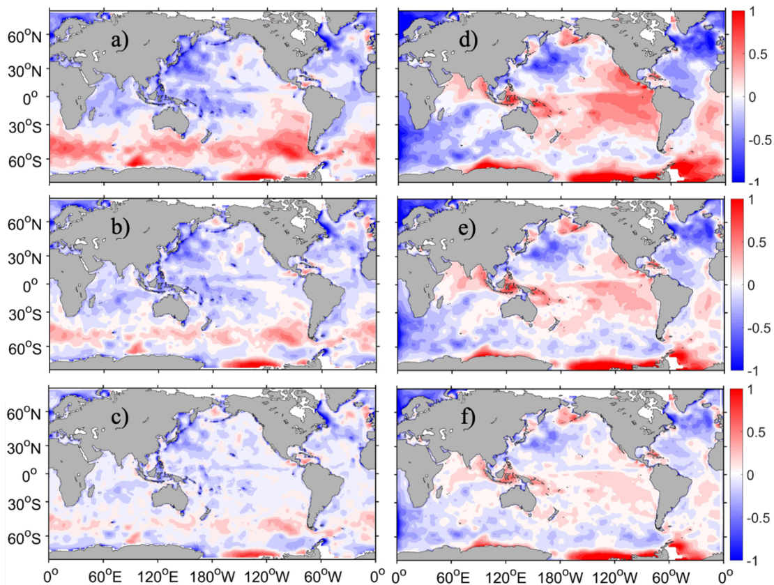
Figure 5: Distributions of SWH mean errors (against the merged grid altimeter data) of the WW3 (left) and SWAN (right) model simulations (upper) and assimilations with Jason-2 (middle), as well as all Jason-2, Jason-3 and SARAL (bottom) data forced by the ERA-Interim wind. The statistics are conducted over the last 30 days of a 70-day total assimilation period (unit: meter).
