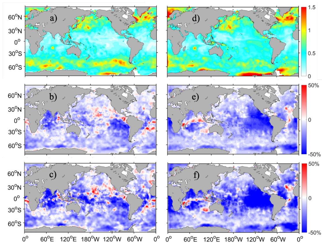
Figure 6: Same as Fig. 5 but for the RMSEs. Panels b, c, e and f show the percentage of RMSE reduction from the model control (unit: meter).
