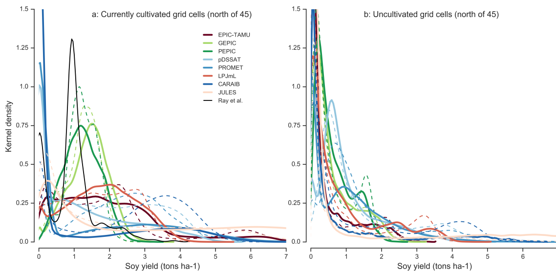
Figure 4. Model probability densities for soybean yields at latitudes north of 45^\circ in historical and warming simulations in the A0 case. While 10 GGCM Phase II models provide simulations (Table 3); we show 8 representative models for clarity. Probability density functions are estimated separately for locations with some current cultivation (left, approximately 2500 grid cells, unweighted by cultivated area) and for uncultivated locations (right, approximately 1500 grid cells), for baseline historical (solid) and T+4 ( ^\circ\text{C} ) (dashed) simulations. Black line in left panel shows actual yields from 1997-2003 derived from Ray et al. (2012). For historical simulations, models agree on low potential yields in currently uncultivated areas (right) but disagree widely on yields in currently cultivated areas (left). Color code groups models into those with realistic yield distributions peaking at 1\text{-}2\text{ ton ha}^{-1} (green), those with flatter distributions extending to unrealistically high values (red), and those with predominantly zero yields (blue). “Green” models show slight decreases under T+4 warming, “red” models moderate increases, and “blue” models large increases.
