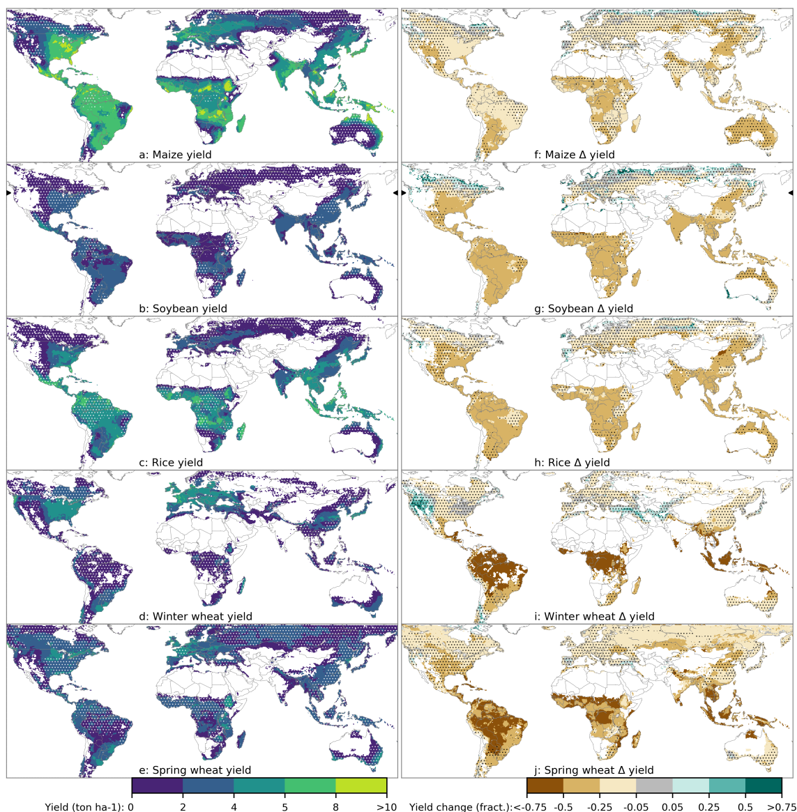
Figure 3. Illustration of the spatial patterns of baseline yields (left) and yield changes (right) in the GGCM Phase II ensemble. Left column shows multi-model climatological(30 year) median yields for the baseline scenario, with white stippling indicating areas where these crops are not currently cultivated. Areas with less than 0.5 \text{ ton ha}^{-1} in the baseline are masked. Absence of cultivation aligns well with the lowest yield contour ( 0-2 \text{ ton ha}^{-1} ). Right column shows multi-model mean fractional yield changes in the T+4 °C scenario relative to the baseline scenario. Areas without stippling are those where models agree on changes: the multi-model mean fractional change exceeds the standard deviation of changes in individual models. Stippling indicates areas of low confidence ( \Delta < 1\sigma ). Some spatial structure in projected changes at high latitudes may be due to differences in model coverage; see Figure 1.
