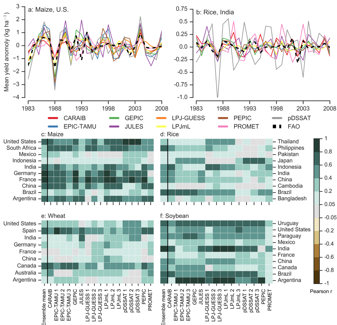
Figure 2. Assessment of crop model performance in GGCMII Phase II, following the protocol of GGCMII Phase I (Müller et al., 2017). Top: example timeseries comparison between simulated crop yield and FAO country statistics (FAO, 2018) at the country level for two example high production countries: US maize, and rice in India, both for the 200 \text{ kg ha}^{-1} nitrogen application level. Bottom: heatmaps illustrating the Pearson r correlation coefficient between the detrended simulated and observed country-level mean yields for the top 10 countries by production for each crop, of those countries with continuous FAO data over 1981-2010. We show separate comparisons for simulations with the three different nitrogen application levels, denoted 1, 2, 3 for 10, 60, and 200 \text{ kg N ha}^{-1} , respectively. Left column shows correlation of ensemble mean yields with FAO data. Because FAO does not distinguish between wheat types, we sum simulated spring and winter wheat for models that provide both (See Table 3.). Note that differences by region and crop are stronger than difference between models, e.g. horizontal bars are more similar in color than vertical bars. Countries are ordered alphabetically, not by production quantity.
