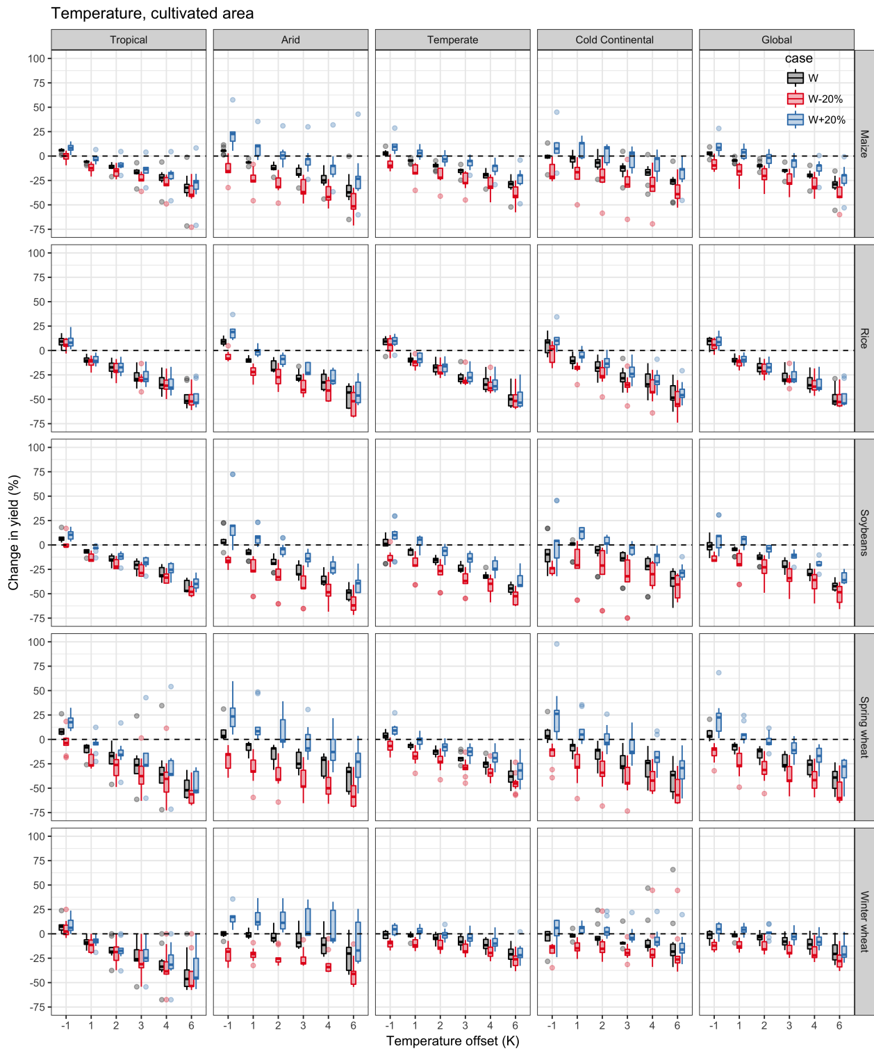
Figure S10: Same as main Figure 5a for all crops. Only over cultivated area.
