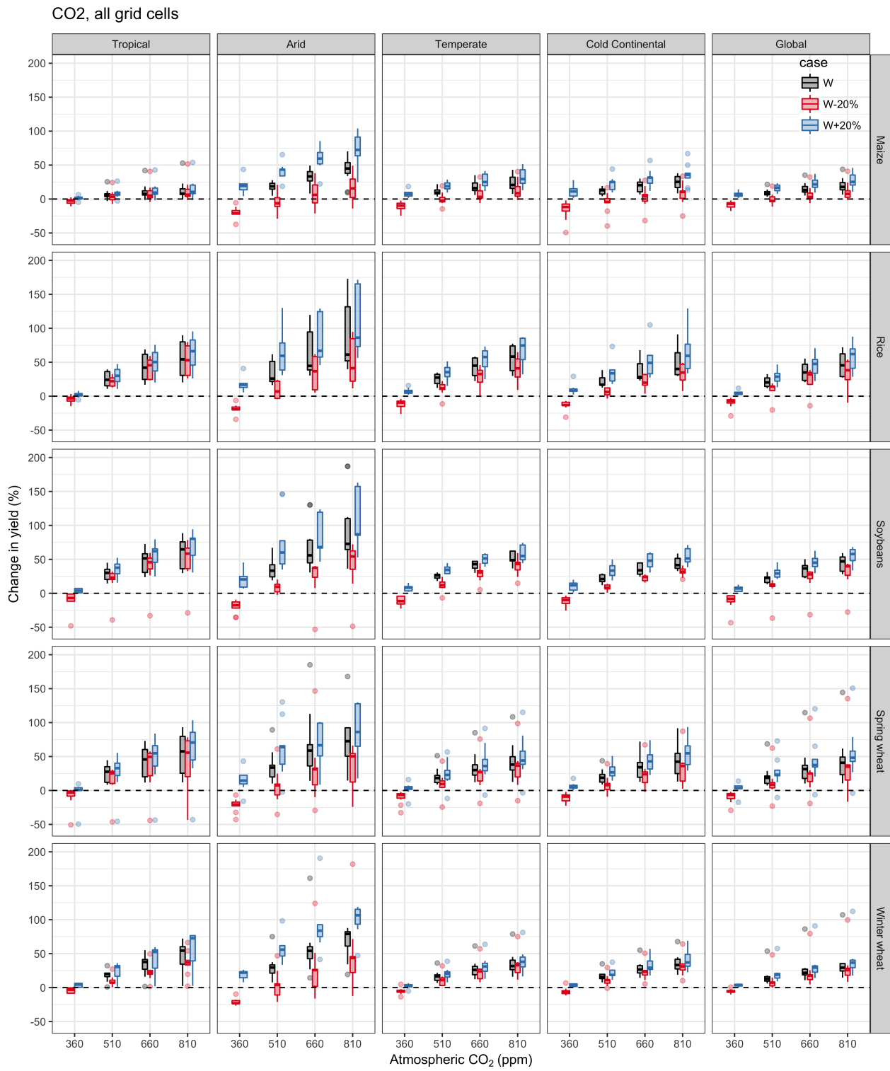
Figure S7: Same as main Figure 6a for all crops.
