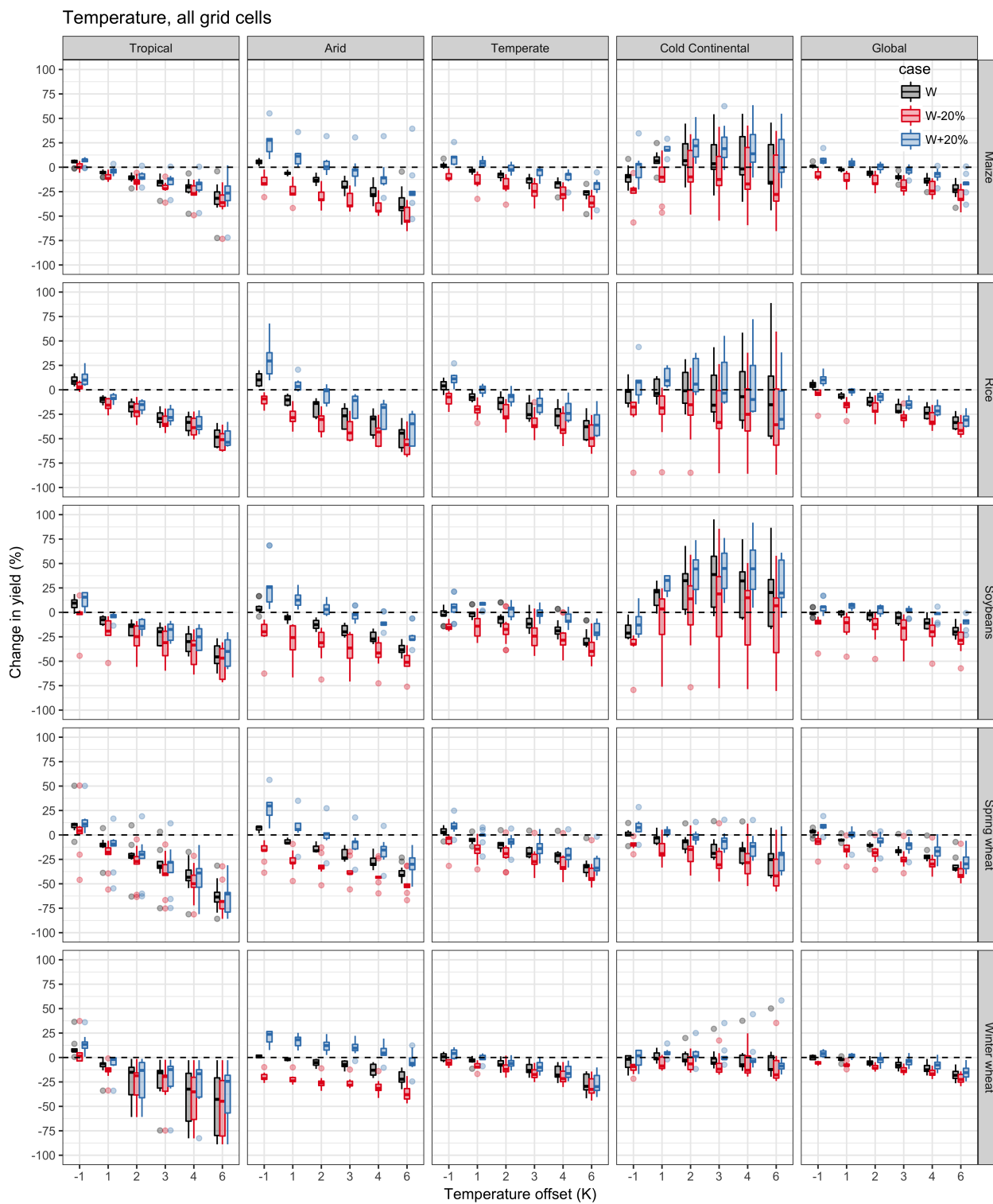
Figure S5: Same as main Figure 5a for all crops.
