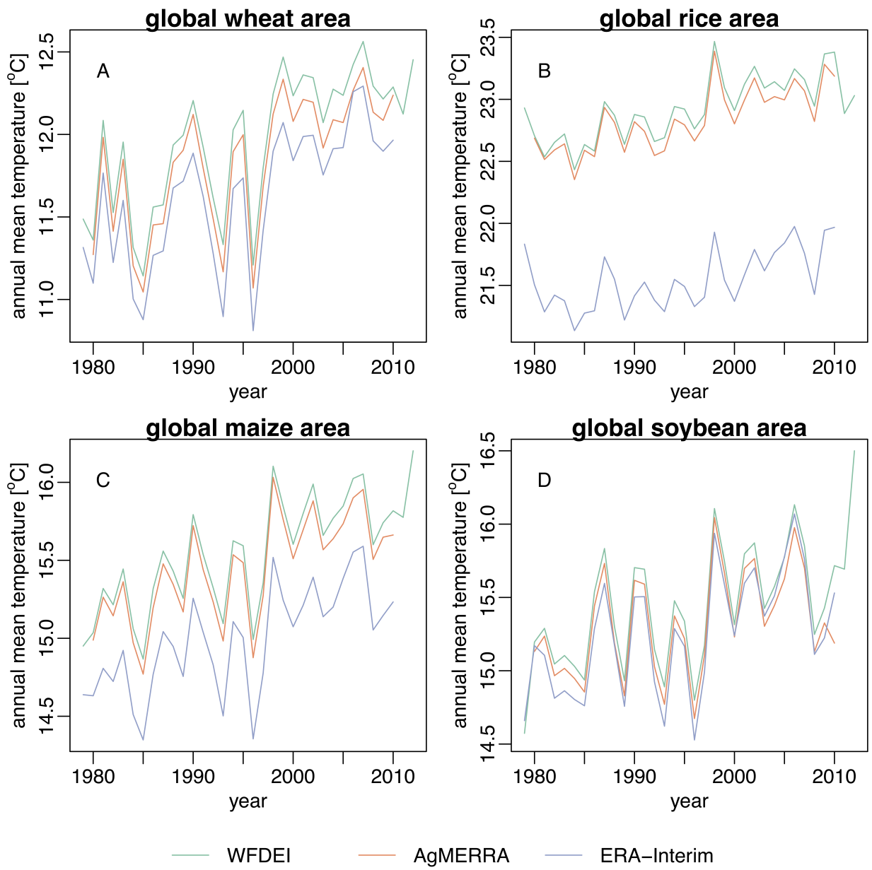
Figure S4: Same as Figure S3 but for temperature.
