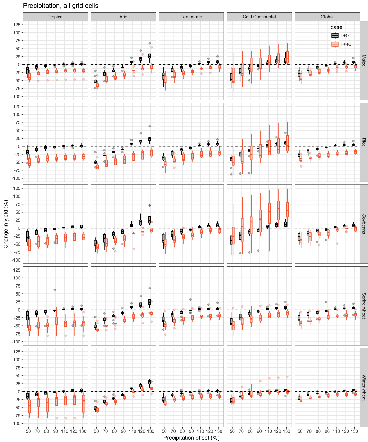
Figure S6: Same as main Figure 5b for all crops.
