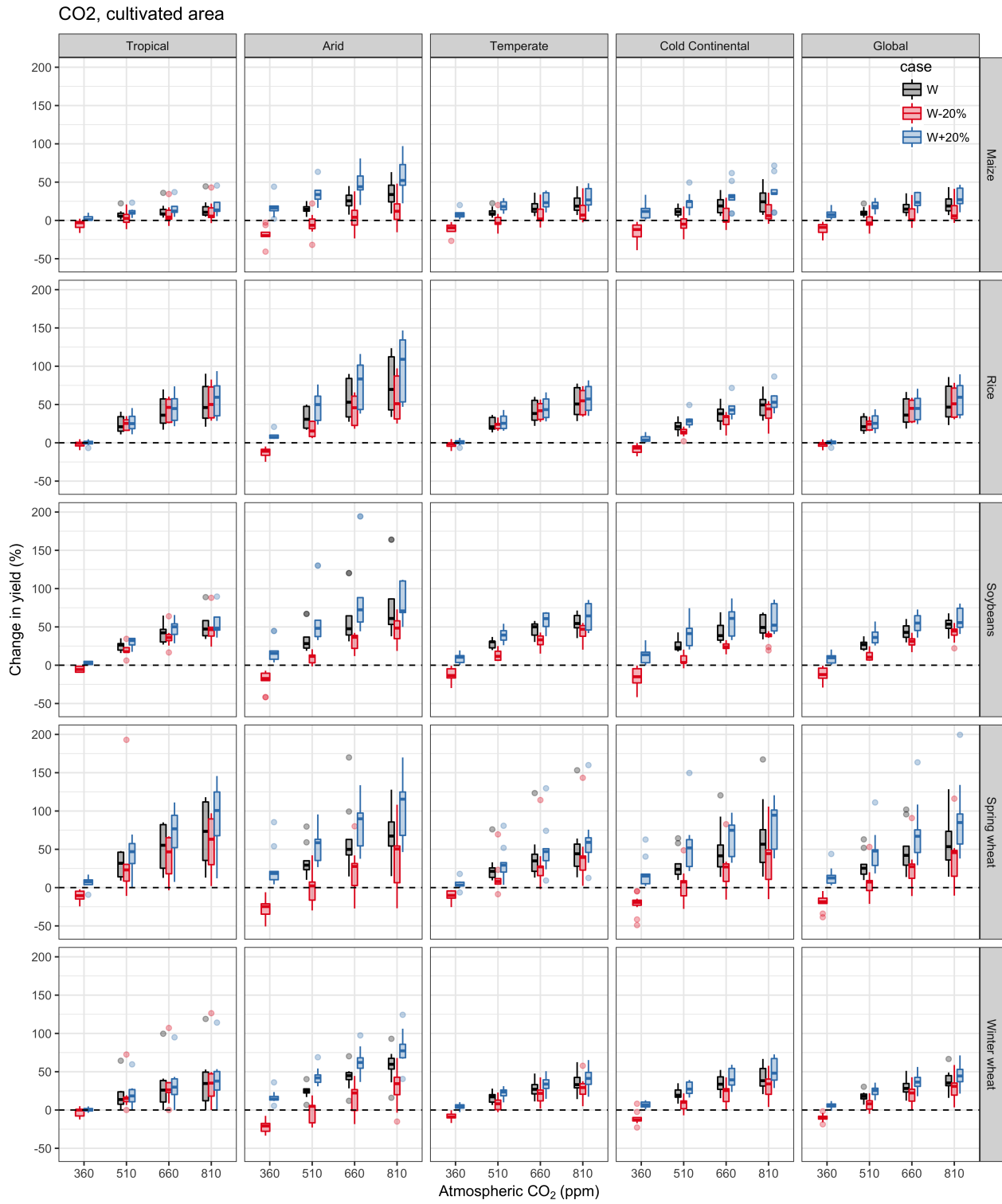
Figure S12: Same as main Figure 6a for all crops. Only over cultivated area.
