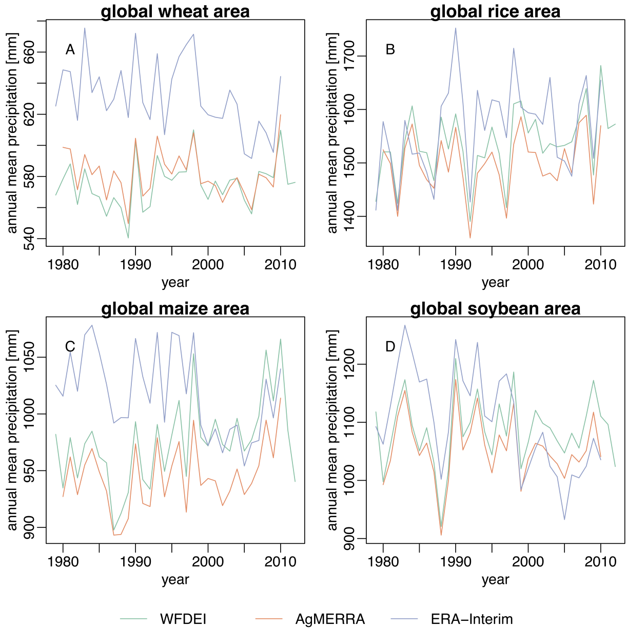
Figure S3: Comparison across the three reanalysis products used in GGCM Phase II. Values are aggregated across cultivation area based on the MIRCA2000 dataset.
