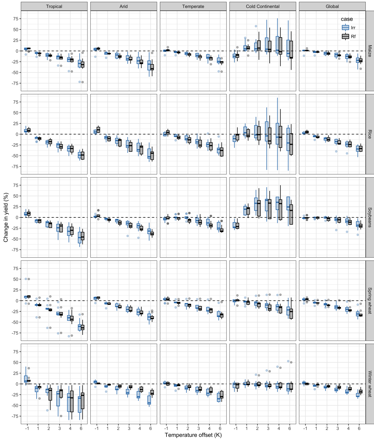
Figure S9: Same as main Figure 5a for all crops. Irrigated crops compared to rainfed. Note that yield change for irrigated crops is from the irrigated baseline, which is typically higher than rainfed.
