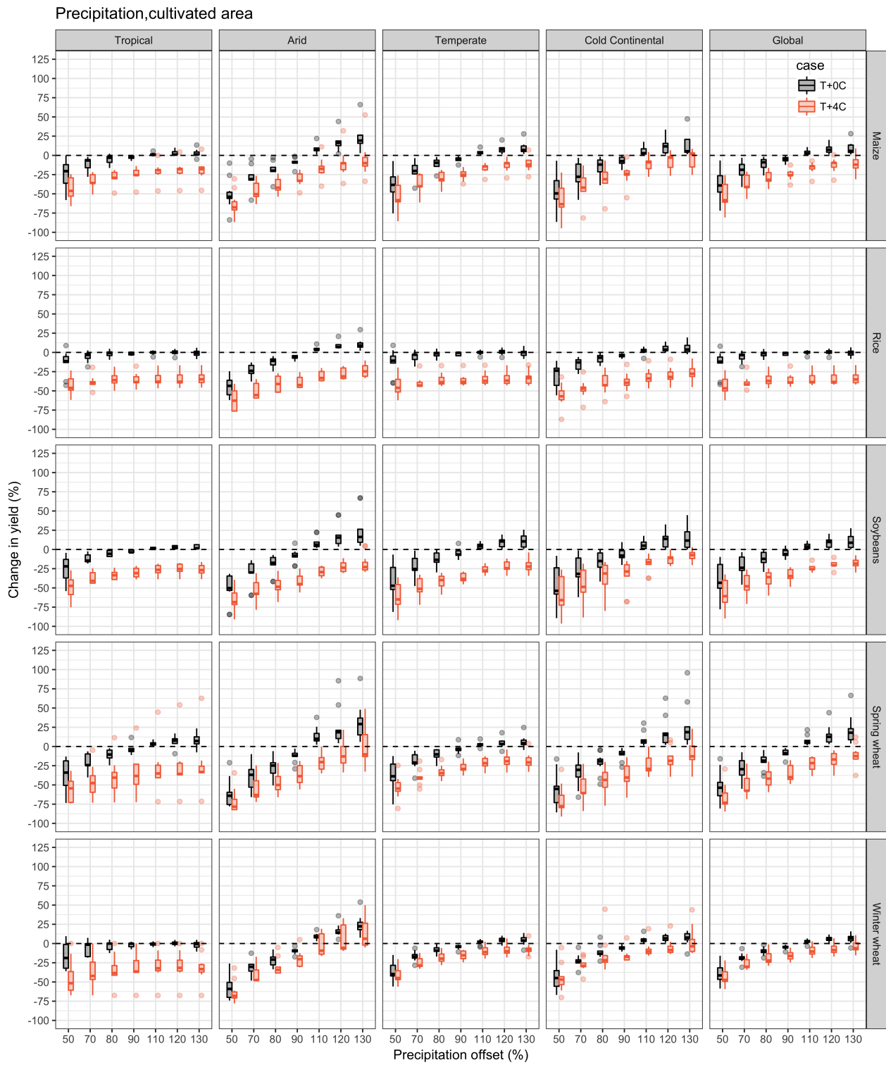
Figure S11: Same as main Figure 5b for all crops. Only over cultivated area.
