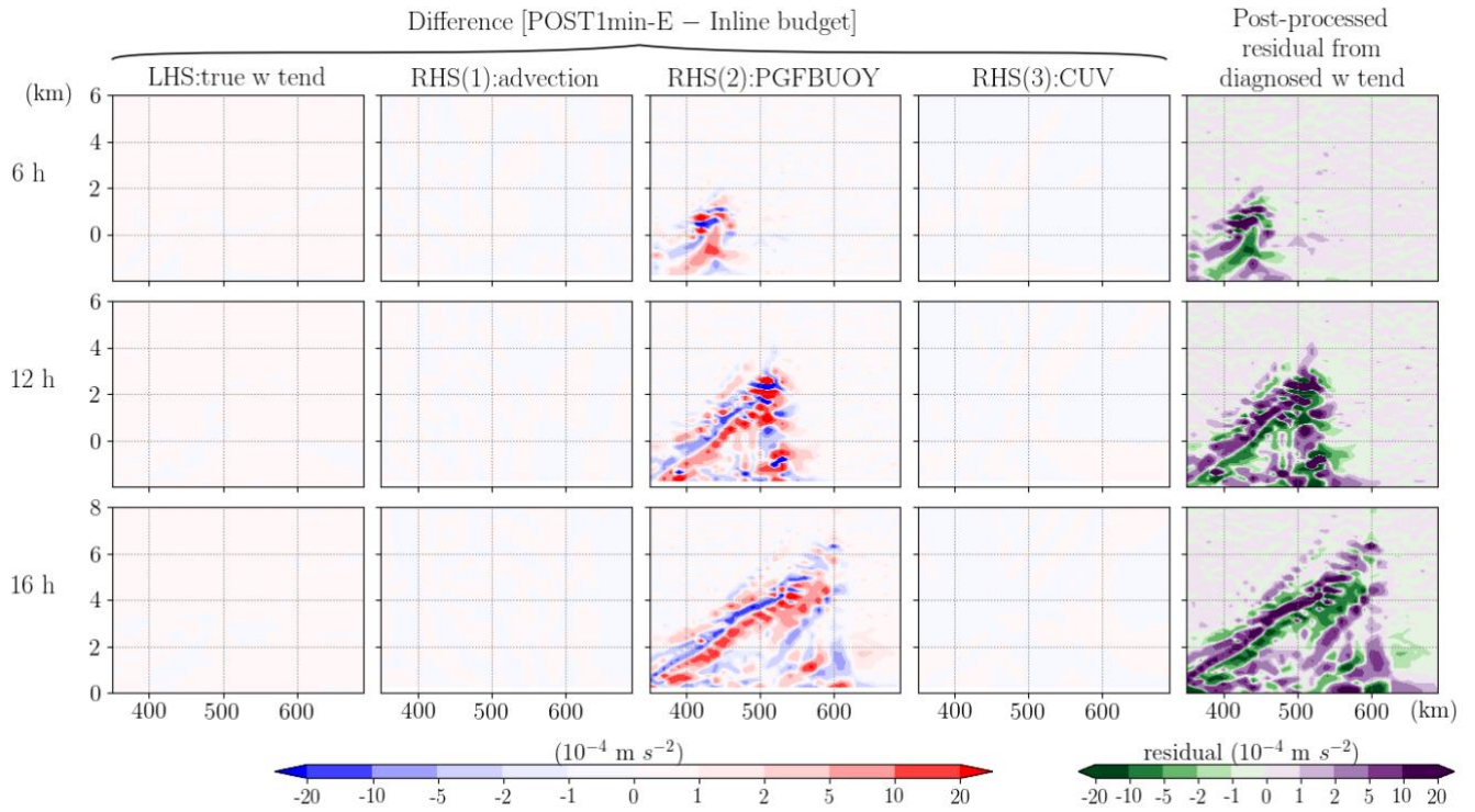
825 Figure 15. The difference between the post-processed (POST1min-E) and the inline budget analysis for vertical momentum W . All terms have been divided by \mu_d and thus have a uniform unit of \text{m s}^{-2} . In each row, the subplots from left to right indicates the difference of true W tendency, ADV, PGFBUOY and CUV. The rightmost subplot indicates the residual term obtained in the post-processed budget analysis. Each row from top to bottom shows the results at 6, 12, and 16 hour, respectively.
