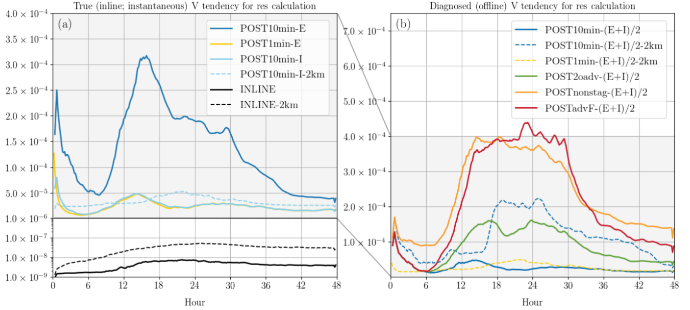
Figure 5. Evolution of the 99th percentile of the residual magnitude ( ms^{-2} ) of the horizontal momentum V budget analysis. For the residual calculation, (a) uses the true V tendency (derived during the integration of the model) and (b) uses the post-diagnosed V tendency (Eq. (8)) as the lhs term. Different colors indicate different post-processed methods for estimating the rhs forcing terms. The residual obtained from the inline budget retrieval are in black. Solid and dashed lines are for the 10-km run and 2-km run, respectively.
