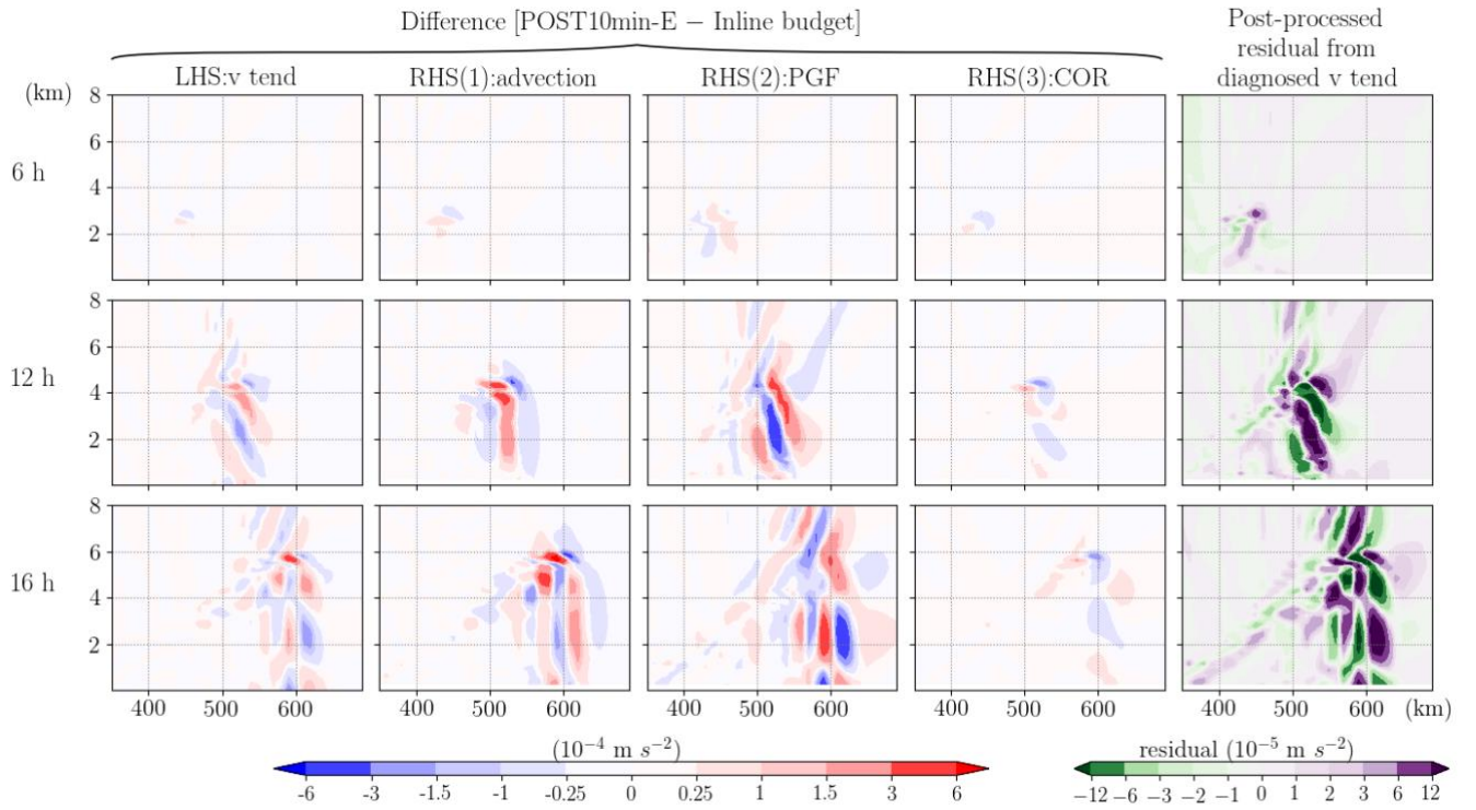
Figure 8. The difference between the post-processed (POST10min-E) and inline budget analysis for the horizontal momentum, \mathbf{V} . All terms have been divided by \mu_d and thus have a uniform unit of \text{ms}^{-2} . In each row, from left to right indicates the difference for \mathbf{V} tendency, ADV, PGF and COR. The rightmost column indicates the residual term obtained in the post-processed budget analysis. Each row from top to bottom shows the results at 6, 12, and 16 hour, respectively.
