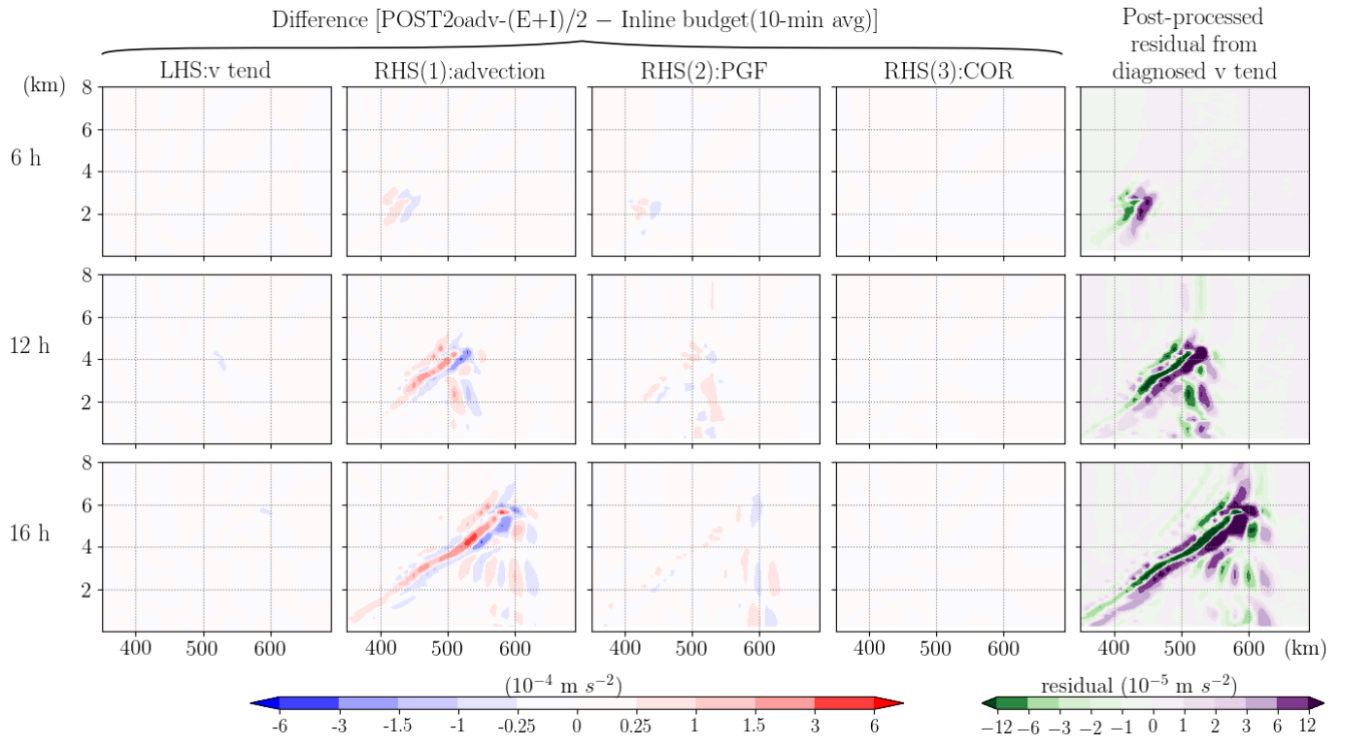
Figure 12. Same as Fig. 11, but the post-processed analysis uses a second order operators for advection calculation ( \text{POST2oadv}-(\mathbf{E}+\mathbf{I})/2 ).
