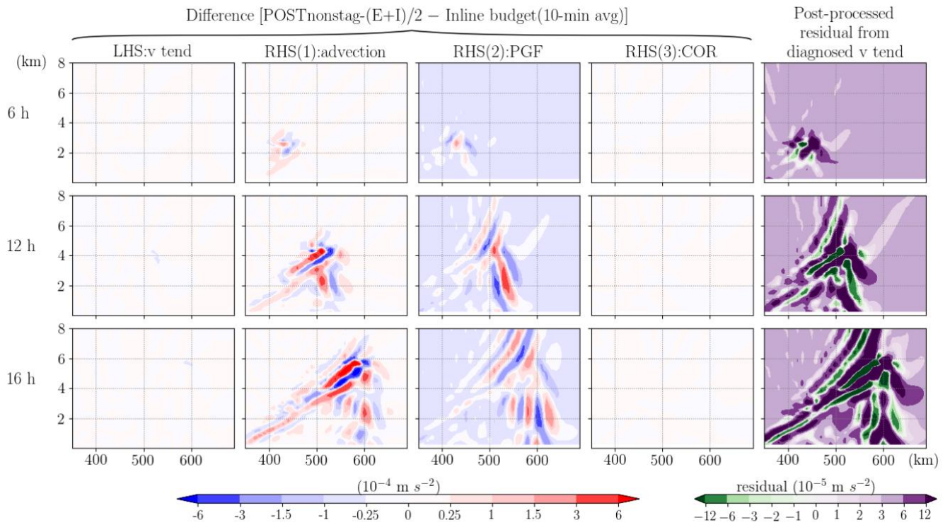
Figure 13. Same as Fig. 11, but for the post-processed analysis does not consider C staggering grids ( \text{POSTnonstag}-(E+I)/2 ).
