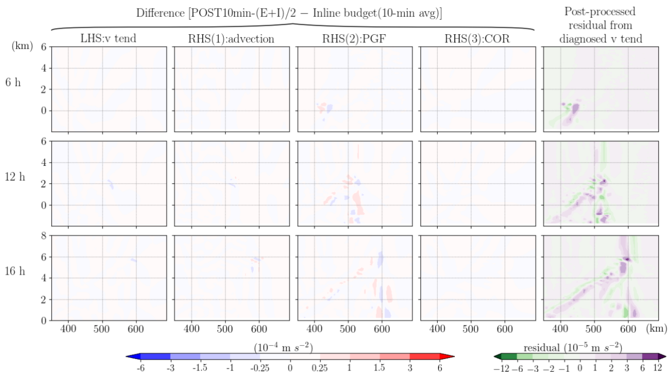
Figure 11. Same as Fig. 8, but the forcing terms diagnosed in the post-processed budget analysis are the average of explicit and implicit methods ( \text{POST10min}-(\text{E}+\text{I})/2 ). To represent the same time window as the post-processed analysis, the inline budget results used here for the difference calculation are the 10-min averages (corresponding to the output interval) instead of the instantaneous values.
