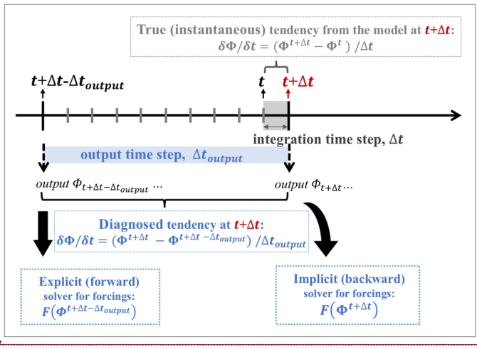
945 Figure 7. Schematic plot showing the explicit (forward) and implicit (backward) solvers for the rhs forcing terms, as well as the diagnosed and the true (calculated inline during the integration of the model) lhs tendency term defined in this study.
