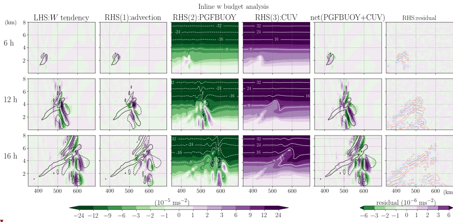
Figure 4. Inline budget analysis of vertical momentum, \overline{w} , with each term extracted directly from the model. In each row, the shading in each subplot from the left to right shows the term of \overline{w} tendency, advection (ADV), net vertical pressure gradient and buoyancy force (PGFBUOY), curvature (CUV) (white contours indicate the values exceeding the color bar), PGFBUOY+ CUV and residual [Eq. (2); P_w is considered but not shown here]. All terms are divided by \mu_4 and thus have units of \text{ms}^{-2} . The black contours indicate the vertical velocity w of 5 and 15 \text{cms}^{-1} (positive and negative values shown in solid and dashed lines, respectively). The red (blue) contours shown in the rightmost column, laid on top of the residual (shading), indicate the small-step components of PGFBUOY with a positive (negative) value of 3 \times 10^{-4} \text{ ms}^{-2} . Each row from top to bottom illustrates the budget analysis at 6, 12, 16 hour, respectively.
