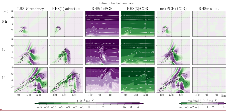
Figure 3. Inline budget analysis of horizontal momentum, \bar{V} , with each term extracted directly from the model. In each row, the shading in each subplot from the left to right shows the term of \bar{V} tendency, flux-form advection (ADV), horizontal pressure gradient force (PGF), Coriolis force (COR) (white contours indicate the values exceeding the color bar), PGF+COR and residual [Eq. (1); P_y is zero and the generally small curvature term (CUV) is not shown]. All terms are divided by \mu_d and thus have units of \text{ms}^{-2} . The black contours indicate the horizontal velocity v of 2 and 6 \text{ ms}^{-1} (positive and negative values shown in solid and dashed lines, respectively). Each row from top to bottom illustrates the budget analysis at 6, 12, 16 hour, respectively.
