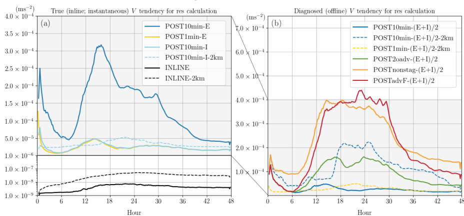
Figure 5. Evolution of the 99th percentile of the residual magnitude ( \text{ms}^{-2} ) of the horizontal momentum V budget analysis. For the residual calculation, (a) uses the true V tendency (derived during the integration of the model) and (b) uses the post-diagnosed V tendency (Eq. (8)) as the lhs term. Different colors indicate different post-processed methods for estimating the rhs forcing terms. The residual obtained from the inline budget retrieval are in black. Solid and dashed lines are for the 10-km run and 2-km run, respectively.
