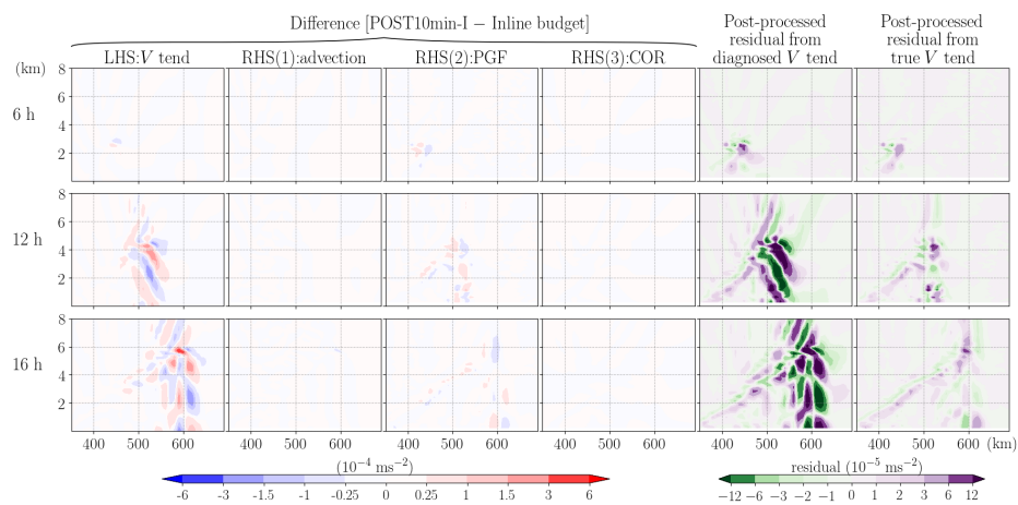
Figure 10. Same as Fig. 8, but the post-processed rhs terms are diagnosed using the implicit/backward method (POST10min-I) and an extra column is added on the rightmost showing the residual from the true tendency (i.e., the instantaneous value obtained from the model).
