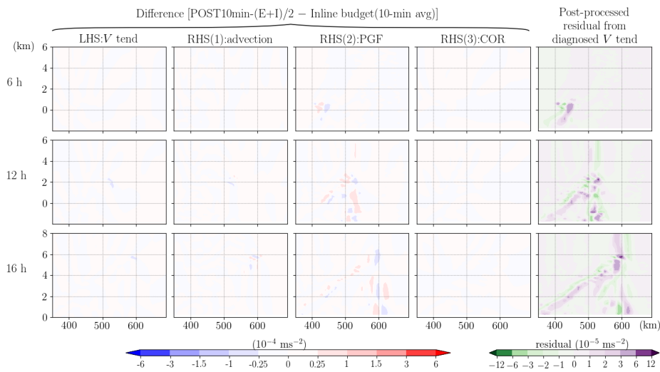
Figure 11. Same as Fig. 8, but the forcing terms diagnosed in the post-processed budget analysis are the averages of explicit and implicit methods (POST10min-(E+I)/2). To represent the same time window as the post-processed analysis, the inline budget results used here for the difference calculation are the 10-min averages (corresponding to the output interval) instead of the instantaneous values.
