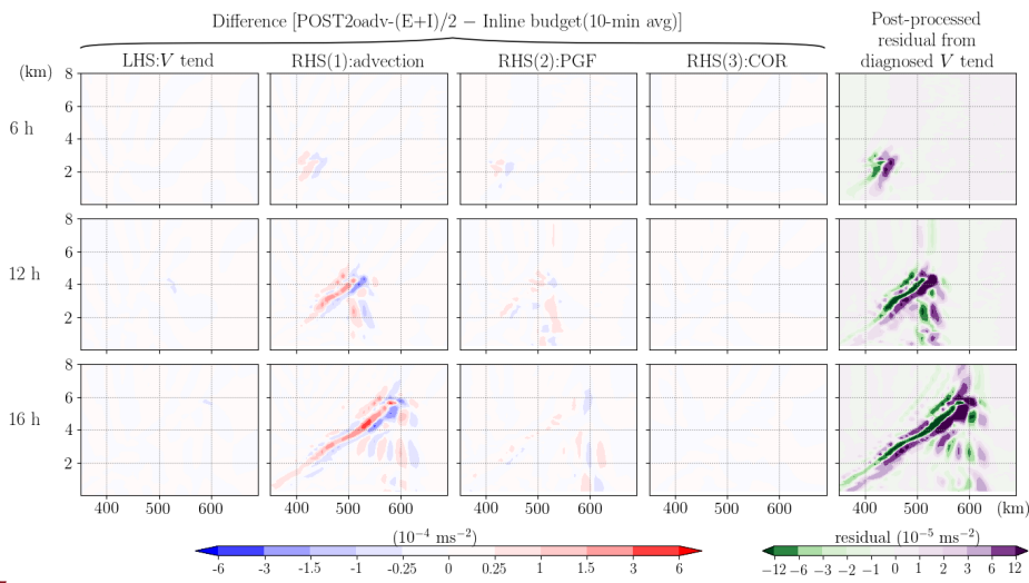
980 Figure 12. Same as Fig. 11, but the post-processed analysis uses a second_order operator for advection calculation (POST2oadv-(E+I)/2).
