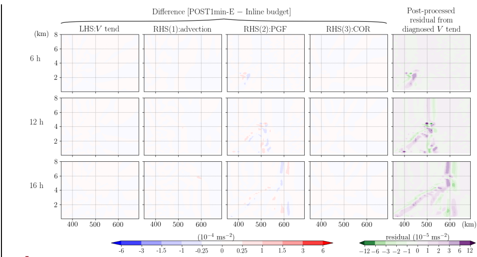
960 Figure 9. Same as Fig. 8, but the post-processed budget analysis is applied on the data with an output time interval of 1 minute (POST1min-E).
