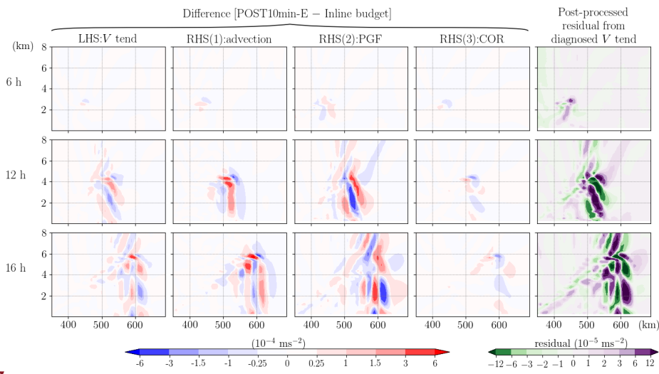
950 Figure 8. The difference between the post-processed (POST10min-E; with an explicit/forward method on 10-min output ) and inline budget analysis for the horizontal momentum, \mathbf{V} . All terms have been divided by \mu_d and thus have a uniform unit of \text{ms}^{-2} . In each row, from left to right indicates the difference for \mathbf{V} tendency, ADV, PGF and COR. The rightmost column indicates the residual term obtained in the post-processed budget analysis. Each row from top to bottom shows the results at 6, 12, and 16 hour, respectively.
