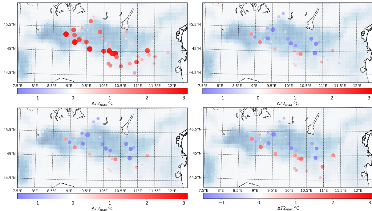
Figure 6. Monthly average for daily maximum 2-meter temperature difference between model run LR2 and the weather stations' location for the control run (top left), CHANNEL (Opt.1, top right), DRIP (Opt.2, bottom left) and SPRINKLER (Opt.3, bottom right)
