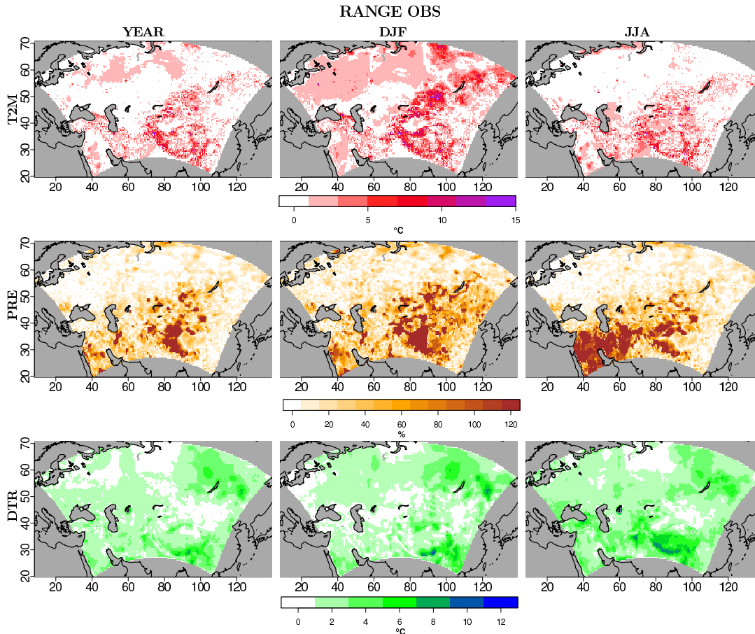
Fig. 4. Maps of the spread calculated among different observational datasets for each considered variable, for the annual mean (left), winter (middle) mean and summer mean (right). From top to bottom, the va
