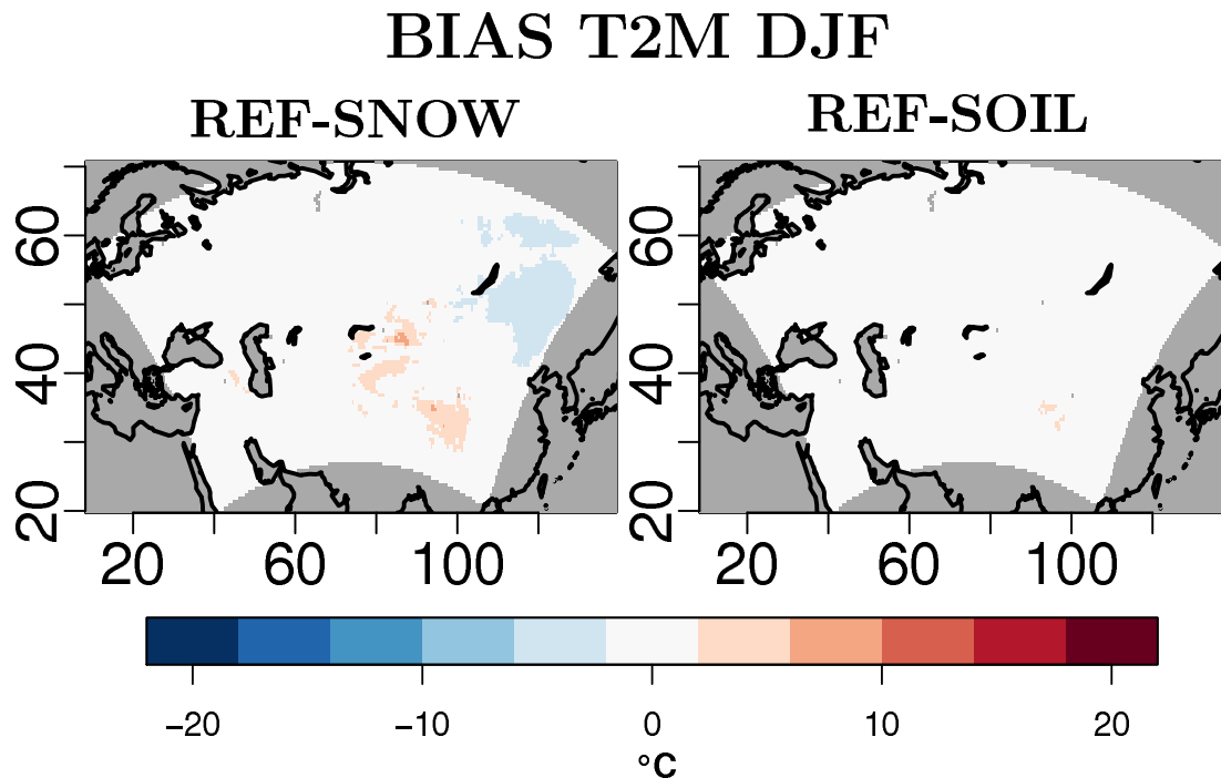
Fig. 2. Mean bias of near surface temperature (T2M, \text{°C} ) winter values of the reference simulation \text{\textbf{a}} and the simulation \text{\textbf{SNOW}} ( \text{\textit{left}} ) and \text{\textbf{SOIL}} ( \text{\textit{right}} ),
