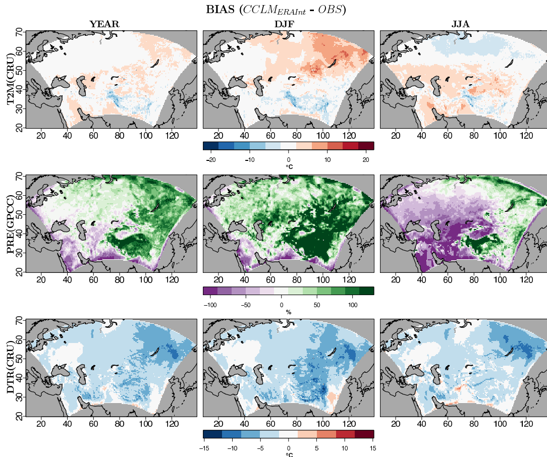
Fig. 1. Mean bias of annual mean (left), winter mean (middle) and summer mean (right) near surface temperature (T2M, °C, top panel), precipitation (PRE, %, middle panel) and diurnal temperature range (D
