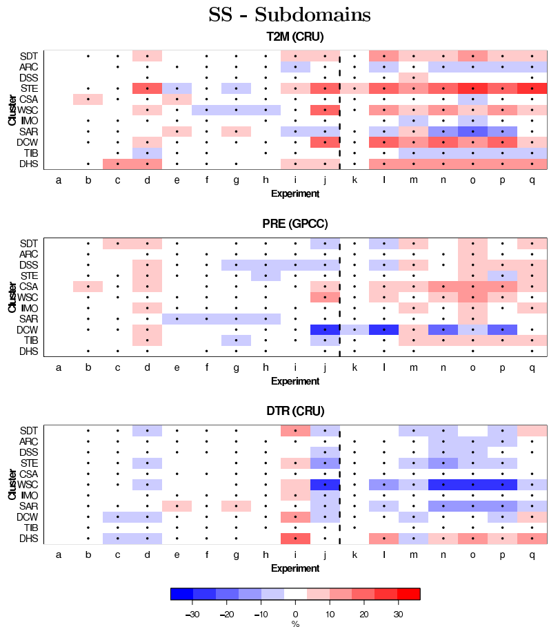
Fig. 8. Skill Score (SS) derived from the MAE calculated for each domain sub-region over the monthly climatological values of the seasonal cycle of different COSMO-CLM simulations and observational datasets.
