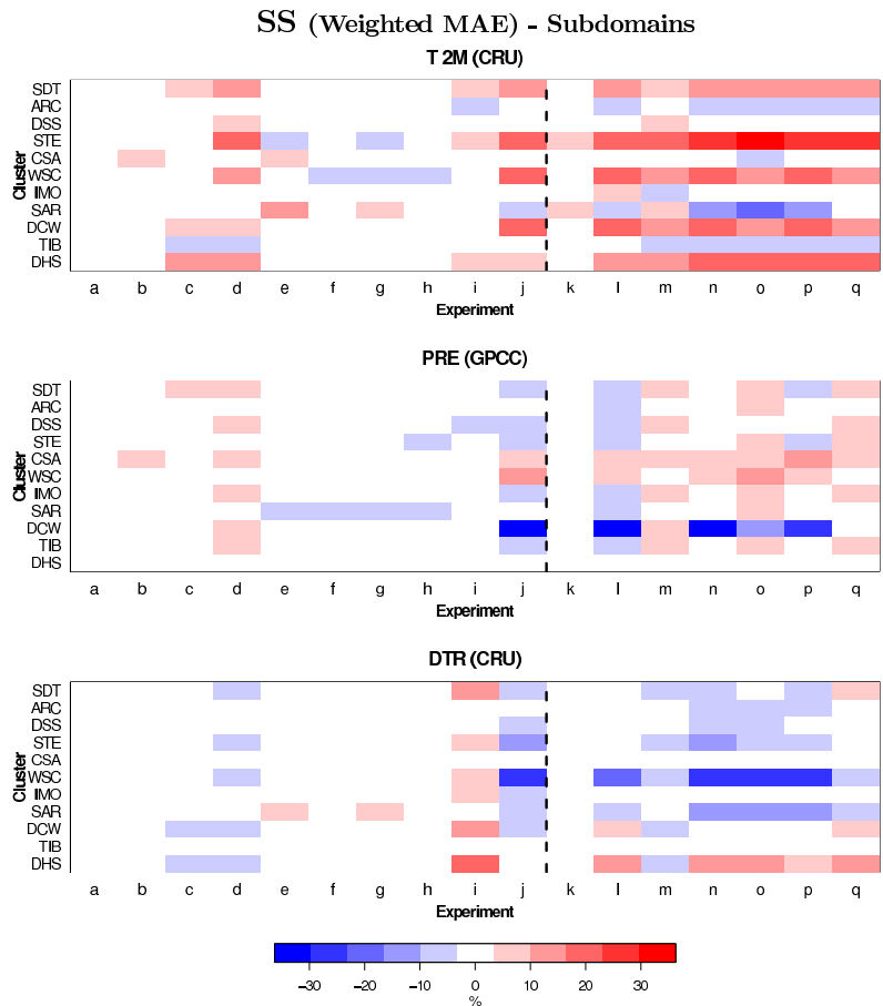
Fig. 10. Skill Score (SS) derived from the weighted MAE ( \$MAE_w\$, Eq. \ref{eqq} ) calculated for each domain sub-region over the monthly climatological values of the seasonal cycle of different COSMO-CLM simula
