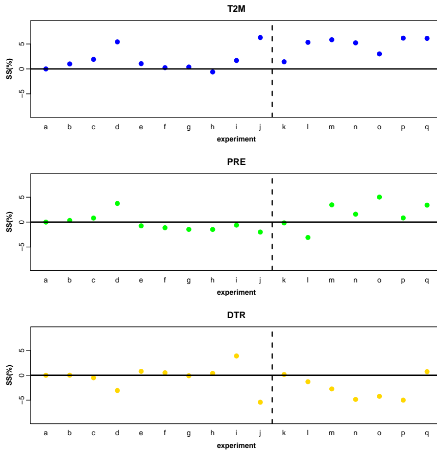
Fig. 7. Skill Score (SS) derived from the weighted MAE ( MAE_w , Eq. \ref{eqa}) calculated over the monthly climatological values of the seasonal cycle of different COSMO-CLM simulations and observational da
