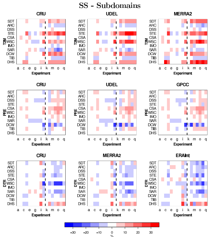
Fig. 9. Skill Score (SS) derived from the MAE calculated for each domain sub-region over the monthly climatological values of the seasonal cycle of different COSMO-CLM simulations and observational datasets.
