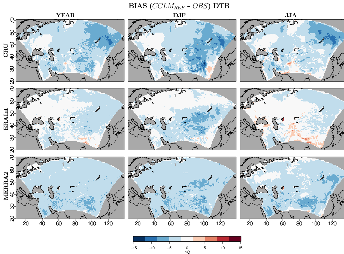
Fig. 6. Mean bias of annual mean ( \textit{left} ), winter mean ( \textit{middle} ) and summer mean ( \textit{right} ) Diurnal Temperature Range (DTR, \textit{degree C} ), of the reference COSMO-CLM simulation (a) with
