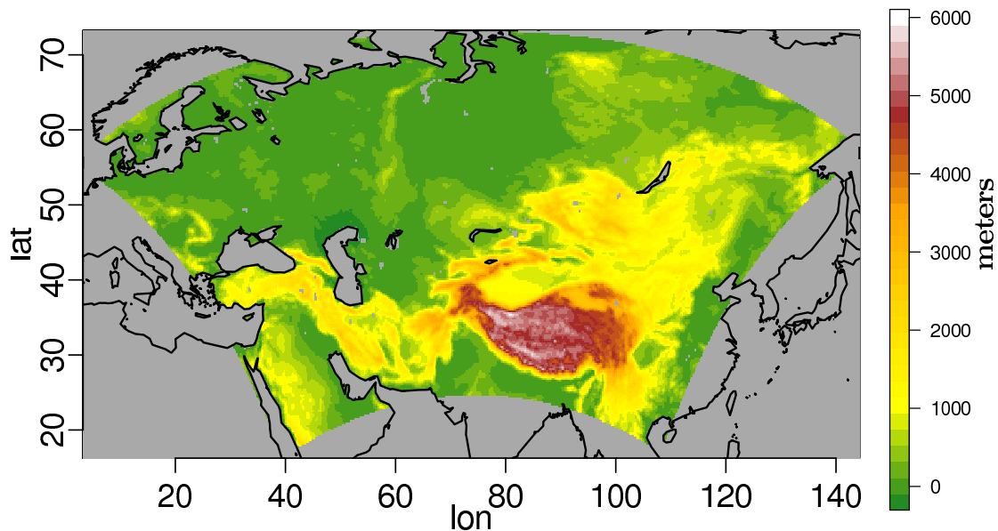
Fig. 11. Orography map of the Central Asia simulation domain on a regular grid with a spatial resolution of 0.25 km. Masked in gray are the ocean and the external area of the domain.
