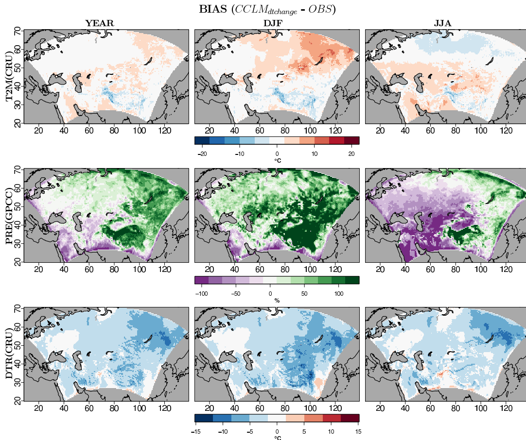
Fig. 3. Maps of bias calculated for the NCEP2-driven simulation with the reference configuration but different time step, against different observational datasets for the 3 considered variables. Every row pre
