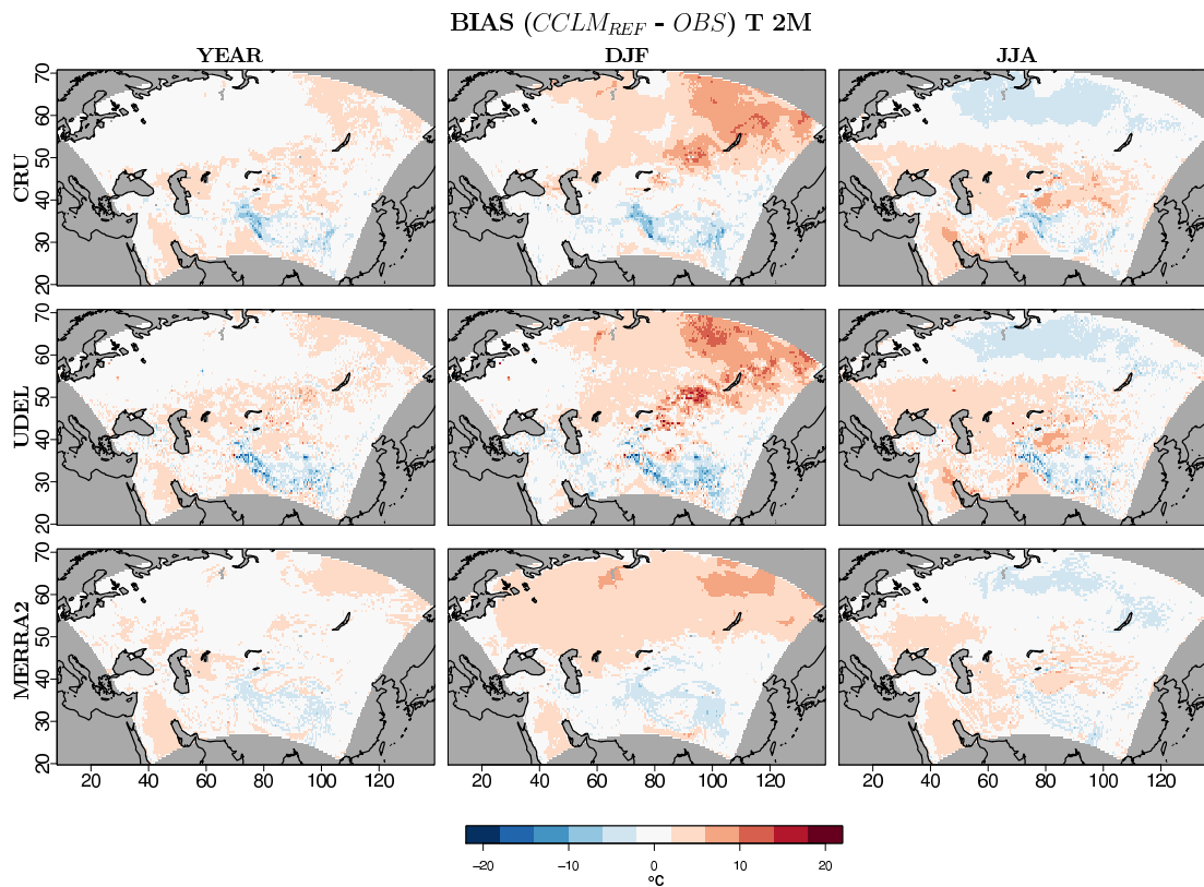
Fig. 5. Mean bias of annual mean ( \text{left} ), winter mean ( \text{middle} ) and summer mean ( \text{right} ) near surface temperature (T2M, \text{degree C} ), of the reference COSMO-CLM simulation (a) with r
