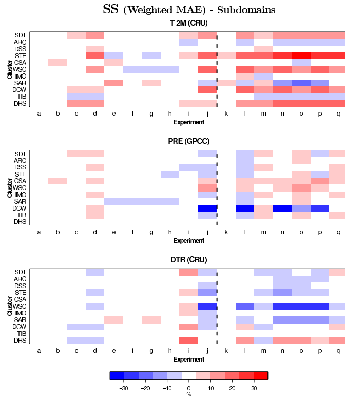
Fig. 10. Skill Score (SS) derived from the weighted MAE ( MAE_w , Eq. \ref{eqa}) calculated for each domain sub-region over the monthly climatological values of the seasonal cycle of different COSMO-CLM simula
