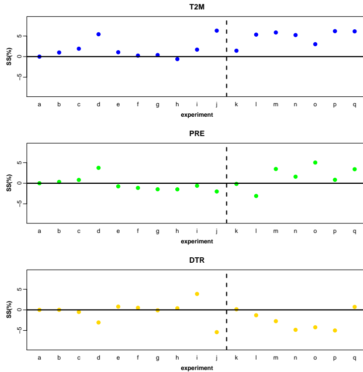
Fig. 7. Skill Score (SS) derived from the weighted MAE ( MAE_w , Eq. \ref{eqa}) calculated over the monthly climatological values of the seasonal cycle of different COSMO-CLM simulations and observational da
