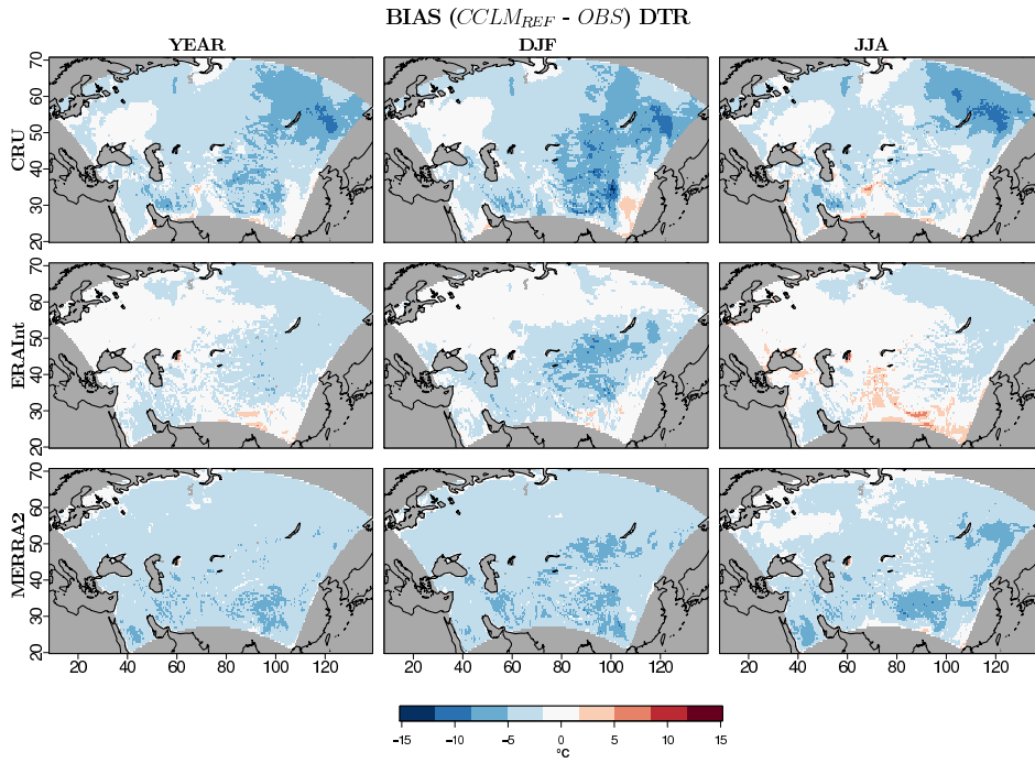
Fig. 6. Mean bias of annual mean (left), winter mean (middle) and summer mean (right) Diurnal Temperature Range (DTR, ^{\circ}\text{C} ), of the reference COSMO-CLM simulation (a) with
