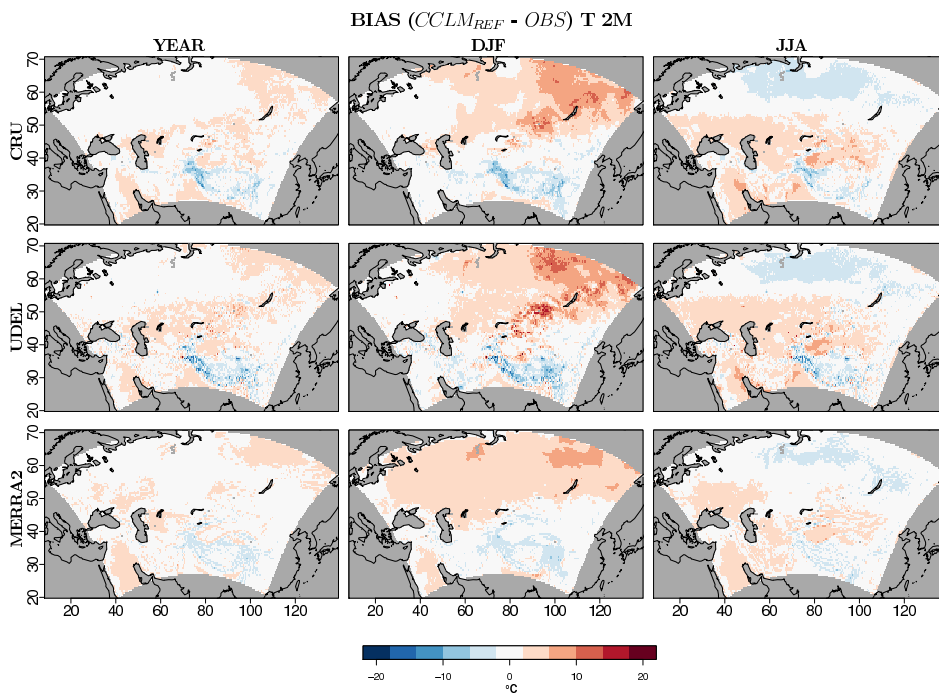
Fig. 5. Mean bias of annual mean (left), winter mean (middle) and summer mean (right) near surface temperature (T2M, °C), of the reference COSMO-CLM simulation (a) with r
