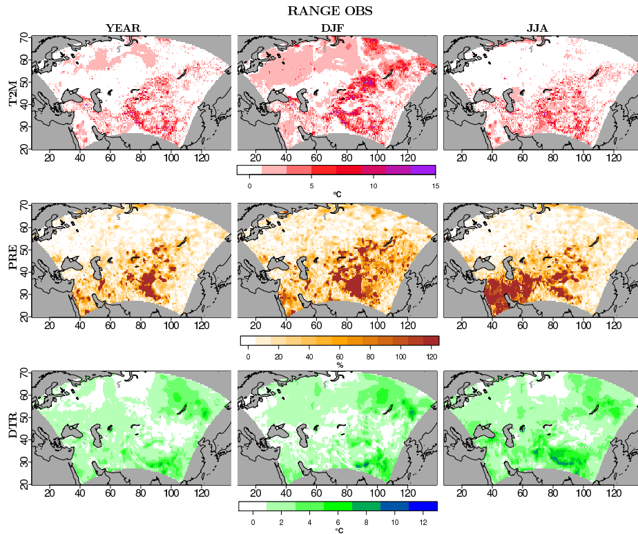
Fig. 4. Maps of the spread calculated among different observational datasets for each considered variable, for the annual mean (left), winter (middle) mean and summer mean (right). From top to bottom, the va
