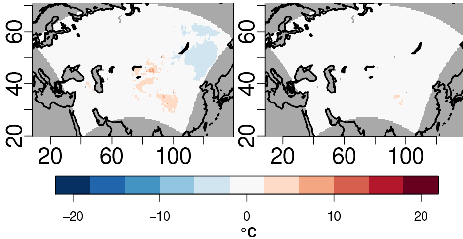
Fig. 2. Mean bias of near surface temperature (T2M, \text{^\circ C} ) winter values of the reference simulation \text{\textbf{a}} and the simulation \text{\textbf{SNOW}} ( \text{\textit{left}} ) and \text{\textbf{SOIL}} ( \text{\textit{right}} ),
