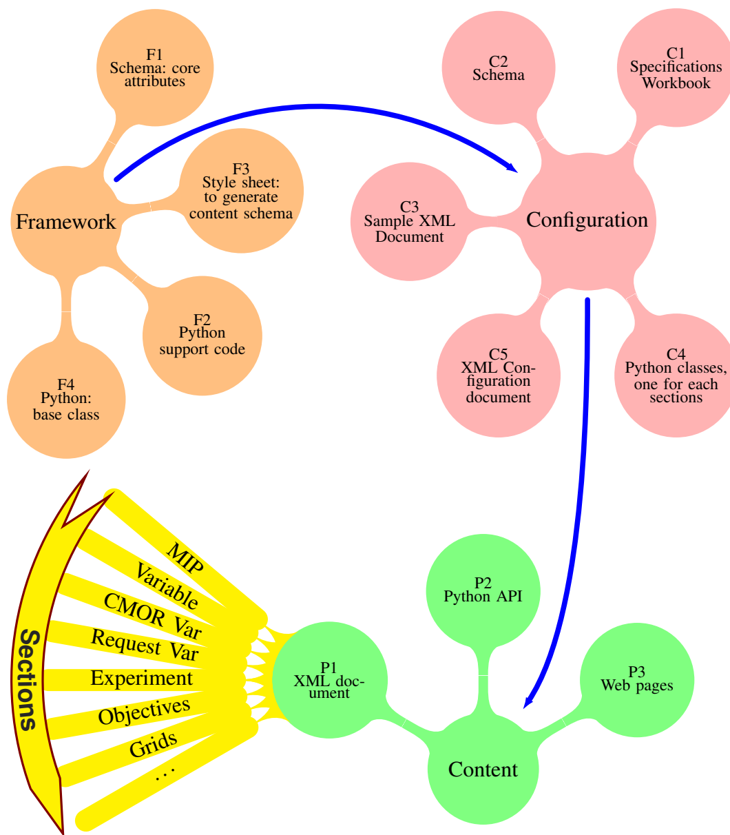
Figure 2. A core framework is explicitly coded into a python base class. The "Configuration" section is information such as the fact that the CMOR variables carry a coords attribute that can specify additional coordinate variables needed for a data variable. The "Content" data includes the specific names of the coordinate variables for each data variable.
