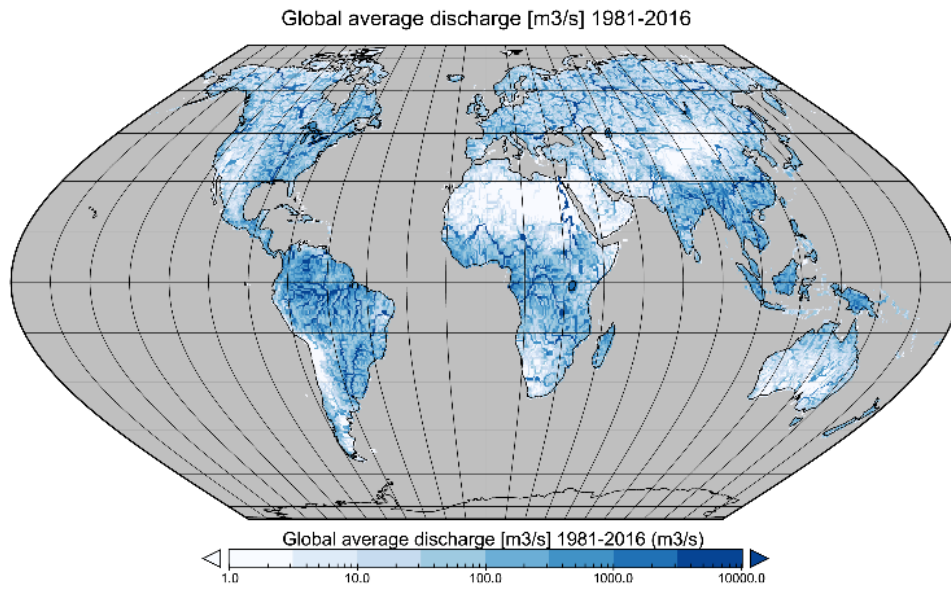
635 Figure 2: Average global discharge in m 3 /s (1979-2016)
