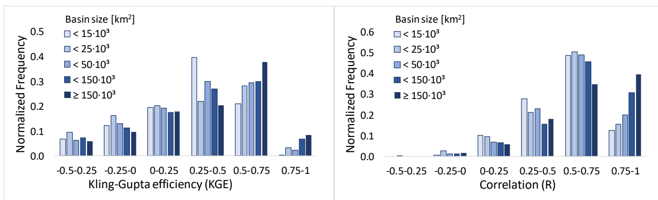
Figure 4: Histograms of Kling-Gupta-efficiency and correlation for different basin size based on 1366 GRDC stations
