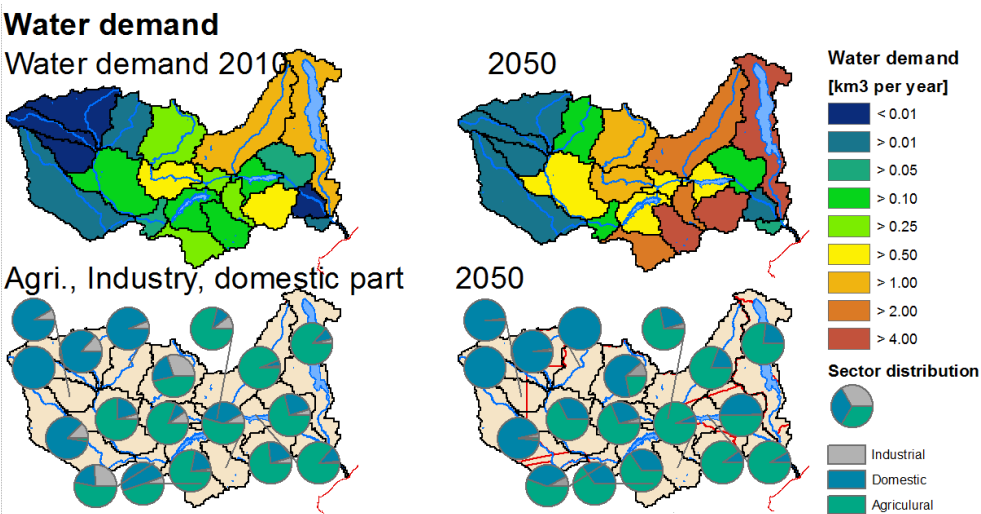
Figure 1314: Water demand projection for scenario SSP2/RCP6.0 to 2050 based on population, GDP, irrigation area projections
