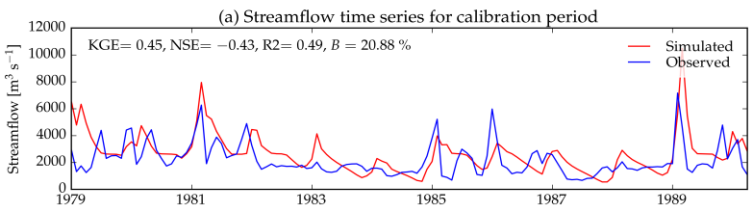
Figure 97: Calibration results for two stations in the Zambezi basin
