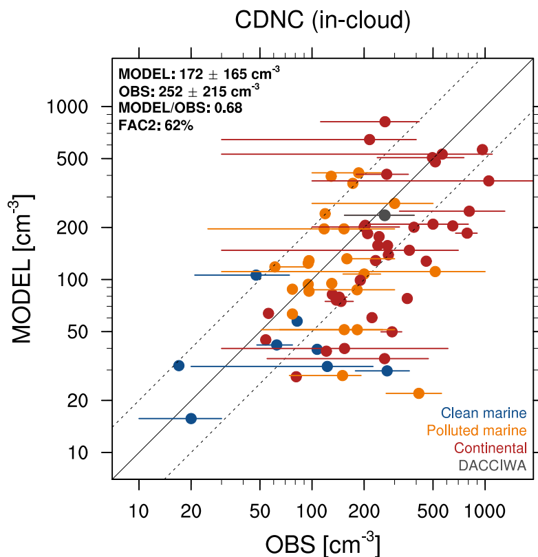
Figure S1. As in Fig. 3 in the paper, but using a different method for calculating supersaturation in liquid clouds. See Sect. 4.3 in the paper for details.
