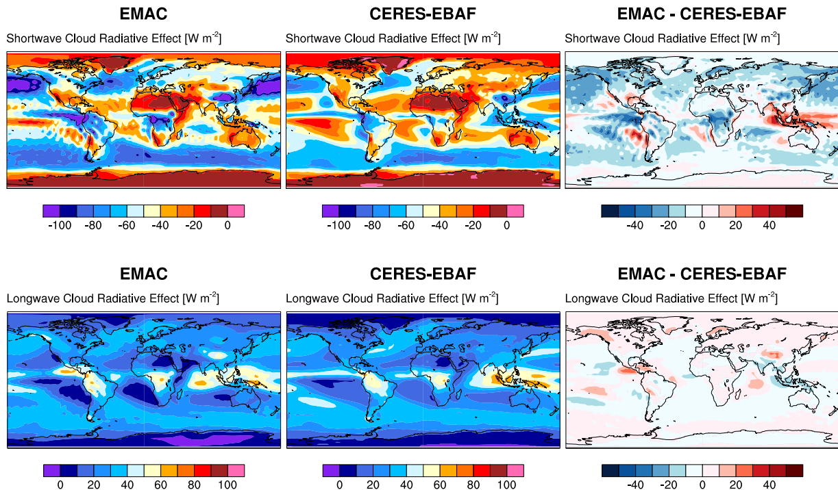
Figure 8. Similar to Fig. 2 but for radiation variables: shortwave (top) and longwave cloud radiative effects (bottom). Satellite data are averaged over the 2003-2015 time period.
