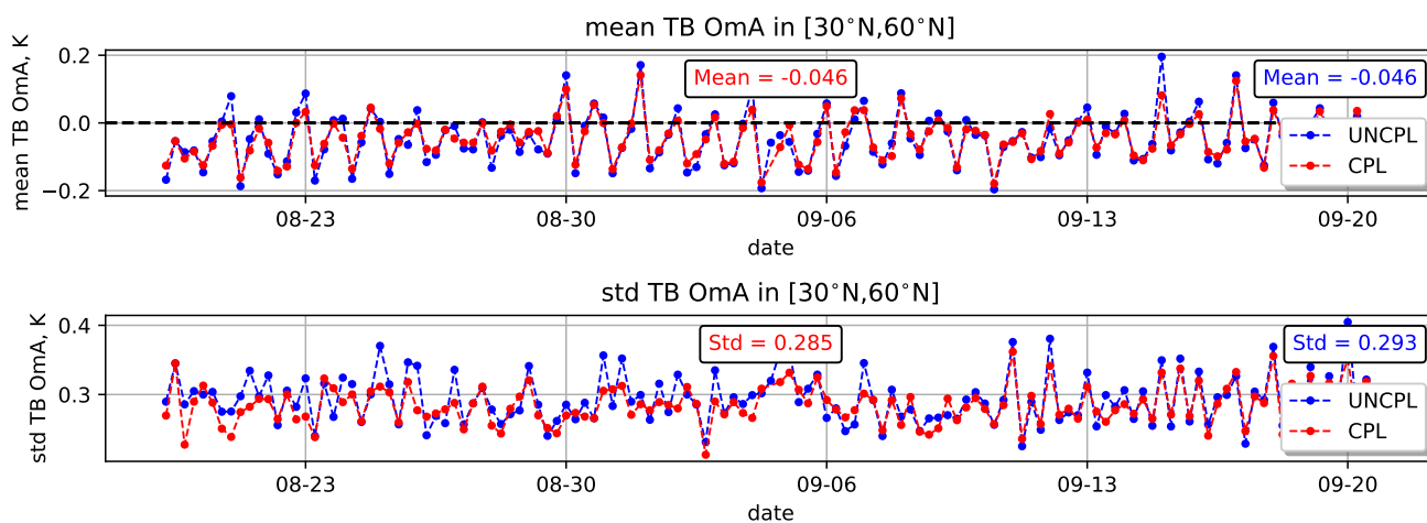
Figure 4. (a) Observation-minus-Analysis (OmA) statistics: bias (top) and standard deviation (bottom) using 6 h forecasts, statistics. Bias and standard deviation for the brightness temperature, in K, as seen by the AQUA AIRS Channel 950. The statistics are computed for UNCPL (blue) and CPL (red) in the Northern Extratropics region [30°N, 60°N].
