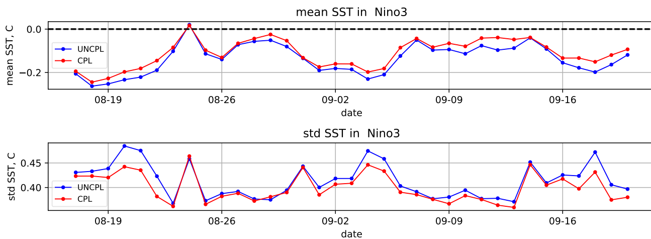
Figure 11. Bias (top) and standard deviation (bottom) with respect to the gridded foundation SST field from the ocean SAM2 DA component for the "Nino3" region situated within the latitude-longitude box defined by [150°W, 90°W] and [5°S, 5°N]. The statistics are computed using 24-h forecasts.
