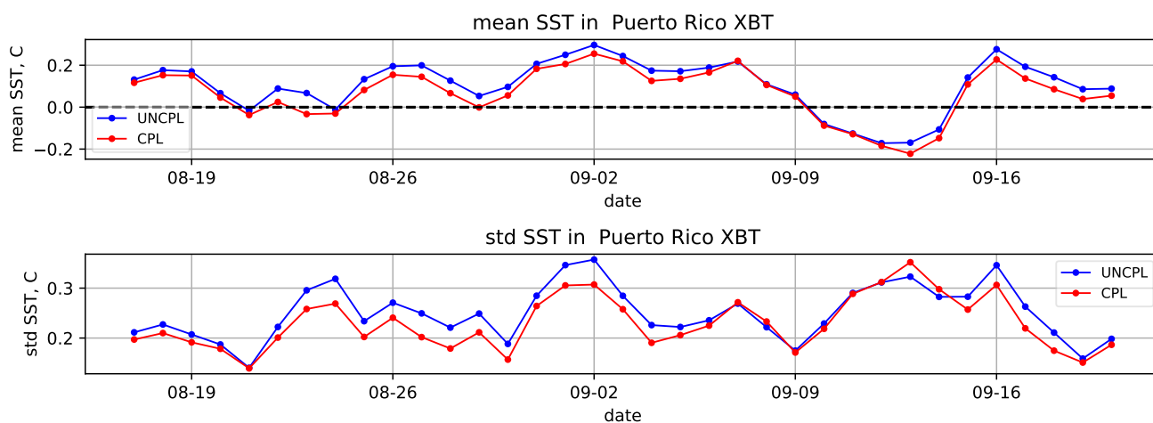
Figure 10. Bias (top) and standard deviation (bottom) with respect to the gridded foundation SST field from the ocean SAM2 DA component for the "Puerto Rico XBT" region situated within the latitude-longitude box defined by [35°W, 65°W] and [25°N, 35°N]. The statistics are computed using 24-h forecasts.
