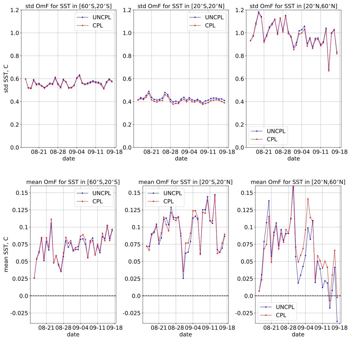
Figure 8. Evolution of sea surface temperature OmF standard deviation (top row) and bias (bottom row), in degrees C, with respect to SST data assimilated within the separate SST DA component. The statistics are computed for UNCPL (blue curves) and CPL (red curves) in three latitude bands: Southern Extratropics [20°S, 60°S] (left), Tropics [20°S, 20°N] (middle) and Northern Extratropics [20°N, 60°N] (right). The statistics are computed for the 12 h forecast and the corresponding data.
