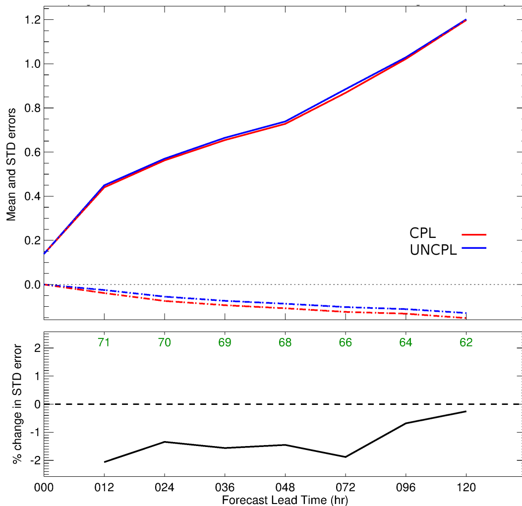
Figure 7. Top panel: standard deviation (solid curves) and bias (dashed curves) growth, in degrees C, as a function of forecast lead time for the air temperature at 1000 hPa. The statistics are computed for the CPL (red) and UNCPL (blue) against mean analysis in the Northern Extratropics region [20°N, 60°N]. Bottom panel: the change in the standard deviation error in % between CPL and UNCPL. The green numbers show the number of samples used to compute the statistics.
