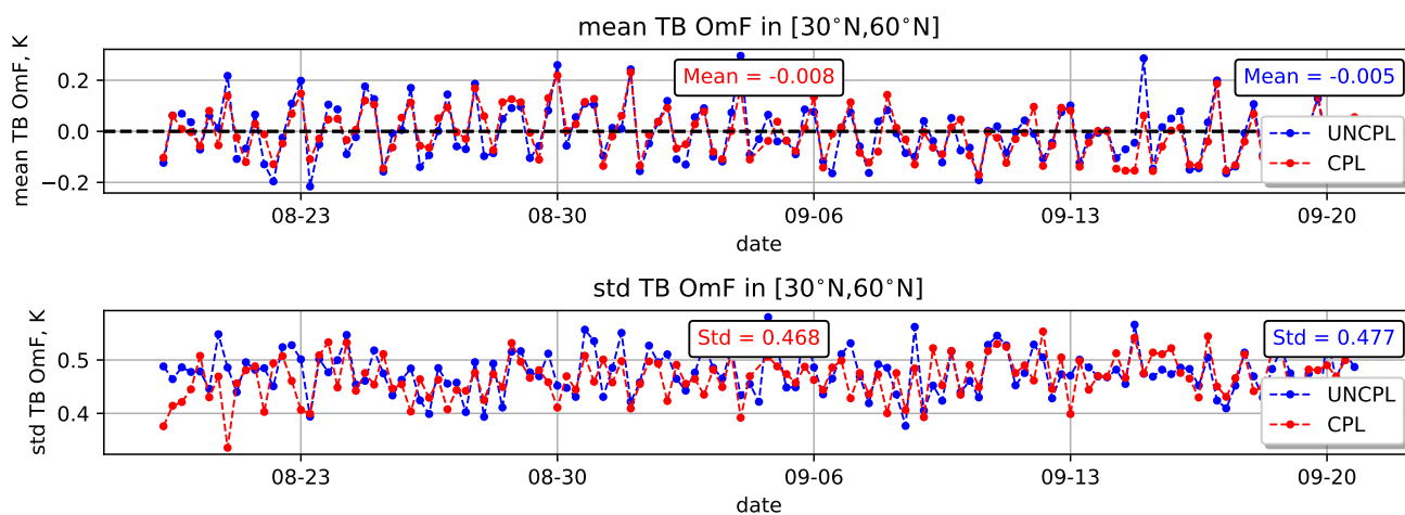
Figure 5. Observation-minus-Forecast (OmF) statistics: bias (top) and standard deviation (bottom) using 6 h forecasts, statistics. Bias and standard deviation for the brightness temperature, in K, as seen by the AQUA AIRS Channel 950. The statistics are computed for UNCPL (blue) and CPL (red) in the Northern Extratropics region [30°N, 60°N].
