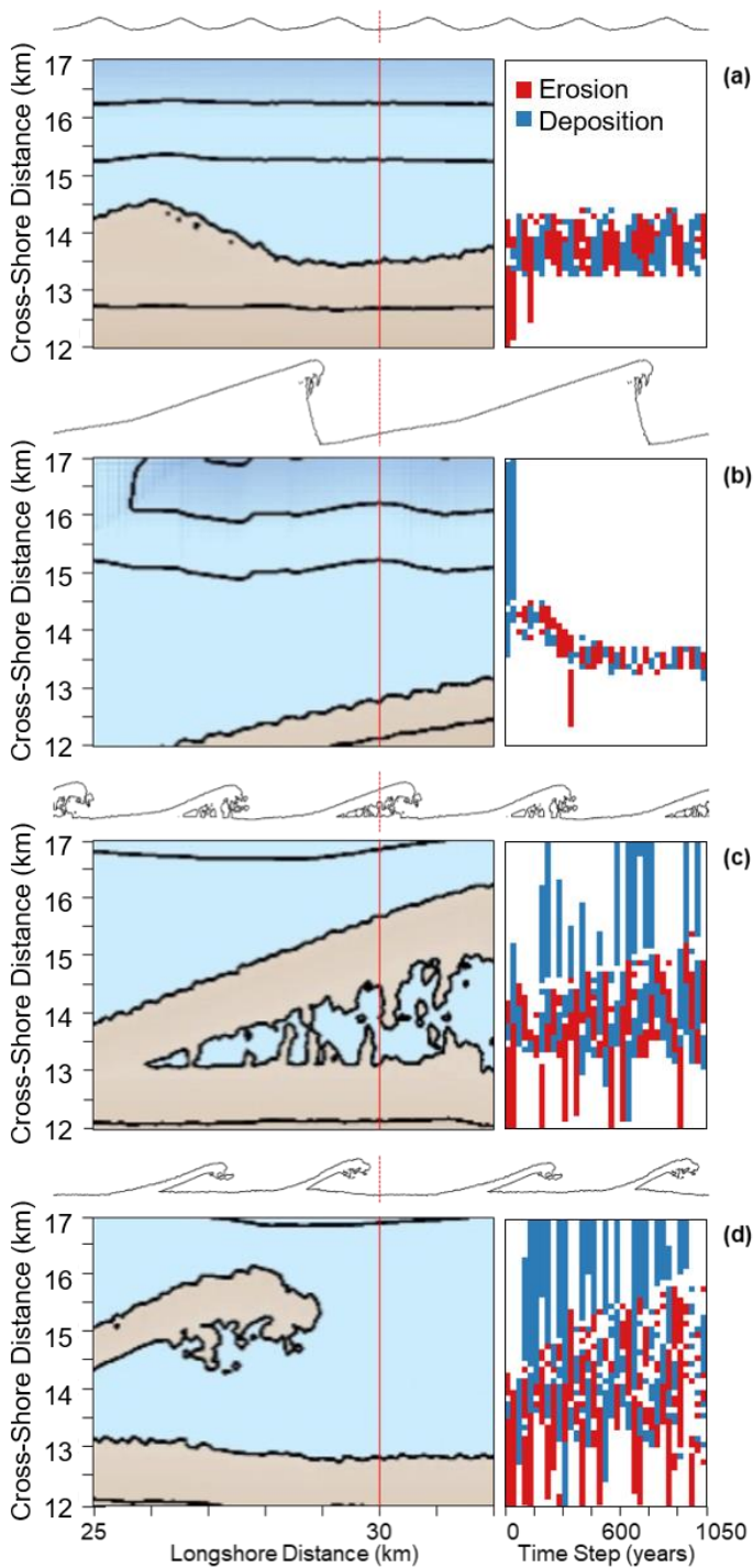
655 Figure 15: Shoreline Morphologies (left) and volume stacks (right) for four simulations where the wave climate is defined by (a) A = 0.5 , U = 0.55 , (b) A = 0.6 , U = 0.6 , (c) A = 0.7 , U = 0.65 and (d) A = 0.8 , U = 0.7 . The red line marks the cross-shore transect where the change in volume at 30 year time intervals is recorded.
