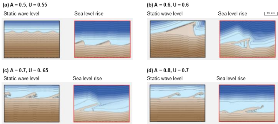
670 Figure 18: Coastal morphologies for four simulations where the wave climate is defined by (a) A = 0.5, U = 0.55 , (b) A = 0.6, U = 0.6 , (c) A = 0.7, U = 0.65 and (d) A = 0.8, U = 0.7 , run with two water level scenarios including a static water level (left, black outline) and a rising sea level at a rate of 2 m / 100 years (right, red outline).
