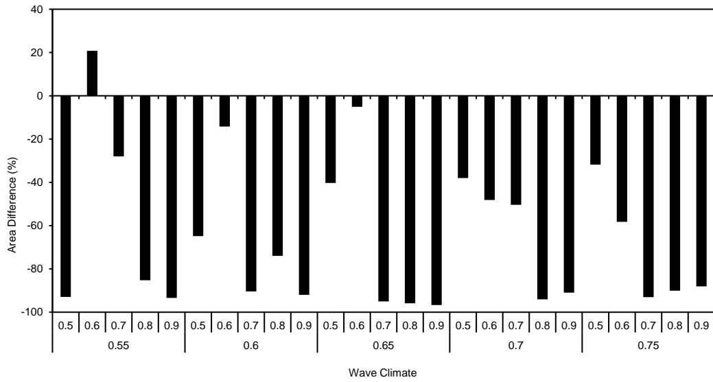
Figure 12: Areal difference (%) between results of CEM2D to CEM. The wave climate given along the x-axis is defined according to the wave asymmetry (top row) and the proportion of high angle waves (bottom row).
