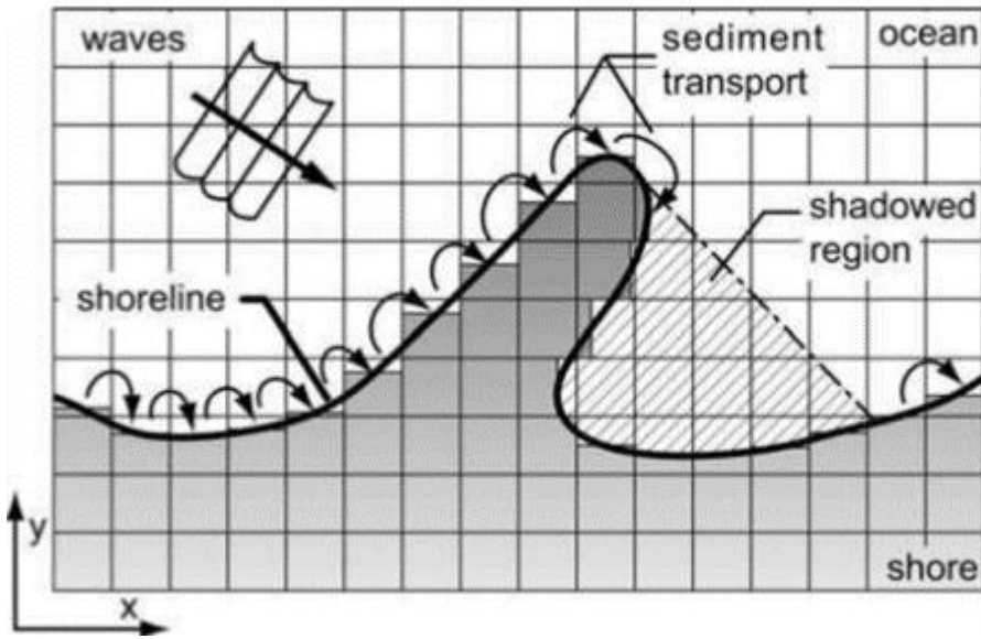
600 Figure 3: Plan-view schematic of CEM showing the shadow zone that is formed when protruding sections of coastline prevent waves from approaching the shoreline (Ashton and Murray, 2006a).
