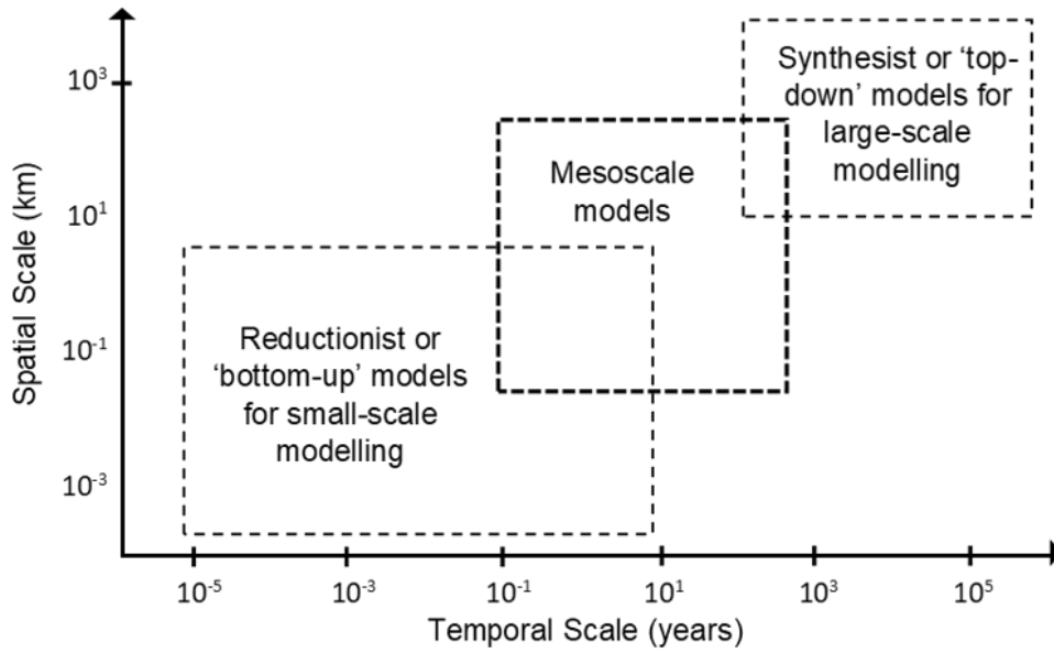
590 Figure 1: Spatial and temporal ranges for traditionally reductionist and synthesist models, with mesoscale models highlighted in grey within the scale appropriate for coastal management (adapted from Gelfenbaum and Kaminsky, 2010; van Maanen et al., 2016).
