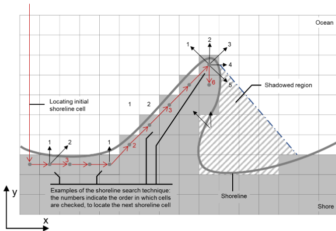
610 Figure 5: A schematic of the shoreline search technique used in CEM (and CEM2D) to map the X and Y location of the shoreline cells. The number in square brackets denotes the shoreline cell number that is associated with a particular X and Y value and the number on each arrow is the iteration of the clockwise search from the shoreline cell where it originates.
