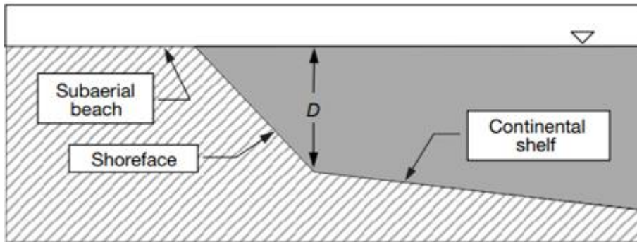
595 Figure 2: Cross-sectional profile of CEM showing the location of the depth of closure, where the shoreface slope intersects the continental shelf slope (after Ashton et al., 2001).
