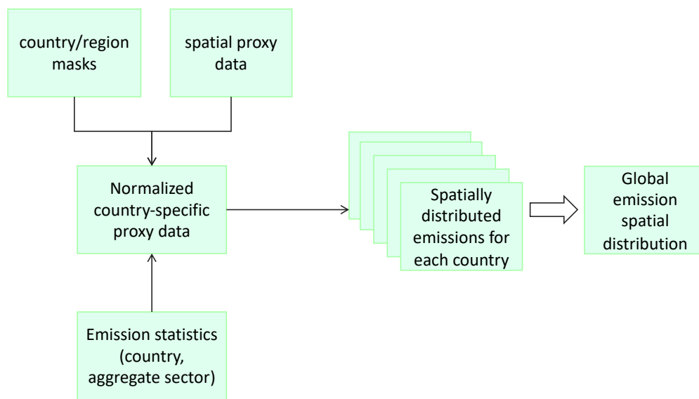
Figure 1: Emissions gridding overview. Emissions data at the level of country and aggregate sector are mapped to spatial grids separately by country and sector, and then combined into global emissions grids as described in the main text.
