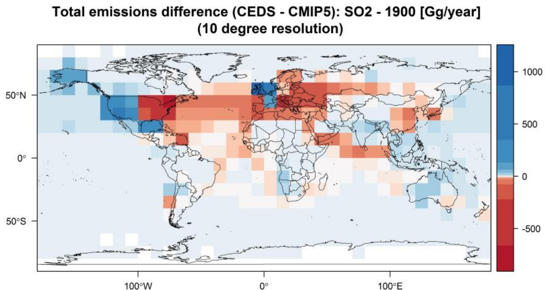
10 Figure 11 – Difference in CMIP6 (e.g. CEDS) and CMIP5 gridded total SO 2 emissions in 1900. For like with like comparison, these figures do not include aviation, or agricultural waste burning on fields.
