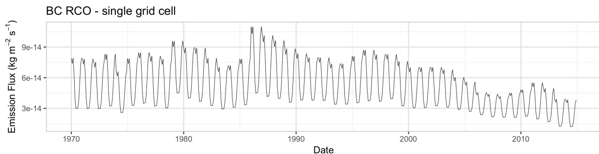
5 Figure 10 – Time series plot for total BC emissions over time at the monthly level for a grid cell in Finland.
