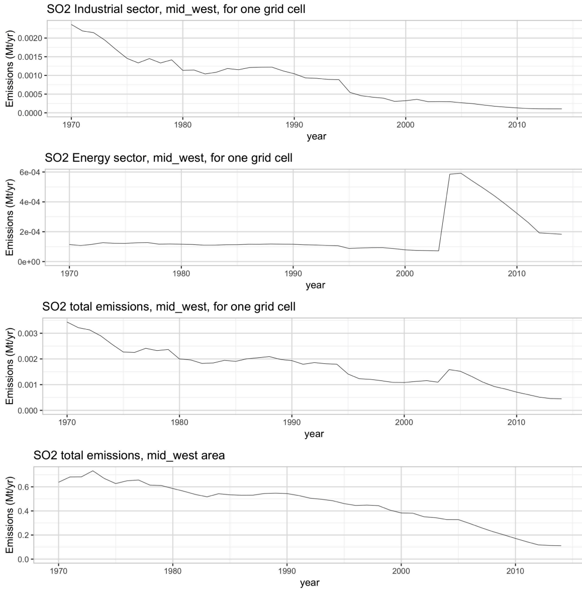
Figure 8 – a) Time series plot for the industrial gridding sector for a single 0.5 degree cell on the US mid west (lat, lon: 41.25, -87.75). b) Time series plot for the Energy sector for the same grid cell. c) Time series plot for total anthropogenic emissions for the same grid cell. d) Time series plot for total anthropogenic emissions summed over 16 grid cells including the cell depicted in a-c.
