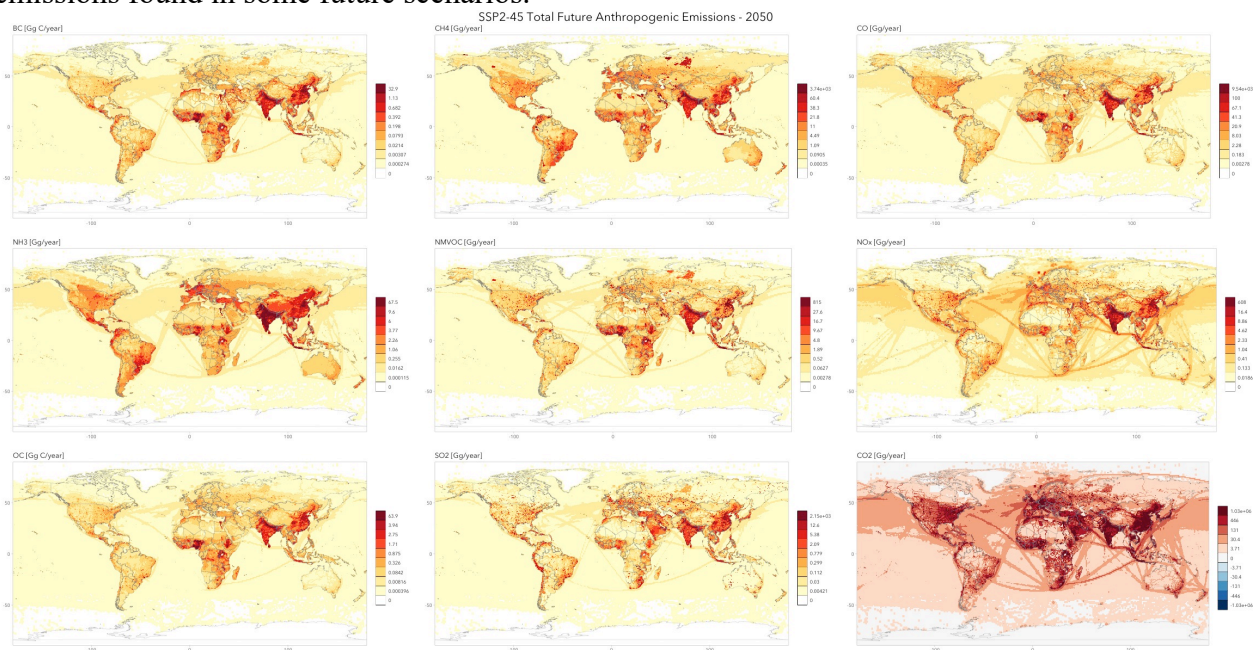
Figure 7 – Total anthropogenic emissions in 2050 by species in the SSP2-45 scenario. Color scale is the same for each emission species across all gridded figures for comparison. The CO 2 color scale accommodates net negative emissions found in some future scenarios.
