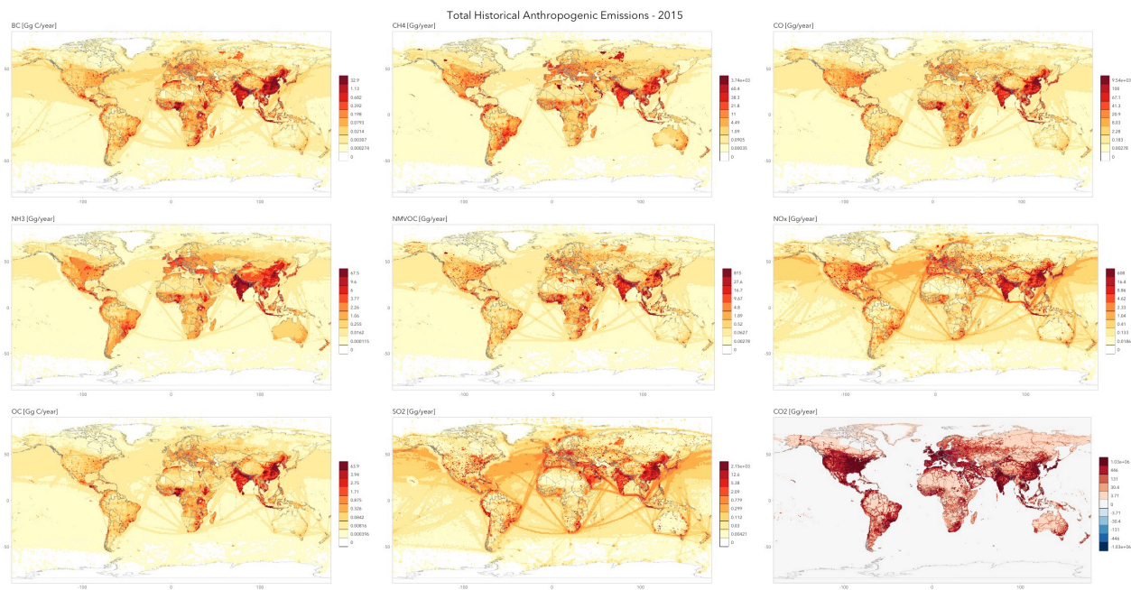
Figure 6 – Total anthropogenic emissions in 2015 by species. Color scale is the same for each emission species across all gridded figures for comparison. The CO 2 color scale accommodates net negative emissions found in some future scenarios.
