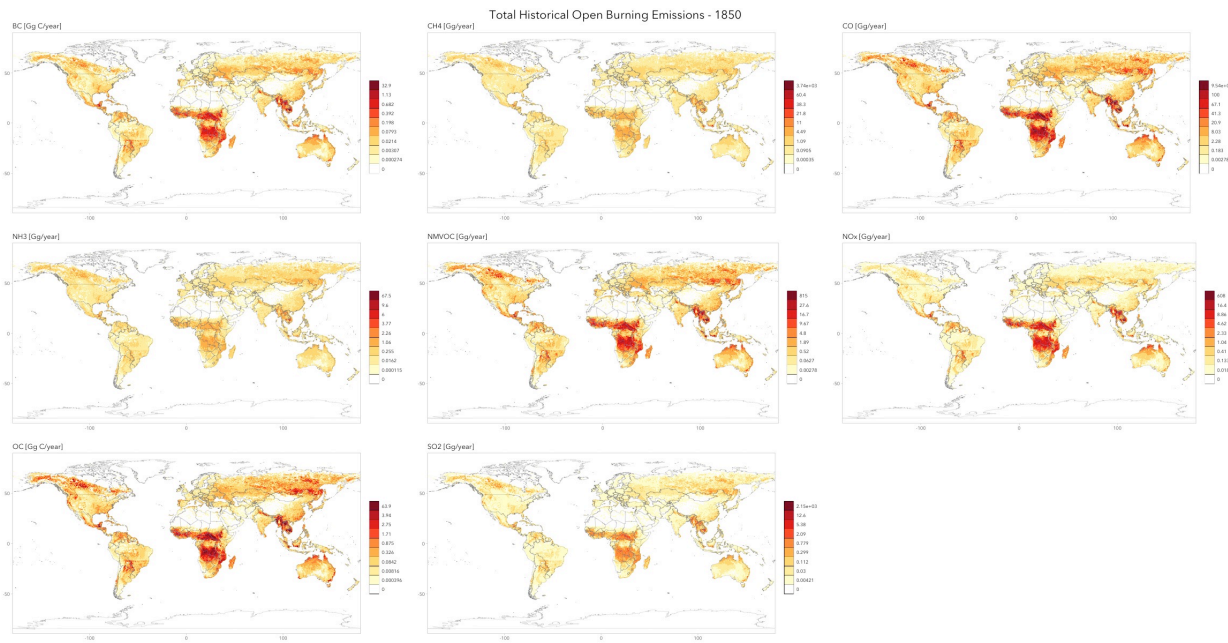
Figure 4 – Total open burning emissions in 1850 by species. Color scale is the same for each emission species across all gridded figures for comparison.
