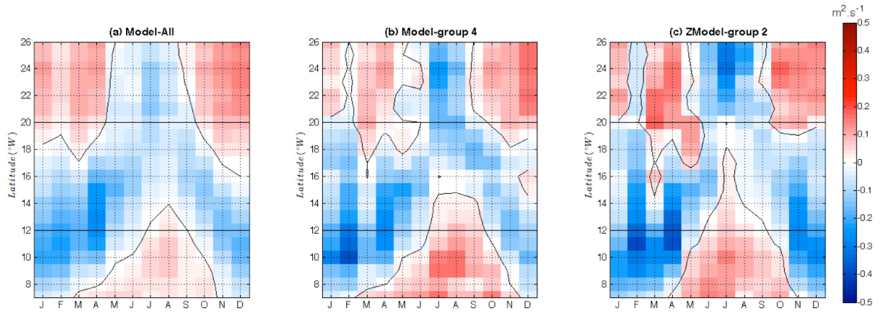
Figure 13: Latitude-time diagram of the seasonal shift of the meridional component of the wind-stress with respect to the present days. For each month and at each latitude, we show the meridional wind stress shift with respect to the present days averaged over the period [2080-2100]. Positive values (red) means that the wind stress shift is southward and is thus favorable to upwelling. Panel (a) stands for Model-All, (b) Model-group 4 and (c) ZModel-group 2.
