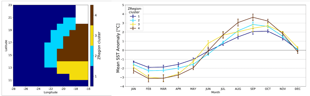
Figure 7: Left panel: ZRegion-clusters associated with the ZSOM-clusters obtained after a HAC on a 10x12 neuron SOM learned on ERSSTv3b observations in the zoomed zone (see text for details). Right Panel: Ensemble-mean monthly climatological SST anomalies for the grid points of the four ZRegion-clusters. The error bars show the standard deviation of this ensemble mean.
