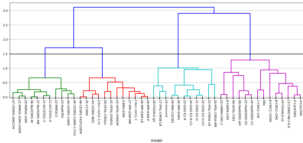
Figure 5: HAC Dendrogram. The horizontal line displays the 47 CMIP5 models, each model being associated with its 7 component skill-vector. As the dendrogram represents a hierarchy of clusters, the numbers on the y axis give the distance between two clusters. We note an optimal ‘jump’ on this graph: the level 1.5 in the vertical axis (materialized by a horizontal black line) is associated with 4 well-separated clusters corresponding to 4 Model-groups that are very different.
