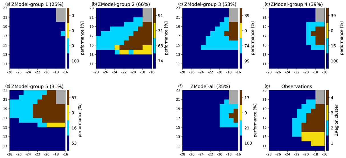
Figure 8: (a)-(e): Projection of the multi-model ensembles (ZModel-groups) onto the ZSOM. The performances are given on top of each panel. The ZRegion-clusters determined by processing the observations in the zoomed region and their associated colors are given in the bottom right panel. The colorbars at the right of each multi-ensemble panel represent the skill (in %) associated with each ZRegion-cluster. Panel (f) shows the same for the full multi-model ensemble. Panel (g) reproduces the Region-clusters based on the observations also shown in Fig. 6.
