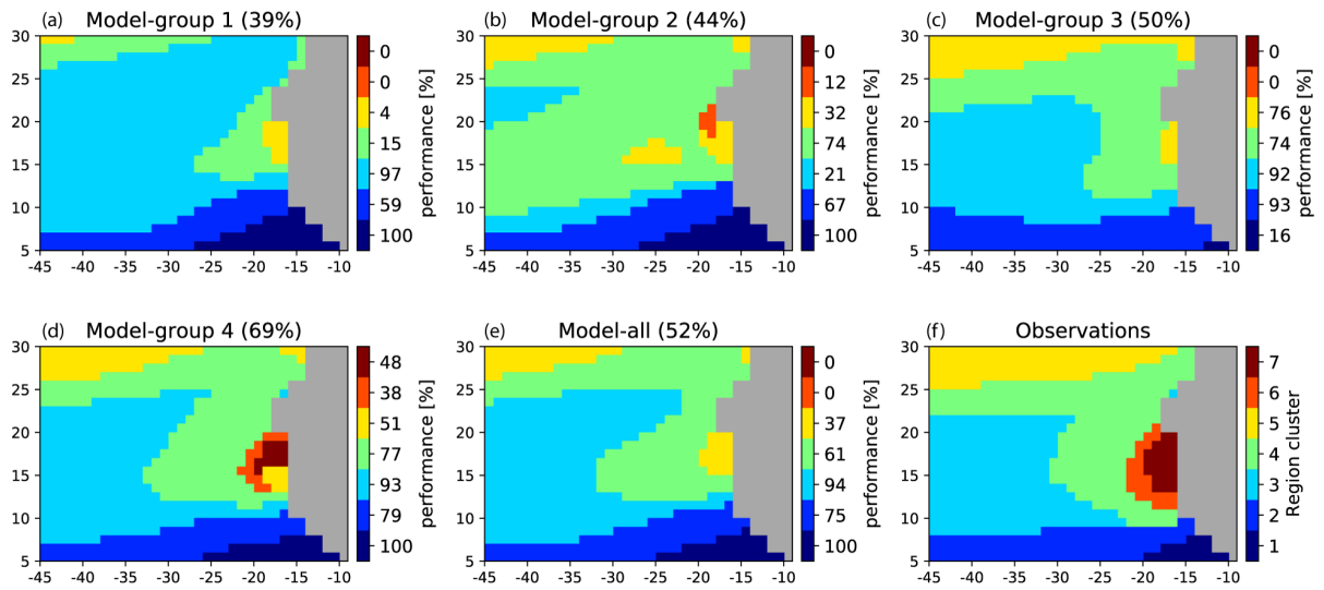
Figure 6: (a)-(d): Projection of the multi-model ensembles (Model-group) onto the SOM learned with ERSSTv3b climatology in the extended zone. Multi-model ensemble performances are obtained by averaging the skill of the models forming each group. The performances are given on top of each panel. The Region-clusters determined by processing the observations in the extended area and their associated colors are given in the bottom right panel. The colorbars at the right of each multi-ensemble panel represent the skill (in %) associated with each Region-cluster. Panel (e) shows the projection for the full multi-model ensemble. Panel (f) reproduces the Region-clusters based on the observations also shown in Fig. 2.
