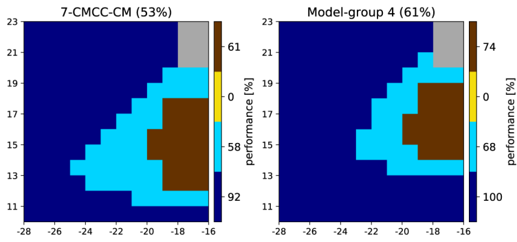
Figure 9 : Same as Fig. 7 but for the individual model CMCC-CM (model 7) (left) and the Model-group 4 (right).
