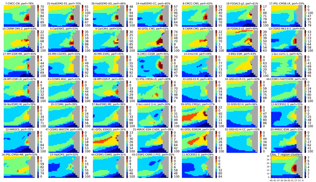
Figure 3: Projection of the 47 climate models of the CMIP5 database onto the SOM learned with ERSSTv3b climatology in the extended zone (see Fig. 1). On top of each panel, we figure: the number referencing the model, its name (Table 1), and its skill given as a mean percentage (see text). The models are ordered according to their skill in decreasing order. The 7 Region-clusters (or SOM-clusters) are defined by applying an HAC to the SOM output learned with the observation field. They are represented by different colors. The numbers in the colorbar at the right of each panel represent the skill for each Region-cluster. The observation field is shown in the bottom right panel and the numbers in front of the colorbar reference the Region-cluster.
