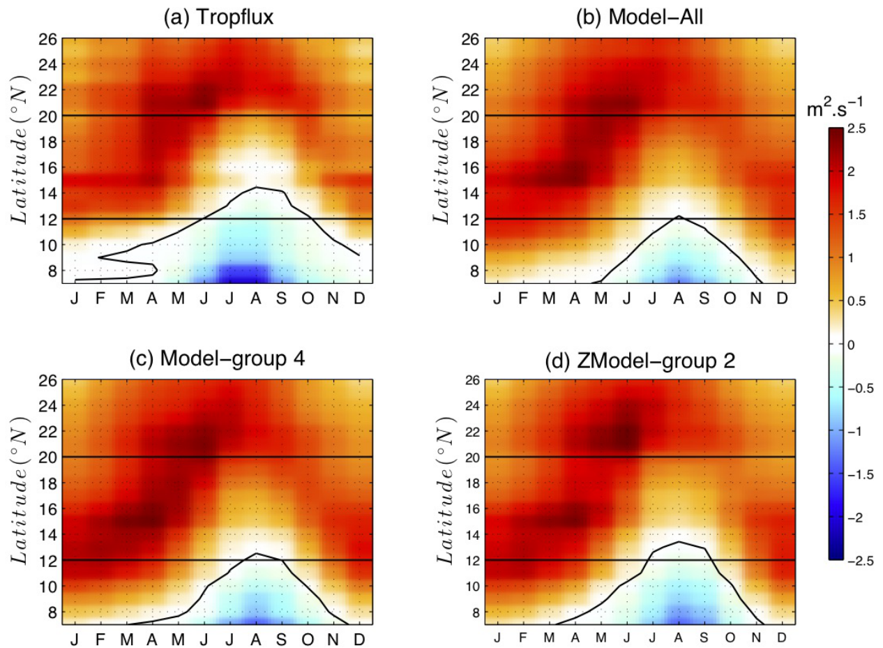
Figure 11: Latitude-time plot of depth integrated Ekman transport computed over the grid point located along the coast (magenta stars in Fig. 9.a). The time axis shows climatological months over the period 1985-2005. Positive (negative) values correspond to upwelling (downwelling) conditions. Panel (a) stands for TropFlux data set (see (Praveen Kumar et al., 2011)) (b) Model-All, (c) Model-group 4 and (d) ZModel-group 2. In each panel, the black contour shows the contour zero. The horizontal dashed lines are positioned at 12 ^{\circ}N and 20 ^{\circ}N and give a rough limitation of the Senegalo-Mauritanian upwelling region.
