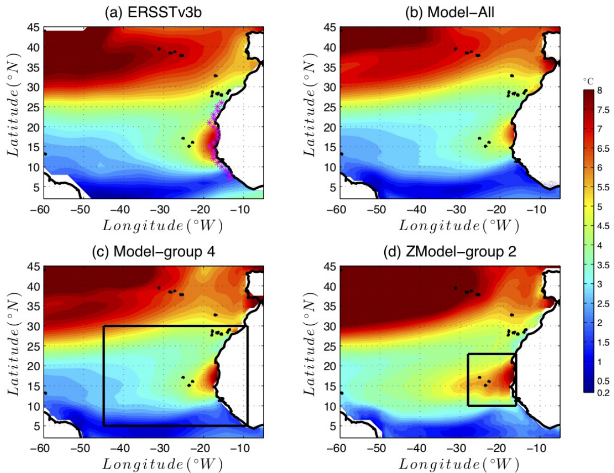
Figure 10: Amplitude of the SST seasonal cycle in the (a) ERSSTv3b Observations (b) Model-All, c) Model-group 4 (best Model-group for the extended area, figured out by the black rectangular box) and (d) ZModel-group 2 (best Model-group for the reduced area, figured out by the small black rectangular box). The SST seasonal cycle is computed over the period 1985-2005
