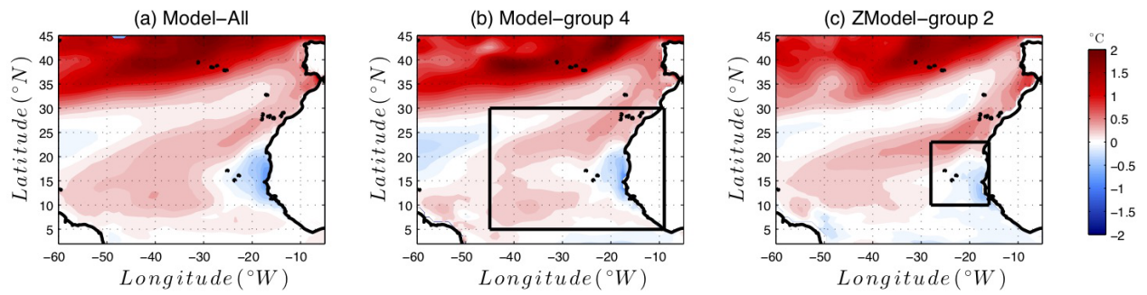
Figure 12: Evolution of the amplitude of the SST seasonal cycle at the end of the 21 st century. The figure shows the difference between the seasonal cycle amplitude averaged over the period [2080-2100] following the RCP8.5 scenario and the amplitude averaged over the period [1985-2005] in the historical simulations. A positive value (red) means that the seasonal cycle is more marked over the period 2080-2100.
