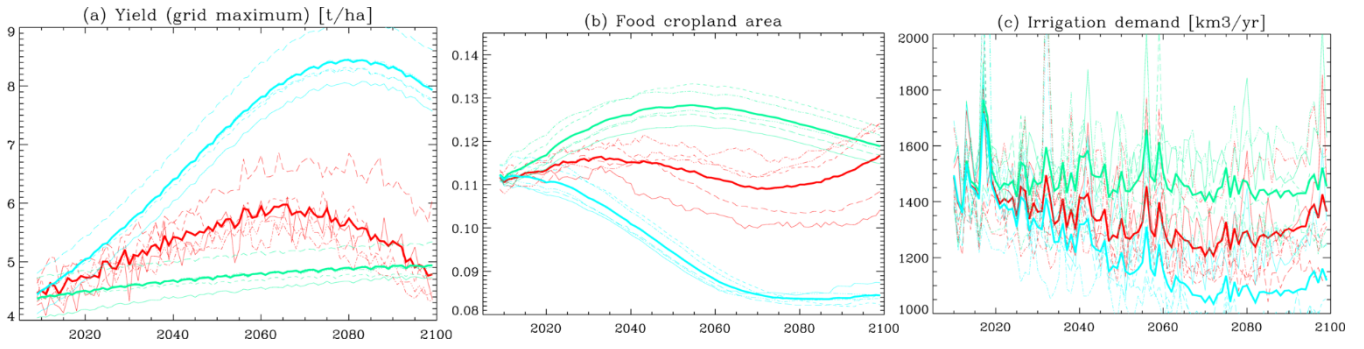
5 Figure 16: Time series of changes in a) cropland yield (maximum across five crops in each grid, t/ha), b) food cropland area (a fraction of total land area), and irrigation demand ( \text{km}^3/\text{yr} ) based on the forcings of the five climate models under the RCP8.5 scenario. Simulations with climatic factors and \text{CO}_2 concentrations fixed at 2006 (light green, noCL+noFE), those with climatic factors fixed (cyan, noCL+FE), and those with varying climate and \text{CO}_2 concentrations (red, CL+FE).
