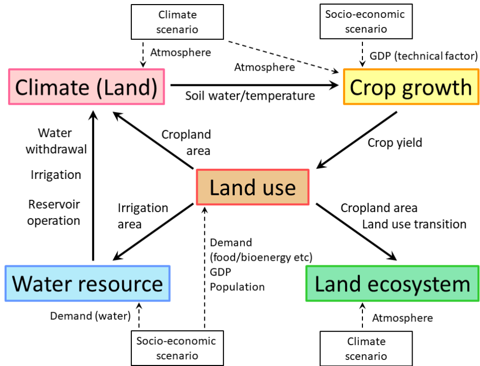
5 Figure 1: Relationship among variables in MIROC-INTEG-LAND. Components of the integrated model (sub-models) are shown 10 as colored boxes. Climate (land surface) and water resource components are HiGWMAT (Pokhrel et al. 2012a), which is based on the land surface model MATSIRO (Nitta et al. 2014) in a global climate model MIROC (Watanabe et al. 2010). Land ecosystem and crop growth components are VISIT (Ito and Inatomi 2012) and PRYSBI2 (Sakurai et al. 2014), respectively. The land use model, TeLMO, is developed in this study. Inputs into the model are shown as boxes of climate and socio-economic scenarios. Solid arrows between the boxes indicate the exchange of variables between the sub-models. Dashed arrows indicate the input variables of the sub-models.
