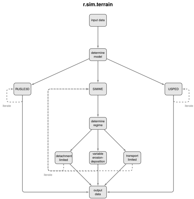
Fig. 1. Concept diagram for r.sim.terrain
