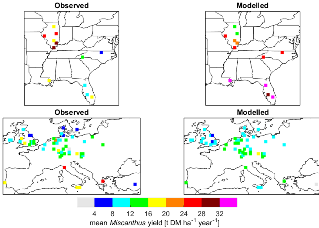
Figure 4. Comparison of modelled Miscanthus yields against observations from Li et al. (2018a).
