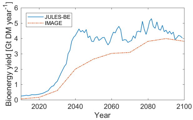
Figure 8. Bioenergy crop yield from Miscanthus under the land-use scenario RCP2.6-SSP2, compared to equivalent bioenergy yield in IMAGE (Huppmann et al., 2018).
