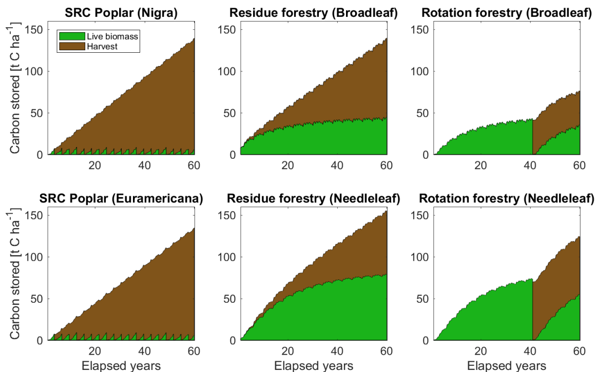
Figure 9. Illustrated cumulative harvests and vegetation regrowth over a 60-year period, showing the application of JULES-BE to short rotation coppicing (left); harvest of residues from forestry (middle), and rotation forestry (right).
