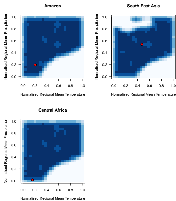
Figure 16. Density of not-ruled-out yet emulated temperature and precipitation pairs for each observed tropical forest fraction, when input parameters are held at their default values. Observed climates for each forest are marked in red.
