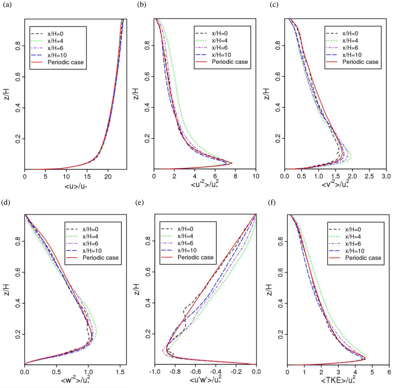
5 Figure 5: Spatially and temporally averaged vertical profiles of (a) \langle u \rangle / u_* , (b) \langle u'^2 \rangle / u_*^2 , (c) \langle v'^2 \rangle / u_*^2 , (d) \langle w'^2 \rangle / u_*^2 , (e) \langle u'w' \rangle / u_*^2 , and (f) \langle TKE \rangle / u_*^2 at a series of downwind locations in the inflow case (LS1.0), and the periodic case (also averaged in the streamwise direction).
