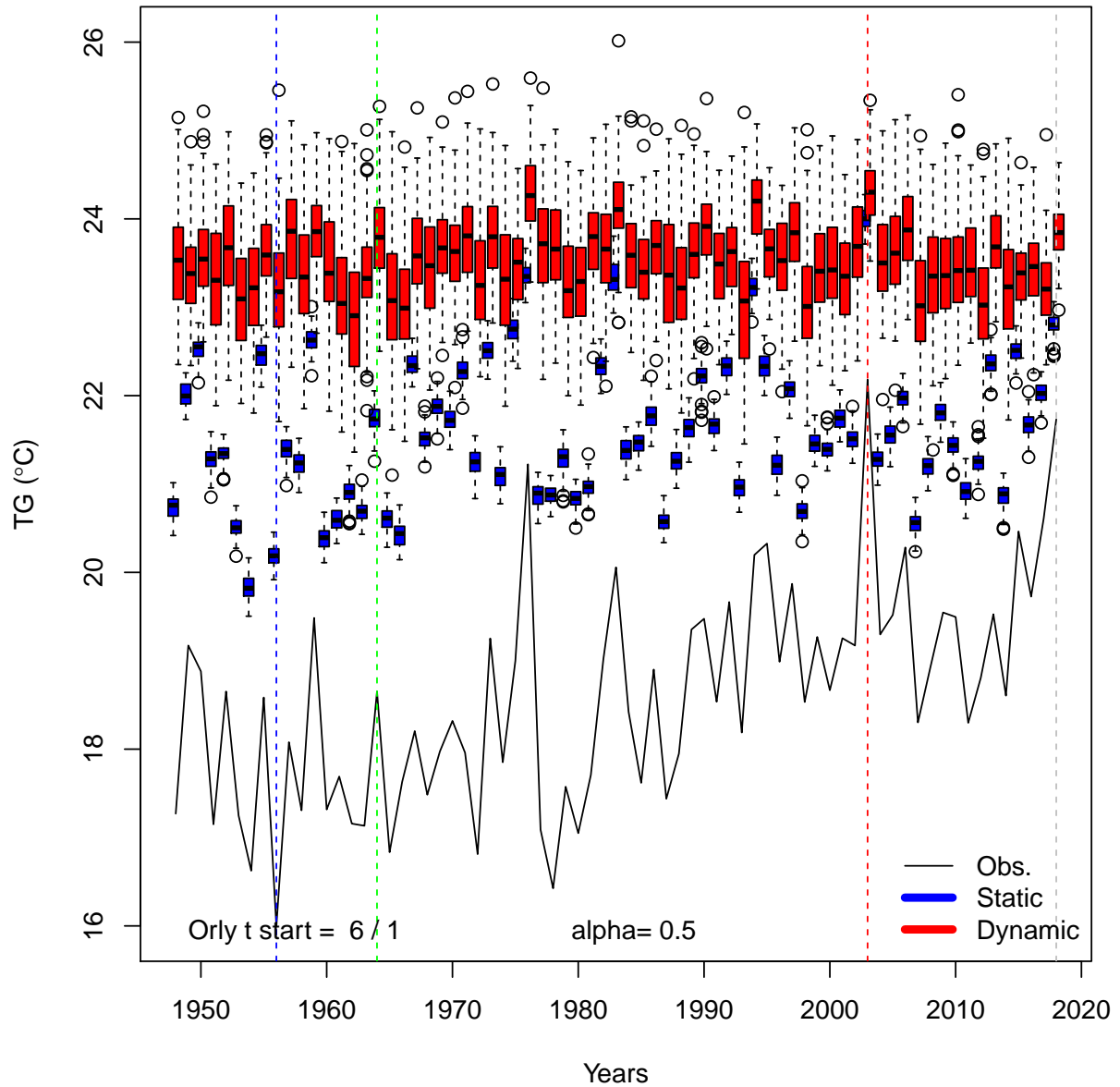
Figure A3. Time variations of probability distributions of simulated average temperatures ( TG ) for \alpha_{TG} = 0.5 in Orly, for \alpha_{TG} = 0.5 . The black continuous line represents the observed variations of Orly summer averages between 1948 and 2018. Temperatures are expressed in ^{\circ}\text{C} . The vertical colored lines indicate the warmest-coldest (red: 2003), coolest (blue: 1956), warmest (red) and 2018 summers. The boxplots represent the ensemble variability of the simulations for each year. The red boxplots are for the dynamic simulations. The blue boxplots are for the static simulations. The boxes of boxplots indicate the median (green: 1964), lower ( q_{25} ) and upper ( q_{75} ) quartiles. The upper whiskers indicate \min[\max(T), 1.5 \times (q_{75} - q_{25})] . The lower whisker has a symmetric formulation. The points are the simulated values that are above or below the defined whiskers.
