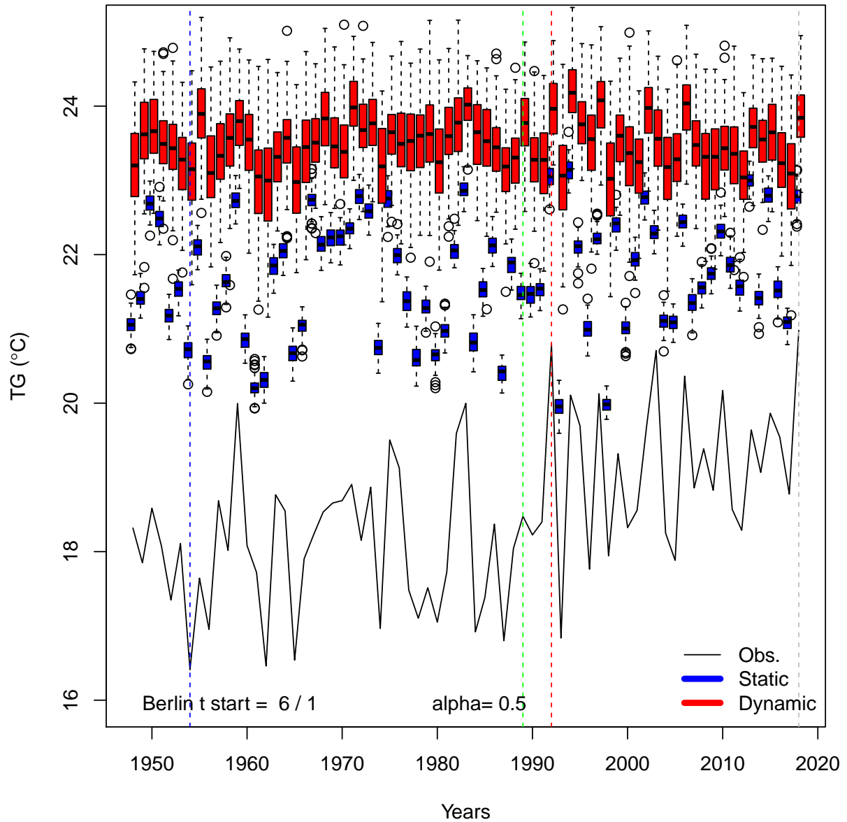
Figure A1. Time variations of probability distributions of simulated average temperatures ( TG ) for \alpha_{TG} = 0.5 in Berlin, for \alpha_{TG} = 0.5 . Vertical dashed lines indicate the warmest (red: 1992), coldest (blue: 1954), median (green: 1989) and 2008 summers. The boxplots represent the ensemble variability of the simulations for each year. The red boxplots are for the dynamic simulations. The blue boxplots are for the static simulations. The boxes of boxplots indicate the median (green: 1989), lower ( q_{25} ) and upper ( q_{75} ) quartiles. The upper whiskers indicate \min[\max(T), 1.5 \times (q_{75} - q_{25})] . The lower whisker has a symmetric formulation. The points are the simulated values that are above or below the defined whiskers.
