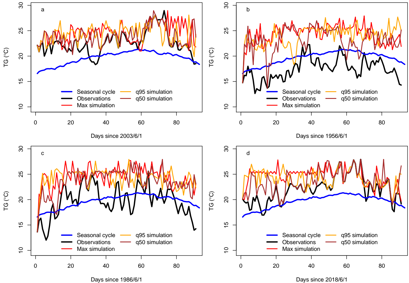
Figure 6. Observed and simulated daily temperature (TG) variations (for the Berlin-De Bilt-Orly-Toulouse-Madrid (BDOTM) average) for the four selected summers: 2003 (panel a), 1956 (panel b), 1986 (panel c) and 2018 (panel d). Temperatures are expressed in °C. The simulation parameters are \alpha_{cal} = 5 and \alpha = 0.5 . The blue lines indicate the average seasonal cycle. The black lines are the observed TG. The red lines are the simulations with the highest JJA mean TG. The dashed lines are the simulations with the 95th quantile of JJA mean TG. The brown lines are for the median simulations.
