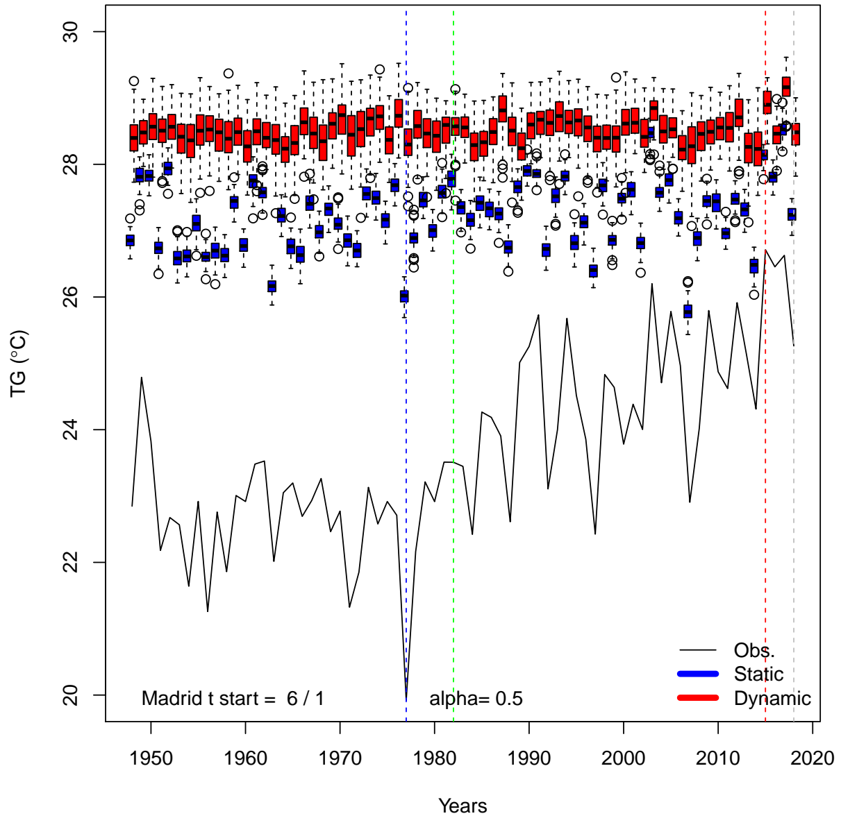
Figure A5. Time variations of probability distributions of simulated average temperatures ( TG ) for \alpha_{TG} = 0.5 in Madrid, for \alpha_{TG} = 0.5 . Vertical-dashed. The black continuous line represents the observed variations of Orly summer averages between 1948 and 2018. Temperatures are expressed in ^{\circ}\text{C} . The vertical colored lines indicate the warmest-coldest (red: 2015, blue: 1977), coolest-median (green: 1982), warmest (red) and 2018 summers. The boxplots represent the ensemble variability of the simulations for each year. The red boxplots are for the dynamic simulations. The blue boxplots are for the static simulations. The boxes of boxplots indicate the median (green: 1982), lower ( q_{25} ) and upper ( q_{75} ) quartiles. The upper whiskers indicate \min[\max(T), 1.5 \times (q_{75} - q_{25})] . The lower whisker has a symmetric formulation. The points are the simulated values that are above or below the defined whiskers.
