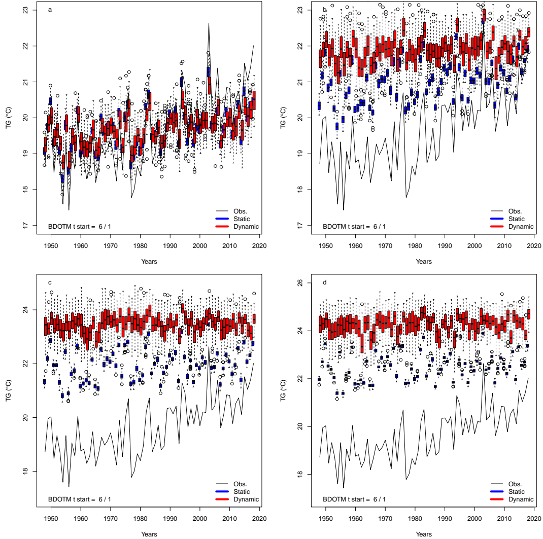
Figure 4. Time variations of probability distributions of simulated average temperatures ( TG in ^{\circ}C ) for four values of the weight on temperatures atg \in \{0, 0.2, 0.5, 1\} : atg = 0 (a), atg = 0.2 (b), atg = 0.5 (c), atg = 1 (d). The black continuous line represents the observed variations of Berlin-De Bilt-Orly-Toulouse-Madrid (BDOTM) summer averages between 1948 and 2018. The vertical colored lines outline the coldest (blue), median (green), warmest (red) and 2018 summers. The boxplots represent the ensemble variability of the simulations for each year. The red boxplots are for the dynamic simulations. The blue boxplots are for the static simulations. The boxes of boxplots indicate the median ( q_{50} ), lower ( q_{25} ) and upper ( q_{75} ) quartiles. The upper whiskers indicate \min[\max(T), 1.5 \times (q_{75} - q_{25})] . The lower whisker has a symmetric formulation. The points are the simulated values that are above or below the defined whiskers.
