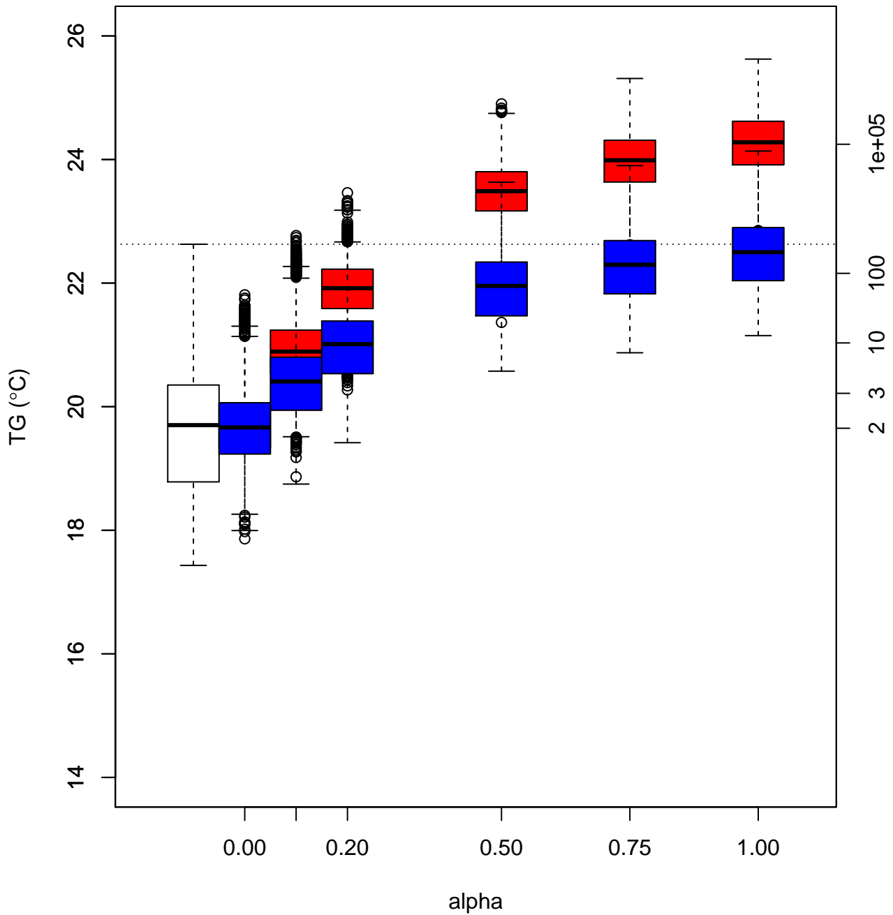
Figure 5. Boxplots of simulated June-July-August (JJA) temperatures ( TG in °C ) as a function of the parameter \alpha for all years. The boxes of boxplots indicate the median ( q_{50} ), lower ( q_{25} ) and upper ( q_{75} ) quartiles of the simulated values. The upper whiskers indicate \min[\max(T), 1.5 \times (q_{75} - q_{25})] . The lower whisker has a symmetric formulation. The points are the simulated values that are above or below the defined whiskers. The axis on the right indicates return times (in years), assuming a Gaussian distribution of JJA temperature averages with parameters estimated from the white boxplot. The horizontal dotted line is the mean TG in 2003.
