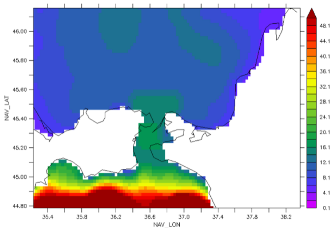
Fig. 1. Detailed model bathymetry around the Kerch Strait
