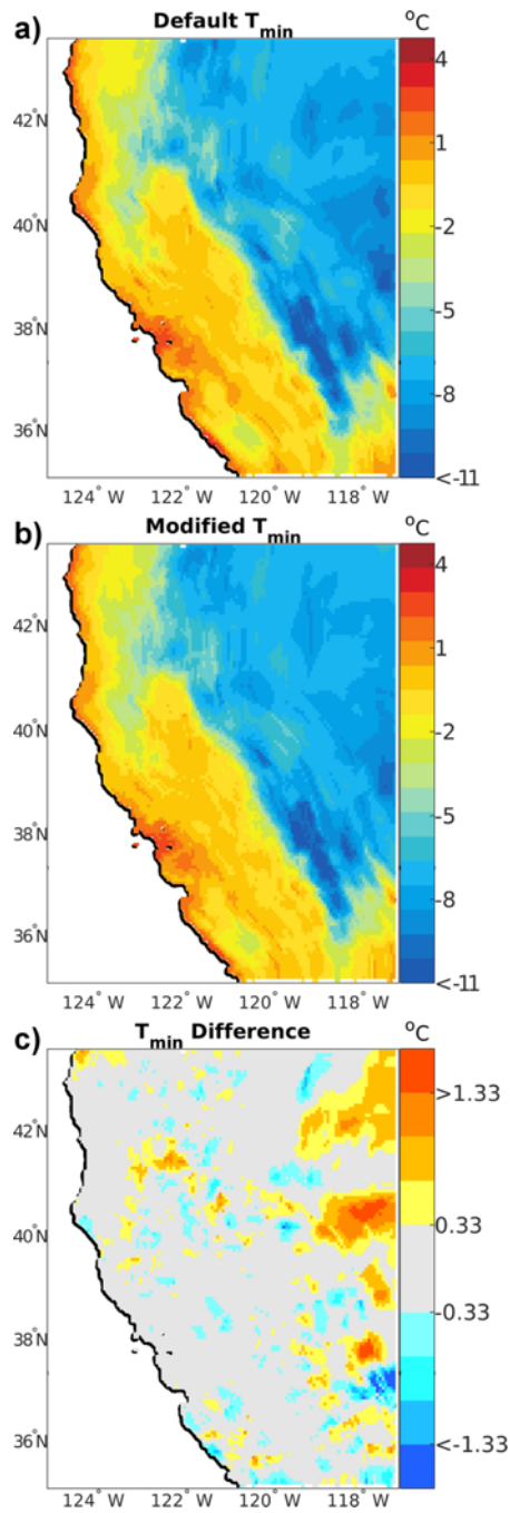
Figure 9: Spatial distribution of minimum temperature ( T_{\min} , °C) for model parameter sensitivity experiment 1. a) default model parameters, b) modified distance weighting exponent, and c) the difference field (default – modified).
