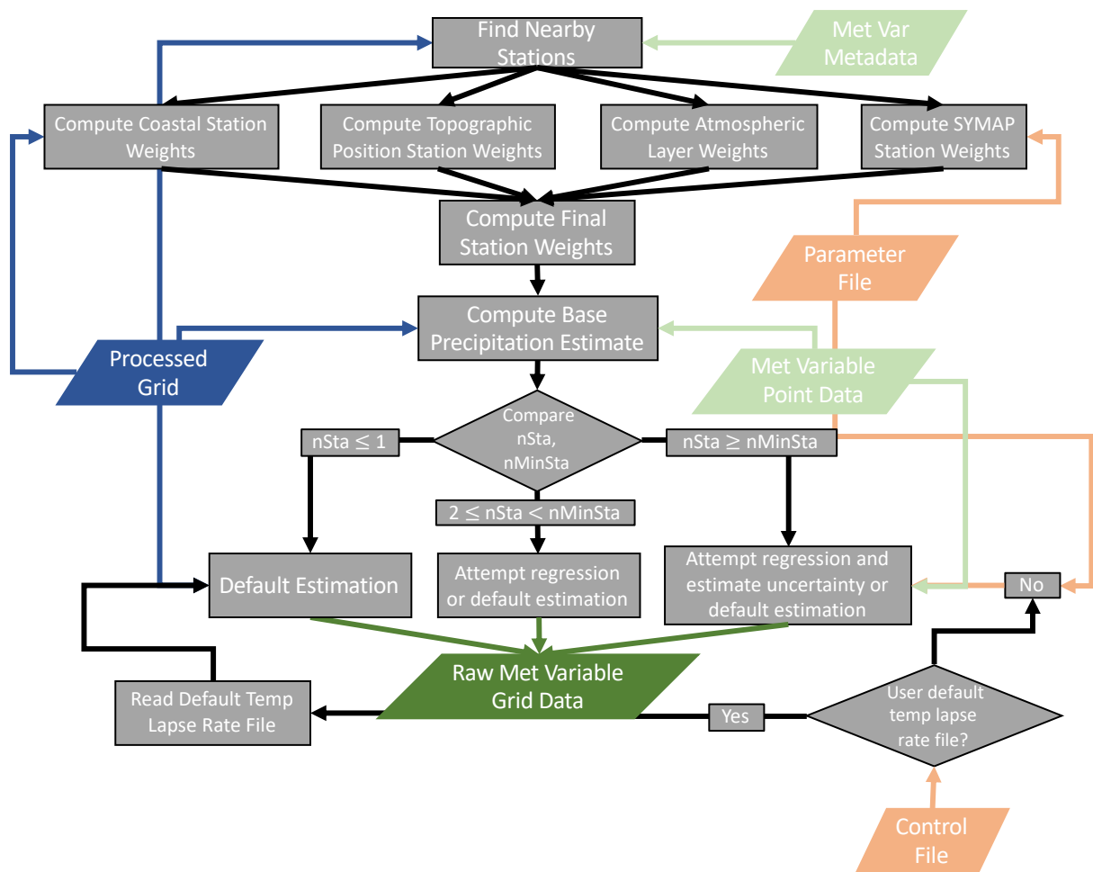
Figure 4: Flow chart describing the temperature grid point estimate algorithm. Color shading is the same as Figure 1.
