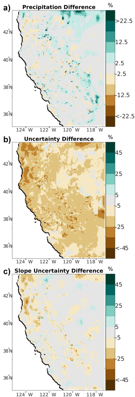
Figure 11: Spatial distribution of differences for model parameter sensitivity experiment 3, modified maximum number of stations parameter (nMaxNear). a) precipitation differences (%), b) total uncertainty differences (%), and c) uncertainty changes due to the slope term in the regression.
