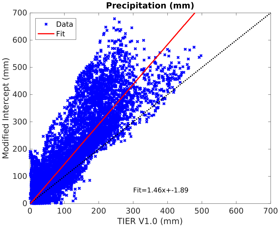
Figure 8: Comparison of precipitation (mm) estimates using \hat{\beta}_0 in Eq. 15. versus TIER v1.0 which uses \hat{\mu}_{b_o} in Eq. 15.
