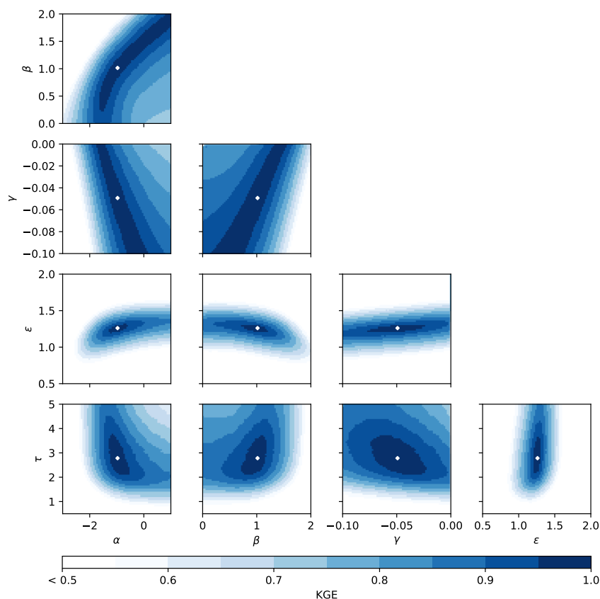
Figure 8. Response surface plots with the Kling-Gupta efficiency (KGE) as the performance metric for a synthetic experiment. The white dot in the middle of each graph represents the location where KGE is equal to 1. Each plot consists of 4900 model runs – where the model has 200 cells, ran for one year on hourly timestep – and took 1 hour and 15 minutes to run on a normal desktop (Intel Core i7-6700, 16GB RAM).
