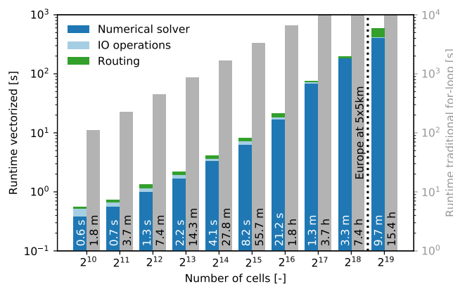
Figure 5. Runtimes for a simulation of three months with an hourly time step with varying number of pixels, ran on a single core of a normal desktop (Intel Core i7-6700, 16GB RAM). The grey bars represent model run times where the numerical solver is called for each individual pixel, and are keyed to the right hand scale, making the difference in runtimes appear smaller than it really is. The dotted line represents the number of pixels when simulating Europe at 5 \times 5 \text{ km}^2 resolution.
