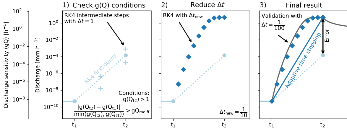
Figure 6. Three steps in the adaptive time stepping scheme. Note that in extreme cases, both Q and g(Q) can change over several orders of magnitude between t_1 and t_2 . The error represents the numerical error without the adaptive time stepping scheme.
