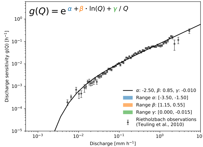
Figure 2. Parameterization of the discharge sensitivity, including the effects of the three parameters. \alpha affects the intercept, \beta affects the slope and \gamma affects the curvature at low discharge values. Parameter values for each parameter are given in the legend as their min-max range.
