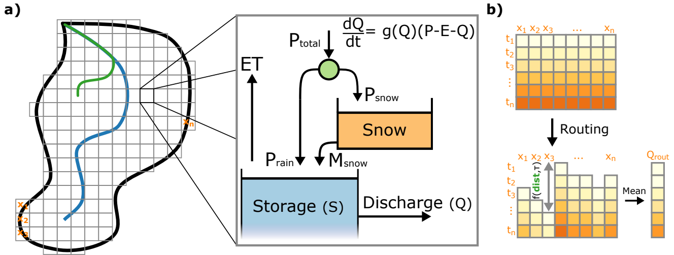
Figure 1. Efficient distributed implementation of the simple dynamical systems approach, which is solved for each pixel. The left hand side of panel a represents a catchment, with a regular grid covering the catchment area. The green line indicates the flow path on which the routing lag is based (green “dist” in panel b). Panel b shows how the catchment is translated to a matrix to allow for computationally efficient calculations, and how the matrix is modified in the routing algorithm, by shifting each column based on the distance to the outlet and the routing parameter \tau .
