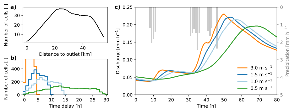
Figure 4. The routing concept visualized: a) the width function of a synthetic catchment, b) the corresponding travel speed given four different \tau values, and c) the effect of different \tau values on the hydrograph.
