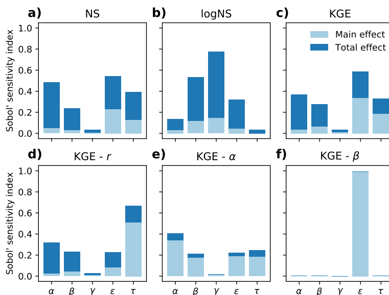
Figure 9. Sobol' parameter sensitivity for a synthetic experiment, shown for different performance statistics. The bottom row (panels d to f) show the three components of the Kling-Gupta efficiency: Pearson correlation coefficient (KGE - r ), ratio of variability (KGE - \alpha ) and bias (KGE - \beta ).
