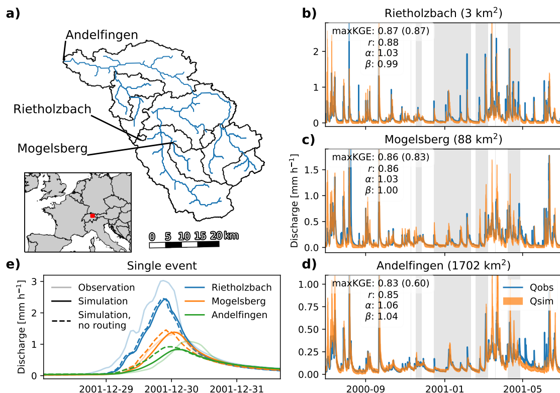
Figure 10. Application of dS2 to the Thur basin in Switzerland, where a) depicts the stream network and sub-basins used in this example. Graphs b) to d) present the model performance in three basins across different orders of sizes. The shaded orange region shows the minimum and maximum discharge of the selected best runs. Periods where more than 20% of the basin is covered with snow are indicated with the grey background. Graph e) shows how a single precipitation event is translated through the different (sub-)basins, where the light colours indicate the observed discharge, the dark lines represent the simulated discharge, and the dashed lines represent the simulated discharge without a delay induced by the routing module.
