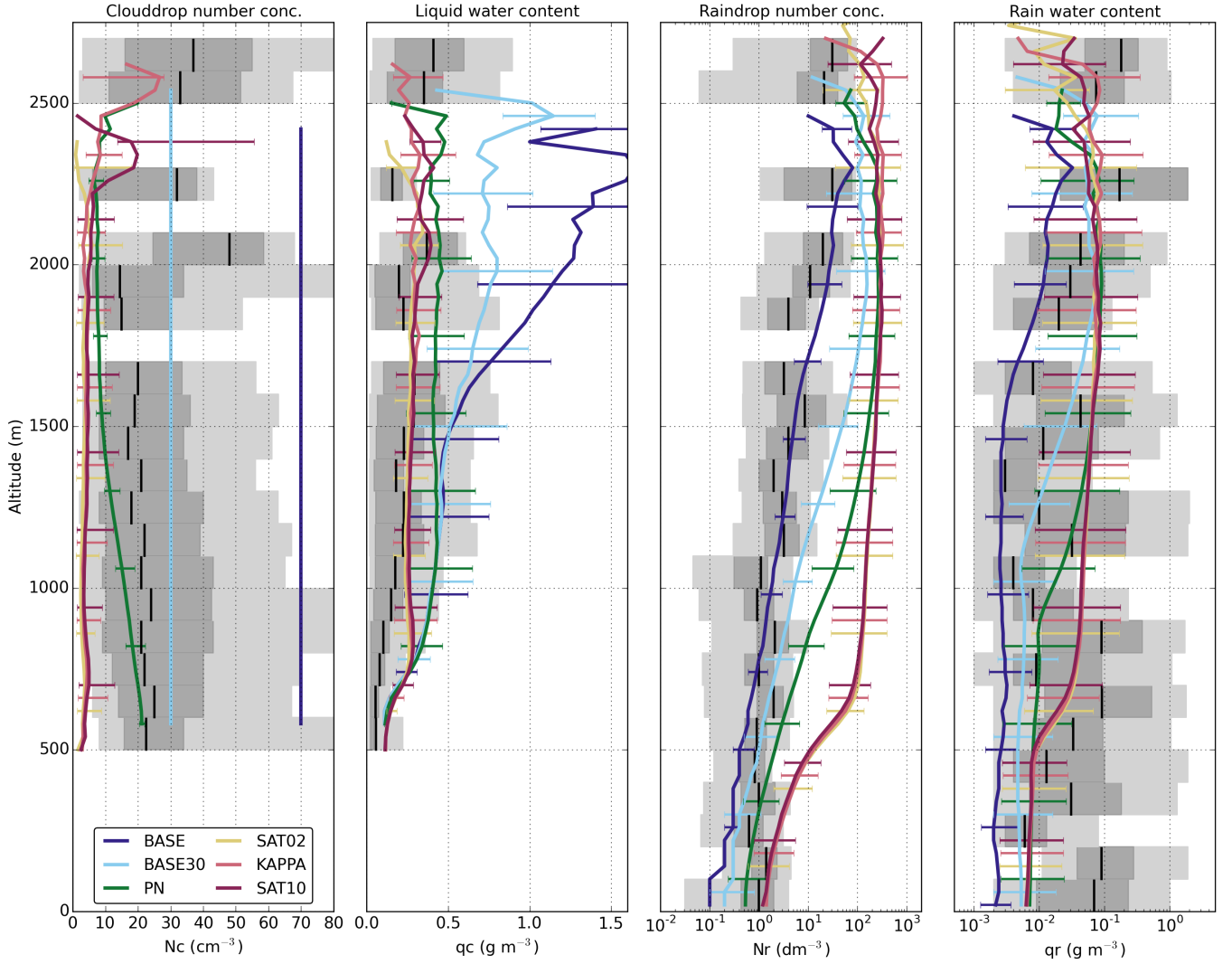
Figure 4. Validation of modeled cloud and rain characteristics against observations of a) cloud droplet number concentration N_c , b) cloud liquid water q_c , c) rain drop number concentration N_r , and d) rain water content q_r . Observations are grouped by altitude using increments of 100 m. Median value is shown by vertical black bars, light grey shading indicates the 5th to 95th percentile, while dark grey indicates 25th to 75th percentile. Median simulated values are represented by colored lines with the errorbars indicating the 25th to 75th percentile.
