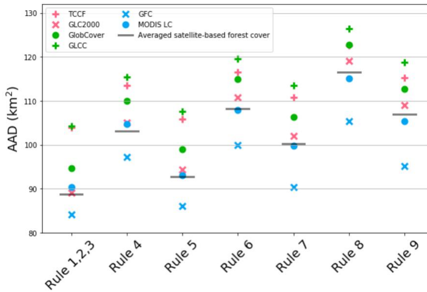
Figure 4. Global average of absolute difference in forest area estimated by translation rules, and each of the six satellite-based forest cover maps as well as the averaged satellite-based forest cover map.
