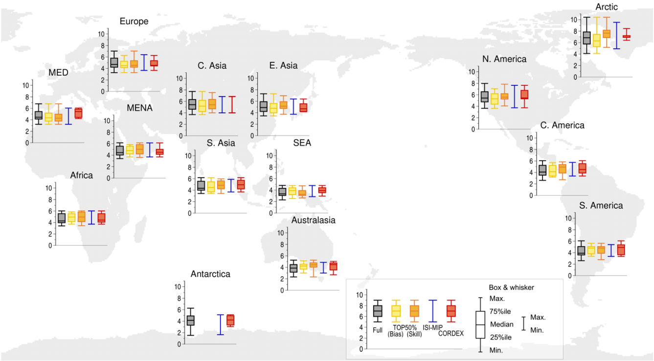
Figure 2: Annual mean temperature increments in the future climate projection (K). The whiskers of the box plots show the range between the maximum and the minimum biases. The boxes and the lines within the boxes show the 25th to 75th percentile range and the median, respectively. Box plots indicate the model bias in the full set of 42 CMIP5 models (black), the model sets with the top 50% of the CMIP5 models for the bias (yellow) or Taylor’s skill score (orange), and the model sets selected for ISIMIP (blue) and CORDEX (red). The top 50% of the CMIP5 models cannot be plotted over Antarctica because of missing the CRU reference data.
