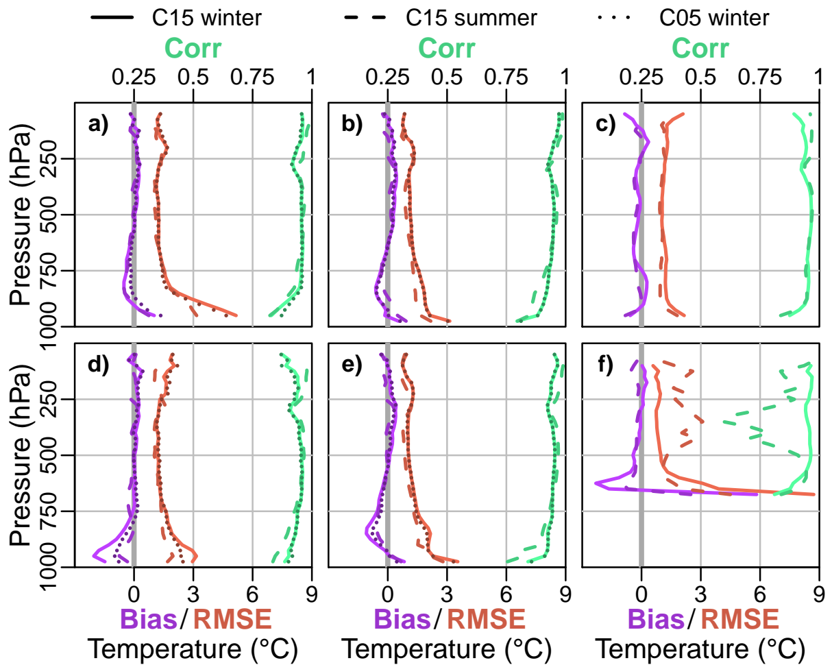
Figure 12. Temperature bias, RMSE (bottom axis) and correlation (top axis) of C15 during winter (solid line), C15 during summer (dashed line) and C05 during winter (dotted line) for the stations Marambio (a), Neumayer (b), Novolazarevskaya (c), Rothera (d), Halley (e) and Amundsen Scott (f).
