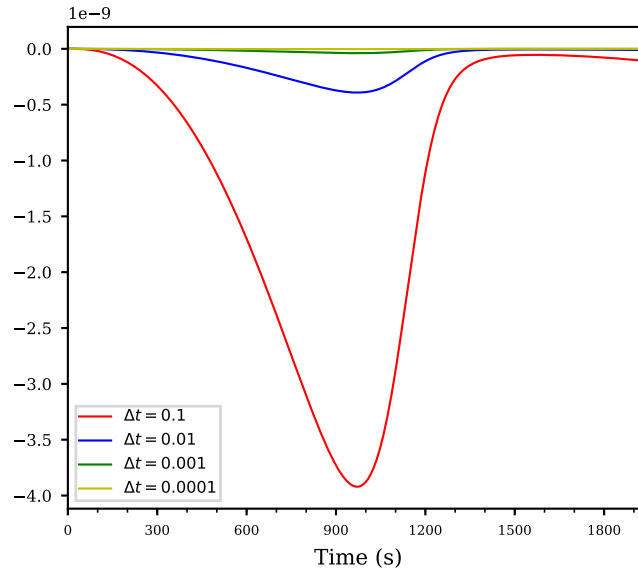
Figure 4. Temporal evolution of the derivative \frac{\partial q_c}{\partial \alpha_1} using the timesteps \Delta t \in \{0.1\text{s}, 0.01\text{s}, 0.001\text{s}, 0.0001\text{s}\} for the computation of the same case as in Figure 2.
