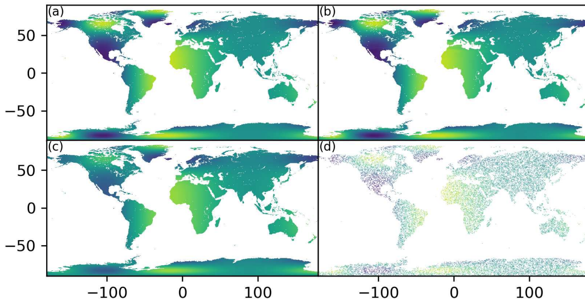
Figure 9. The synthetic fields of the true state (a), the posterior state (b) after the assimilation, the prior state (c) before the assimilation, and the observations (d) for the medium scale problem. Please refer to the second paragraph of Section 4.2.1 for the generations of these synthetic fields.
