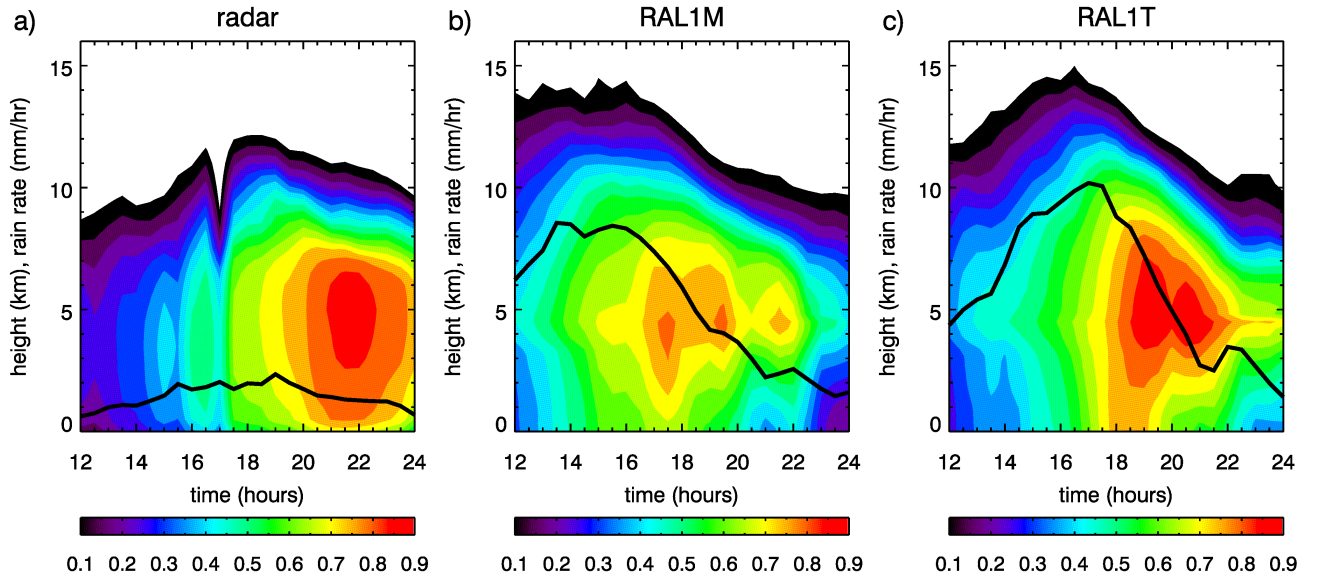
Figure 17. Fraction of radar area covered by reflectivities greater than 10 dBZ as a function of height and time (coloured contours) from 12:00 to 24:00 UTC on 18 February 2014. Solid lines are the time series of the domain mean rain rate (mm/hr).
