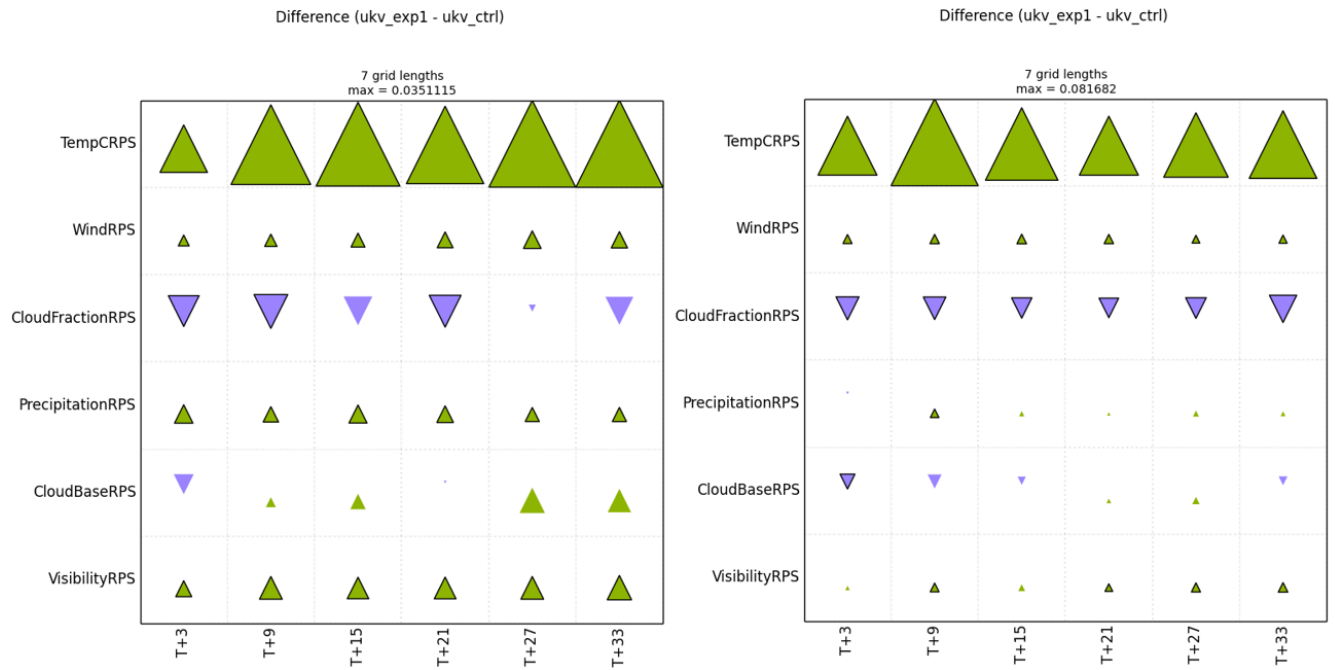
Figure 5. 3DVAR trials: RAL1-M vs RAL0 HiRA summary scorecard at 10.5km (7 grid-lengths) spatial scale for Winter (left) and Summer (right).
