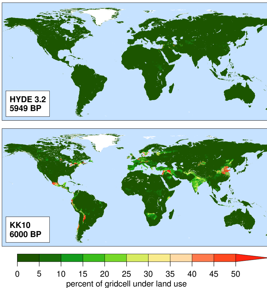
Figure 1: Land use at ca 6000 years ago (6ka BP, 4000 years BCE), from the two widely used global historical land-use scenarios HYDE 3.2 (top panel, Klein Goldewijk et al. 2017a) and KK10 (bottom panel, Kaplan et al. 2011), illustrating the large disagreement between LULC scenarios at a regional scale. In both scenarios, the land-sea mask and lake areas are for the present day.
