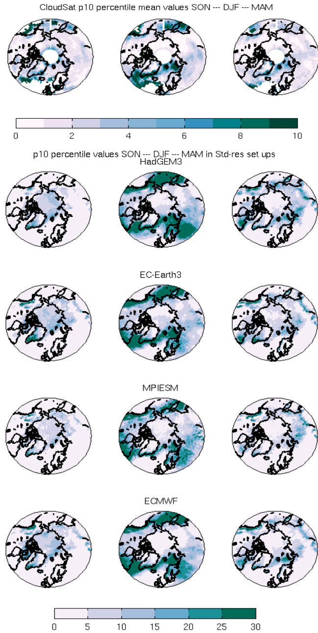
Figure S1. 10-percentile thresholds of monthly snowfall accumulations (mm/month) for the SON, DJF and MAM months in the 3 columns respectively. The top row shows the CloudSat observations and the other four rows below show snowfall from the Low-Res (or Std-Res) setups of HadGEM3, EC-Earth3, MPIESM and ECMWF respectively.
