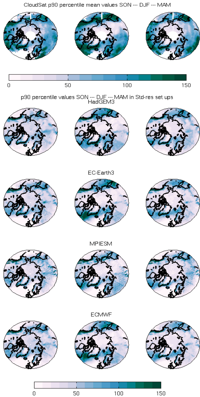
Figure S3. Same as Fig. S1, but, at 90-percentile threshold.
