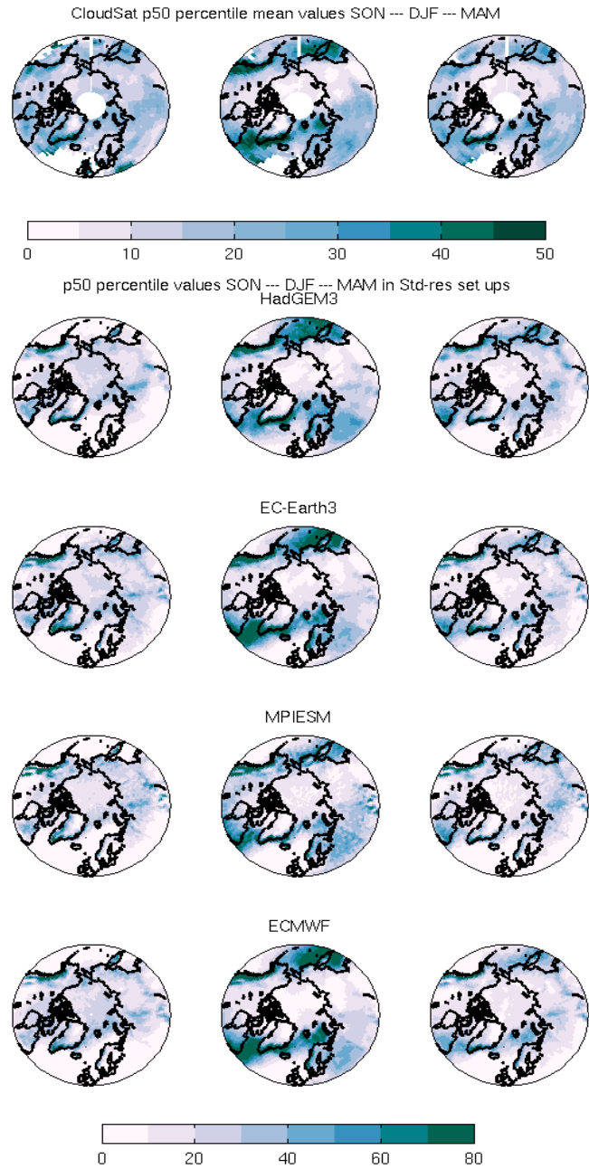
Figure S2. Same as Fig. S1, but, at 50-percentile threshold.
