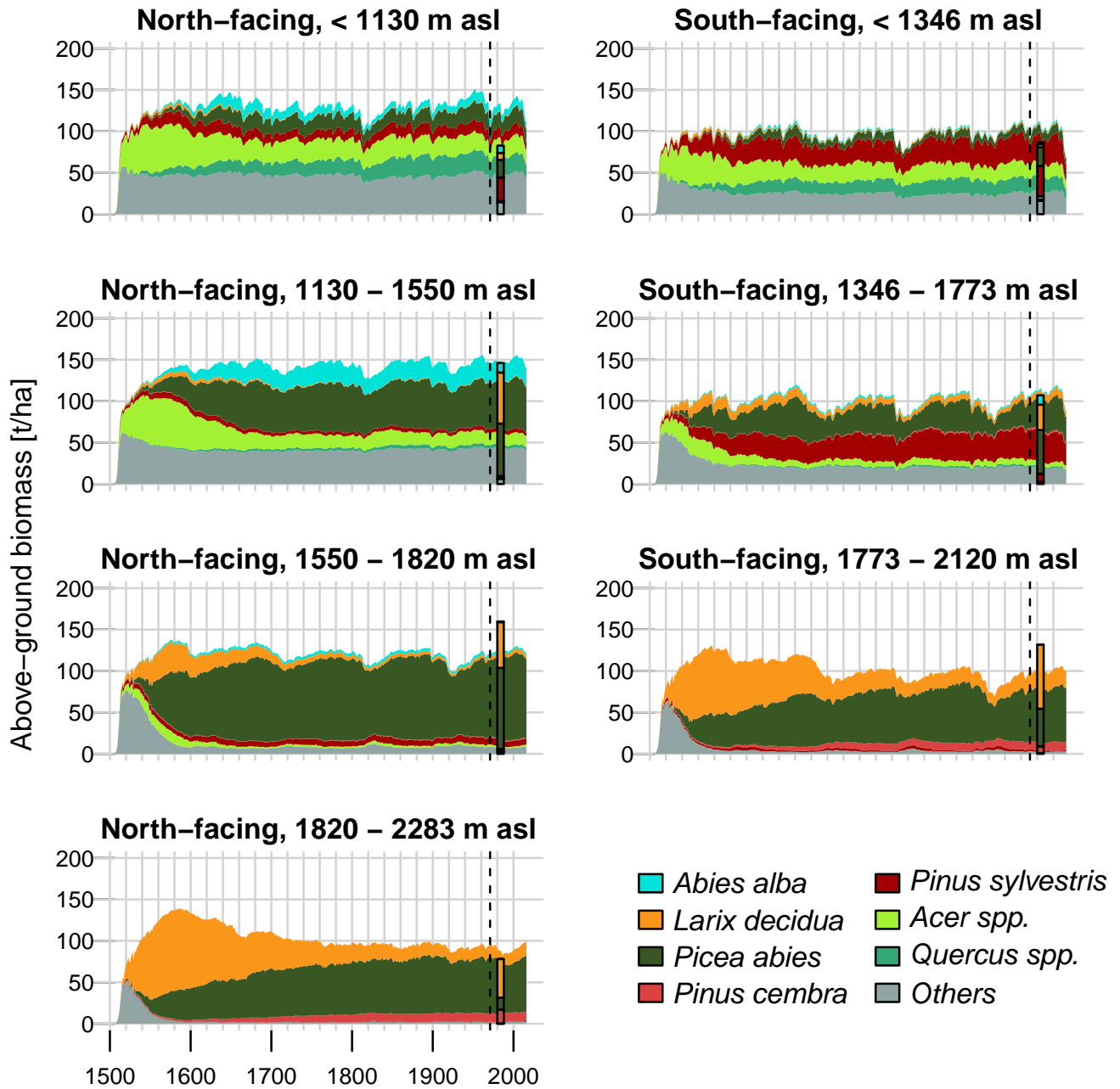
Figure 6. Aboveground tree biomass simulated with FORHYCS using the configuration S_noLared (Table 1). The graphs show annual values, averaged over seven clusters of cells. The bar shows the aboveground biomass in the same area, from the first Swiss national forest inventory (1982-1986; Bachofen et al., 1988). The limits of the elevation bands were set so that each cluster contains at least 30 forest inventory plots. The dashed line marks the year 1971, from when meteorological data are available. Simulation years before 1971 use meteorological data bootstrapped from the years 1981-2000.
