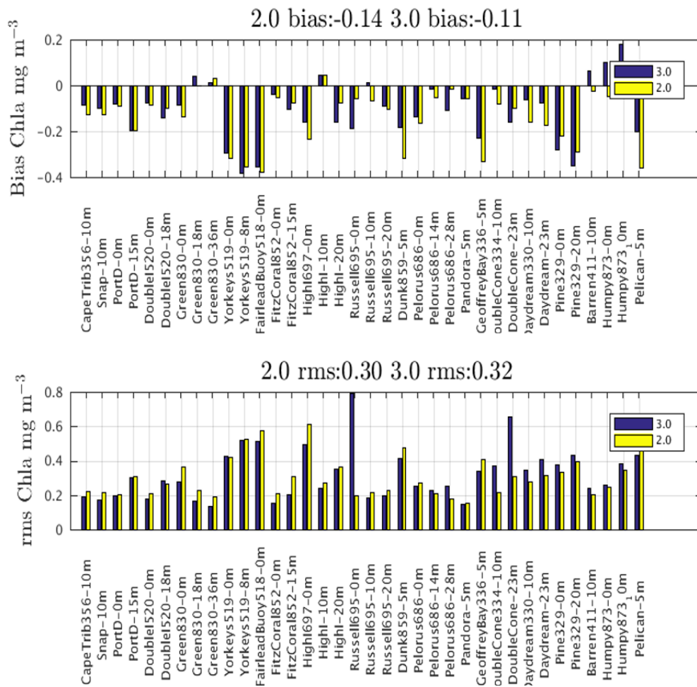
Figure 15. Skill metrics for the comparison of chlorophyll extracts at the Long Term Monitoring sites against observations for model version 2p0 and 3p0. For more information see Fig. 14 and S5, Sec. 10.
