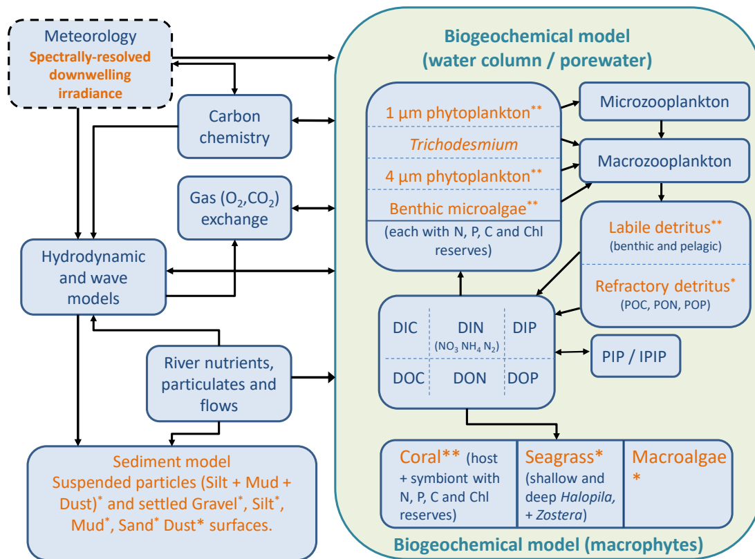
Figure 3. Schematic of the CSIRO Environmental Modelling Suite, illustrating the biogeochemical processes in the water column, epipelagic and sediment zones, as well as the carbon chemistry and gas exchange used in vB3p0 for the Great Barrier Reef application. Orange labels represent components that scatter or absorb light.
