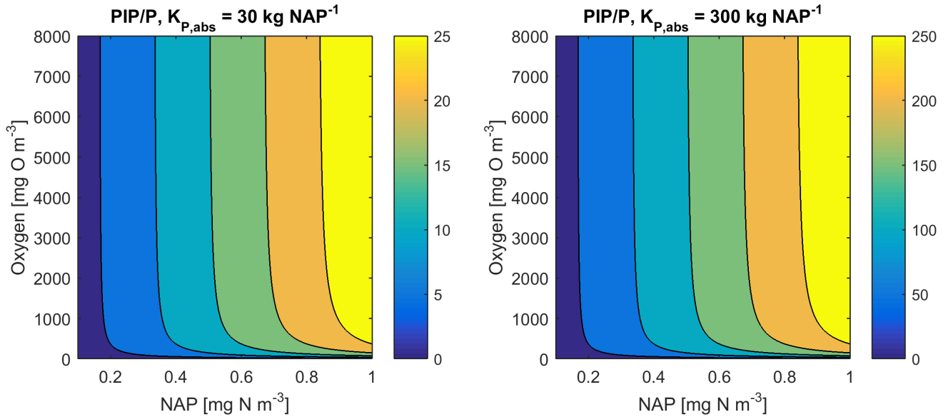
Figure 12. Phosphorus adsorption - desorption equilibria, K_{O_2,abs} = 74 \text{ mg O m}^{-3} at two values of K_{Pads,wc} .
