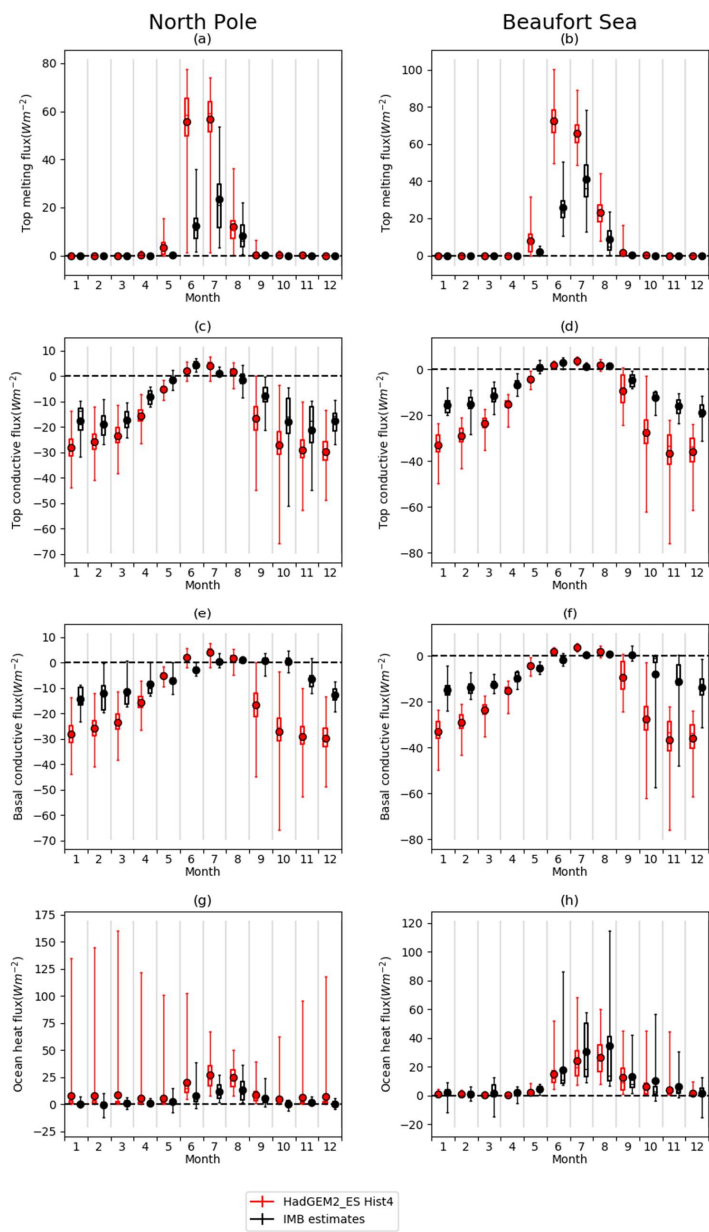
Figure 9. Comparing distributions of (a,b) top melt, (c,d) top conductive flux, (e,f) basal conductive flux and (g,h) ocean heat flux from HadGEM2-ES (red) to those estimated from the IMB data (black), for the North Pole (left) and Beaufort Sea (right) regions.
