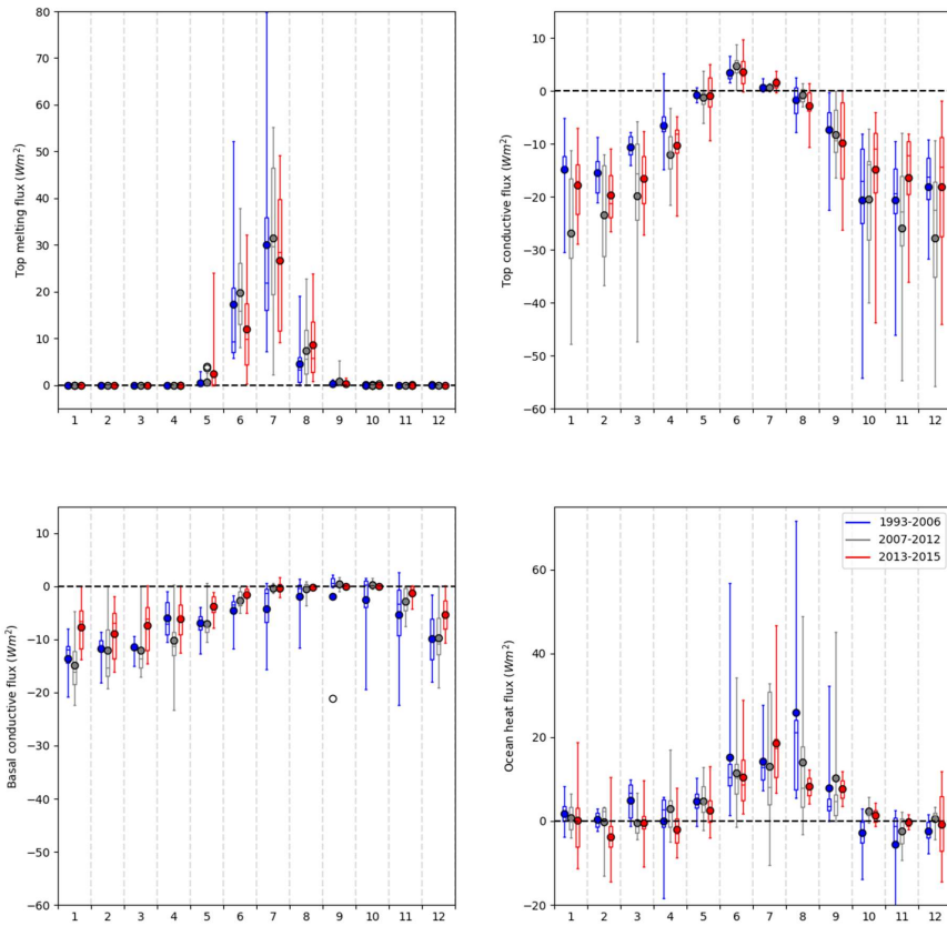
Figure 8. IMB-measured distributions of (a) top melting; (b) top conductive flux; (c) basal conductive flux and (d) ocean heat flux, divided into the three periods 1993-2006, 2007-2012 and 2013-2015. Each distribution is illustrated with a boxplot showing range, interquartile range, median (horizontal lines) and mean (filled circles).
