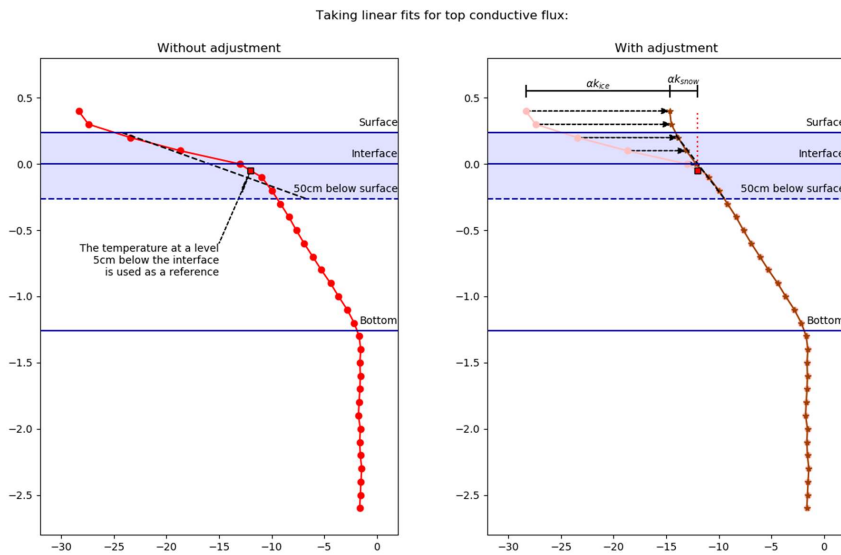
Figure 6. Illustrating the process of estimating conductive flux across the top 50cm of the snow-ice column, in the case that the snow-ice interface lies within this layer. The left panel shows the raw temperature profile: taking a linear fit through these points does not produce a meaningful result because of the sharp ‘corner’ associated with the change in medium. The right panel shows the adjusted temperature profile: the temperatures that would be expected if the snow layer were ice, temperature below the interface and conductive fluxes remaining the same. The adjusted profile eliminates the corner, and a linear fit can be taken. In the right panel, k_{ice} denotes ice conductivity, k_{snow} snow conductivity, and \alpha an arbitrary constant of proportionality.
