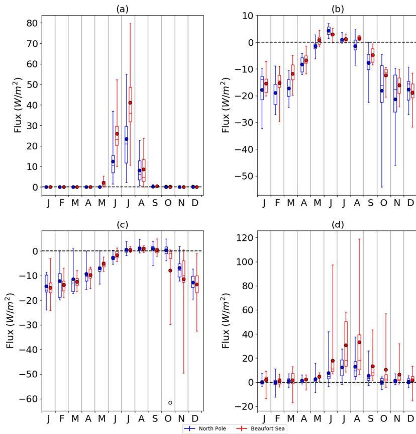
Figure 7. Fluxes of (a) top melting, (b) top conductive flux, (c) basal conductive flux and (d) ocean heat flux, estimated from the IMB data, shown for North Pole (blue) and Beaufort Sea (red) regions. For each month, flux and region, the distribution is indicated by a boxplot showing range, interquartile range, median (horizontal lines) and mean (filled circles). For all fluxes, the convention is that downwards=positive.
