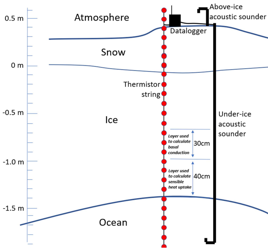
Figure 2. Diagram of the main components of an IMB, with layers used in this study for calculation of fluxes at the base of the ice indicated. Adapted from Figure 1a of Planck et al (2019). Adapted from a diagram by the data providers at http://imb-errel-dartmouth.org/imb/ .
