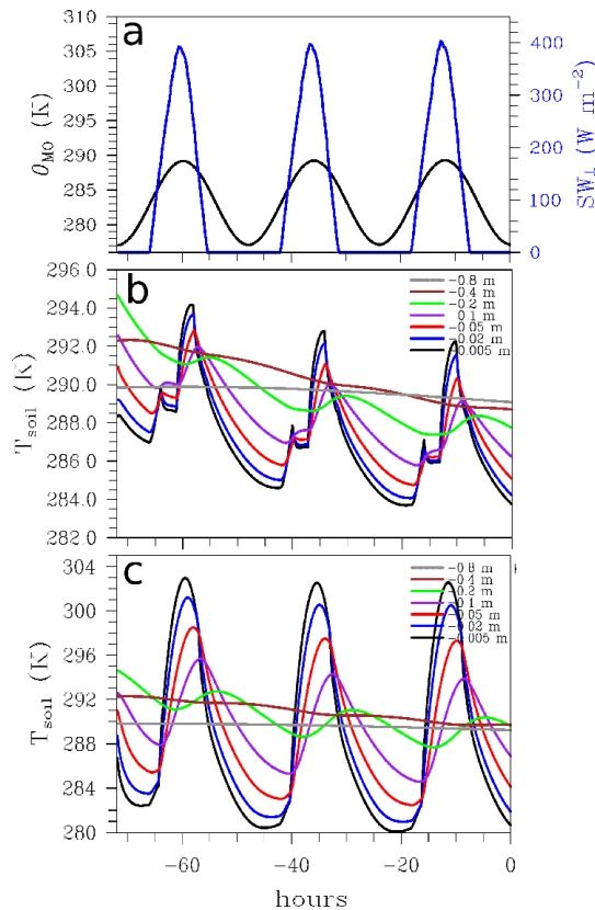
Figure 3. Timeseries during an exemplary surface spin-up of three days (72 h) starting on March 03 for a small LES setup, including different surface types and buildings, geographically located in Hannover, Germany. (a) shows the surface forcing, imposed by an unobstructed incoming solar radiation and the subsequent near-surface potential temperature forcing, while (b) and (c) show the resulting material temperatures T_{\text{soil}} for a soil covered by short grass and an asphalt pavement, respectively. The time axis denote the hours until start of the full 3-D atmospheric simulation. Note that the radiative forcing shown in (a) does not match to the results shown in (b), where shadowing by buildings causes a drop in incoming shortwave radiation during afternoon hours.
