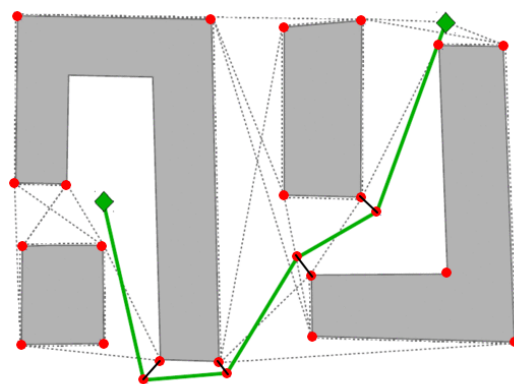
Figure 5. Final result of the pathfinding algorithm using the visibility graph created by the preprocessing tool APT-P. The dots at the obstacle corners mark the nodes of the graph and connections between these nodes, annotated with a cost to travel, are indicated by dashed lines. The left/right rhombus visualises the starting/end point of the path to go, which is illustrated by green lines that are connected at the shifted navigation points. The outward shift of the original nodes toward the actual navigation points is visualised by black lines.
