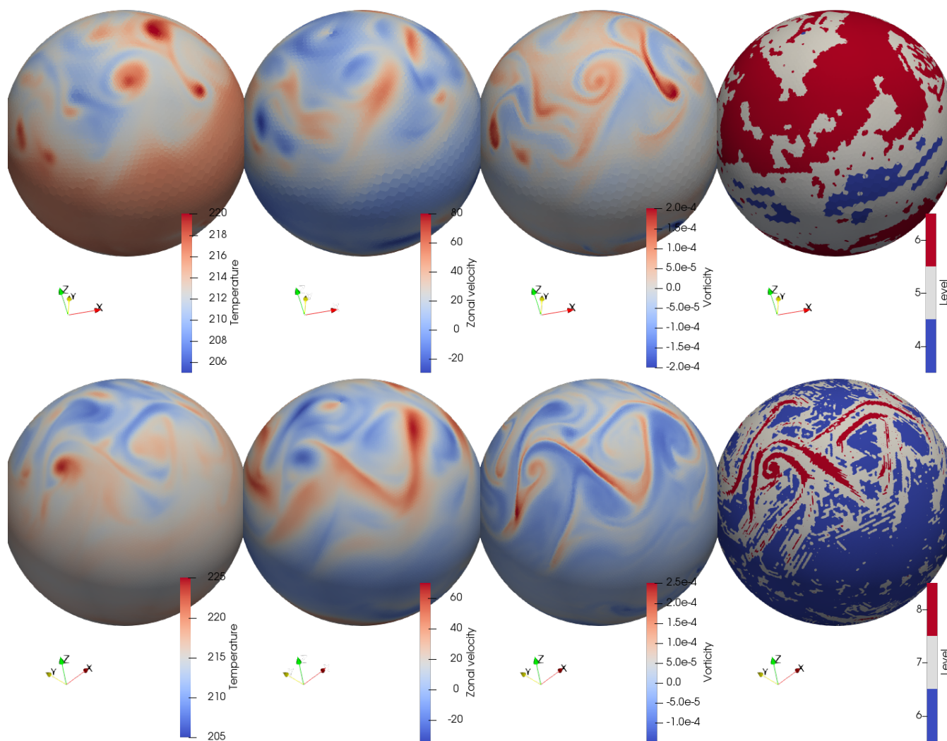
Figure 12. Typical results for the low resolution (top) and high resolution (bottom) Held and Suarez general circulation test case at 250 hPa. The grid is adapted on the solution with relative error tolerance \varepsilon = 0.04 in the low resolution case and \varepsilon = 0.02 in the high resolution case. The grid compression ratio is 2.0 for the low resolution case and 7.5 for the high resolution case.
