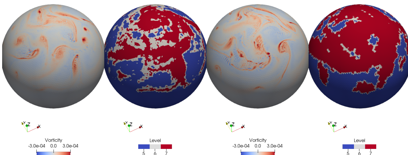
Figure 10. Comparison at days 9 and 20 of the grid compression ratios for the baroclinic instability when adapting on the trend or adapting on the solution. The relative error threshold was set to \varepsilon = 0.03 (fixed) when adapting on the solution and \varepsilon = 0.6 when adapting on the trend. In both cases the resolution is j = 5, 6, 7 and there is no additional diffusion. The tolerances were set to achieve similar compression ratios at 9 days. The vorticity field is shown at hybrid vertical level 4 (about 870 hPa).
