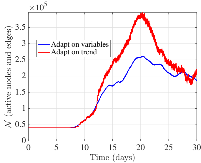
Figure 9. Comparison of the \mathcal{N} for the baroclinic instability when adapting on the trend or adapting on the solution. The relative error threshold was set to \varepsilon = 0.03 when adapting on the solution and \varepsilon = 2 when adapting on the trend. In both cases the active scales are j = 5, 6, 7 and there is no additional diffusion. The tolerances were set to achieve similar compression ratios at 9 days. The total number of available grid points is 8.6 \times 10^5 , and so the minimum grid compression ratio is 3.3 when adapting on the solution and 3.3 when adapting on the trend.
