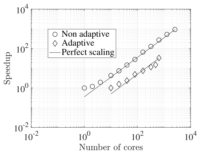
Figure 4. Strong scaling of wavetrisk on the Compute Canada machine niagara for a simulation of the Held and Suarez (1994) general circulation experiment for a perfectly balanced (non-adaptive) run at a resolution of J = 8 ( 1/4^\circ ) and for a strongly unbalanced (dynamically adaptive) run at a maximum resolution of J = 9 ( 1/8^\circ ) resolution with trend based error tolerance \varepsilon = 0.08 .
