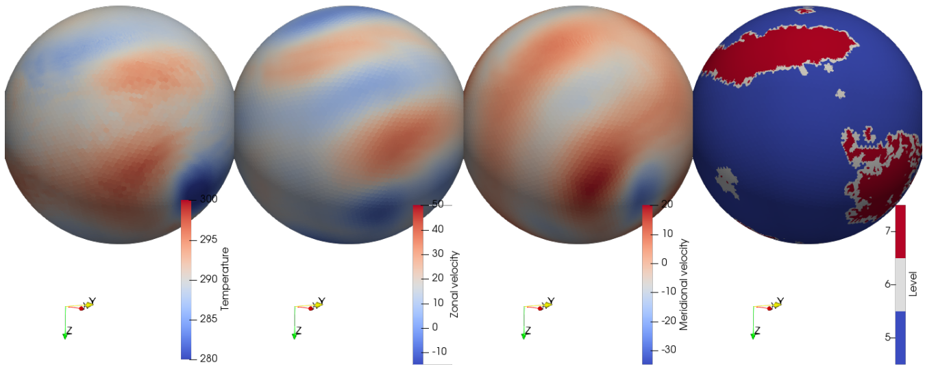
Figure 6. Results of the adaptive simulation of the mountain induced Rossby wave case shown at 700 hPa at day 25.
