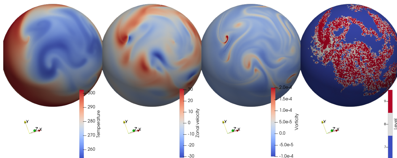
Figure 5. Adaptive Held and Suarez (1994) general circulation experiment at t=500 h with maximum resolution 1/8^\circ used for the strong parallel scaling results shown in figure 4. Results are shown at the vertical level corresponding to 850 hPa. The rightmost figure is the adaptive grid with a grid compression ratio of about 4.5.
